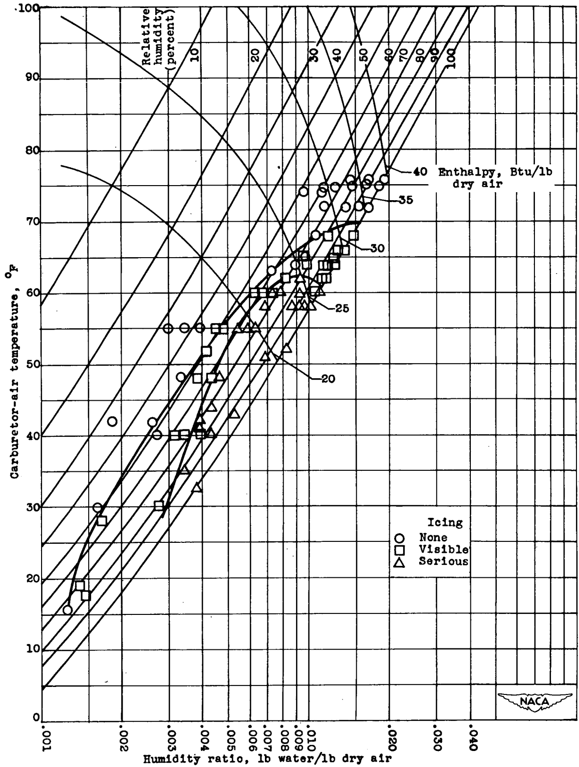
(b) Low-cruise power.
