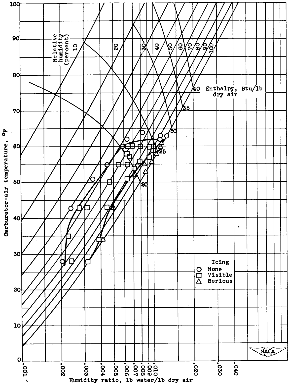
(a) High-cruise power.
