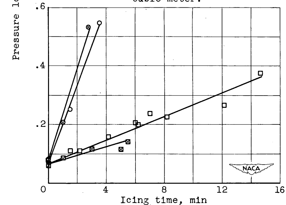
(b) Liquid-water content, 0.9 gram per cubic meter.
