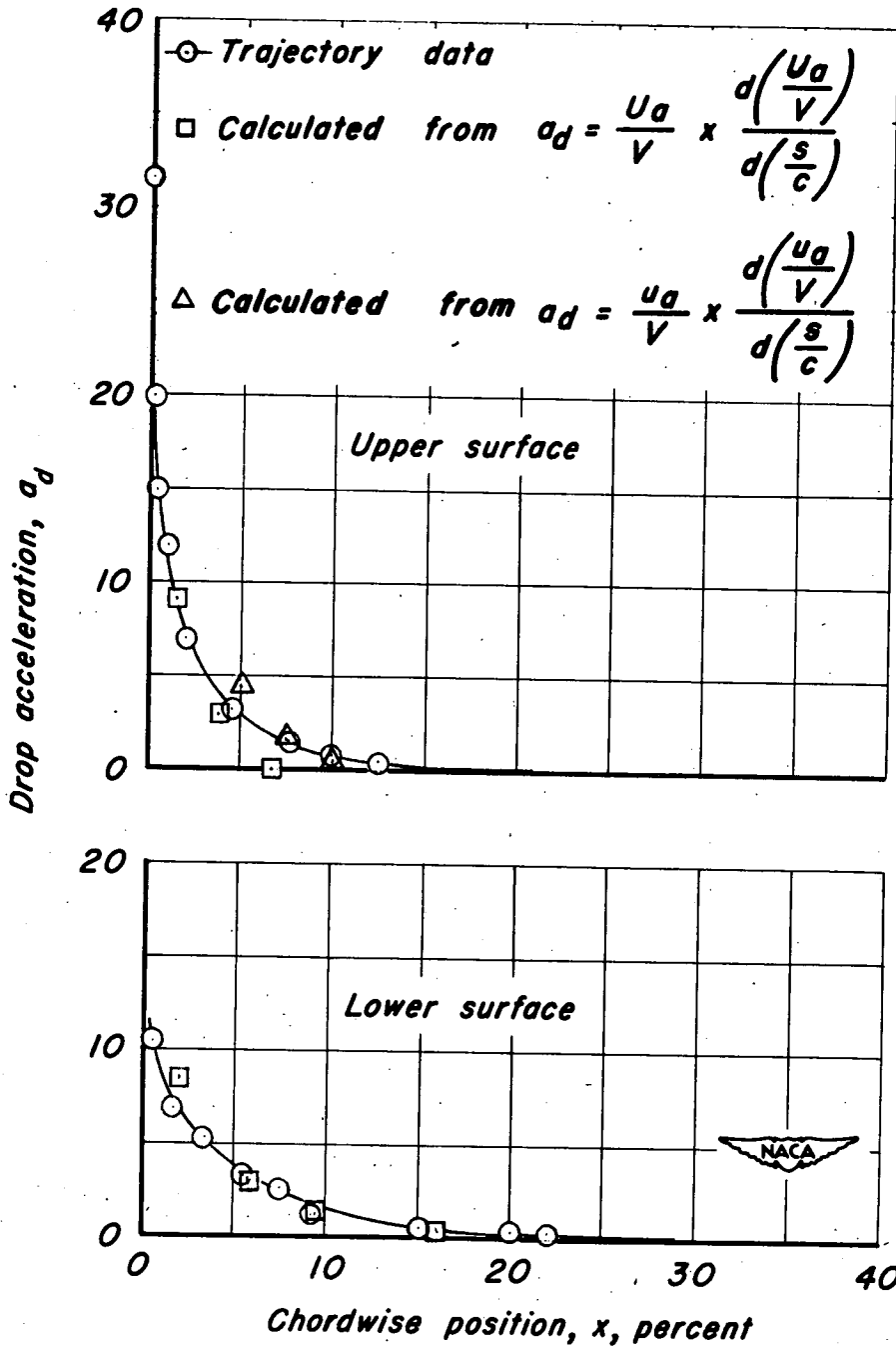
(b) 15-percent-thick symmetrical Joukowski airfoil; \alpha = 2^\circ .
