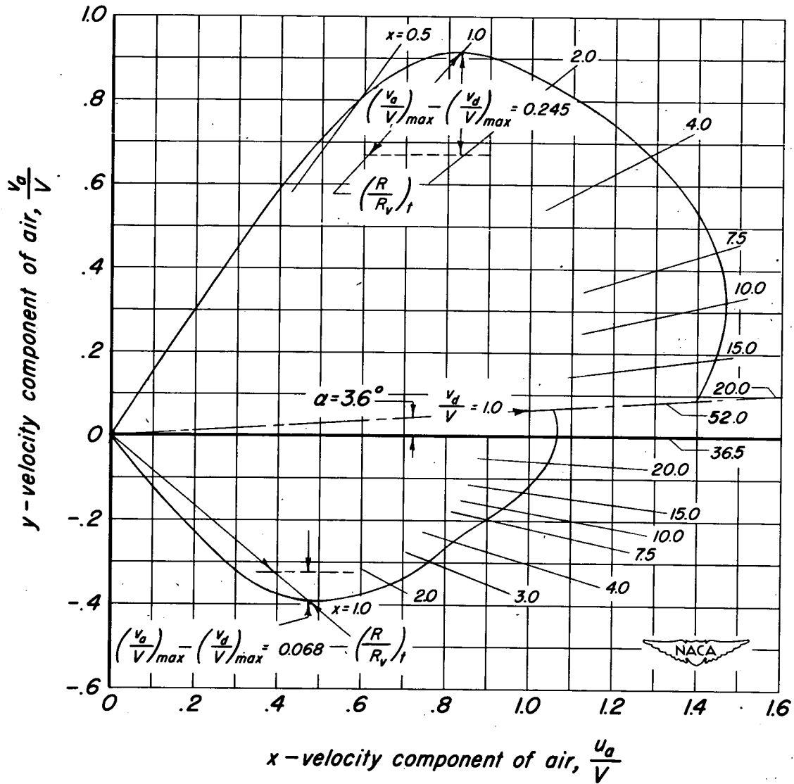
(f) Initial phase of drop hodograph.
