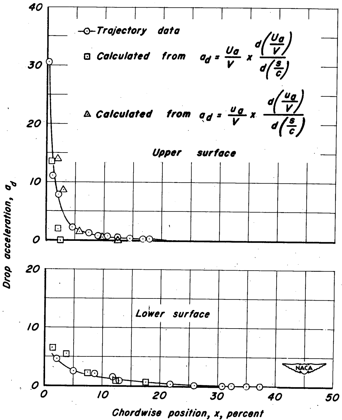
(c) 15-percent-thick symmetrical Joukowski airfoil; \alpha = 4^\circ .
