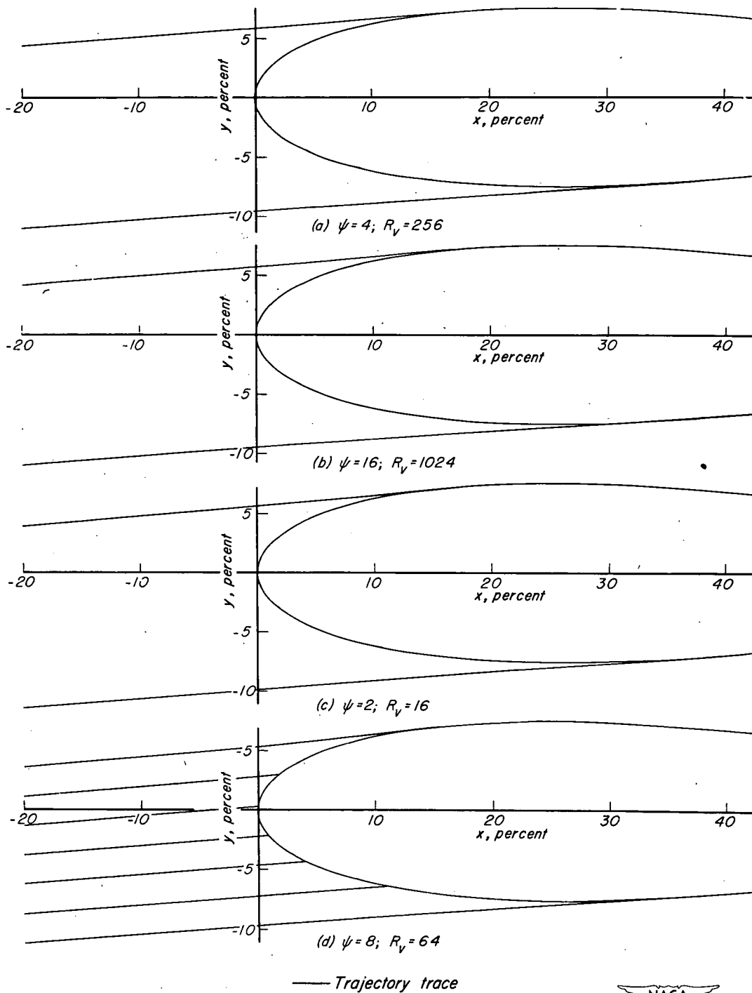
Figure 4.—Water-drop trajectory traces from a differential analyzer for a 15-percent-thick symmetrical Joukowski airfoil; c_l = 0.44 ; \alpha = 4^\circ .
