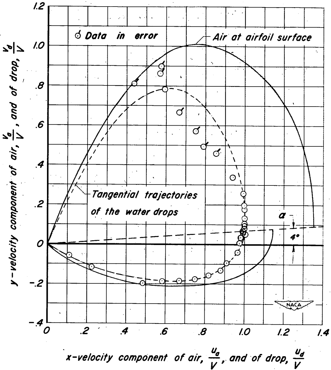
(e) NACA 65 2 -015 airfoil, \alpha = 4^\circ .
