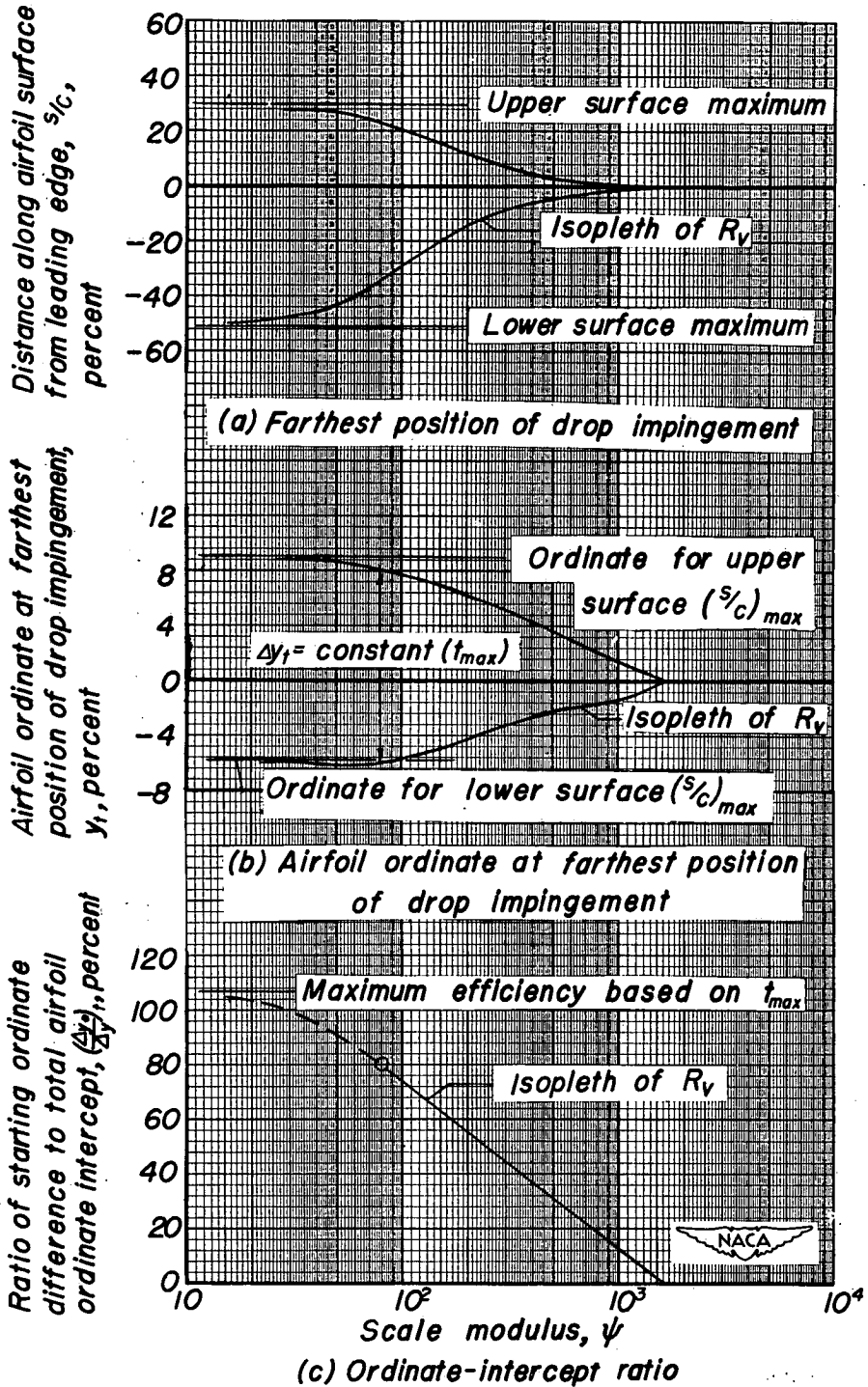
Figure 16.— Graphical representation of the procedure used to obtain a value of \psi corresponding to (\Delta y_s/\Delta y)_t = 0.8
