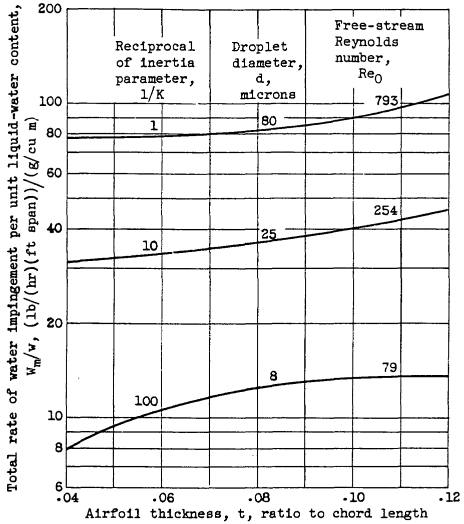
Figure 14. - Rate of water impingement as function of airfoil thickness ratio. Flight speed, 400 miles per hour; airfoil chord length, 12.5 feet; altitude, 10,000 feet; angle of attack, 4°.
