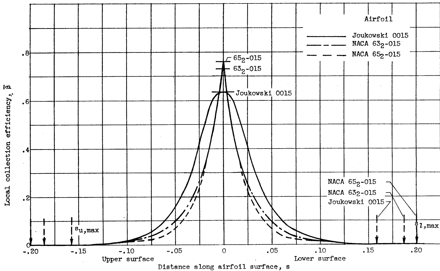
(c) Shape effect. Angle of attack, 0^\circ ; 13-inch chord.
