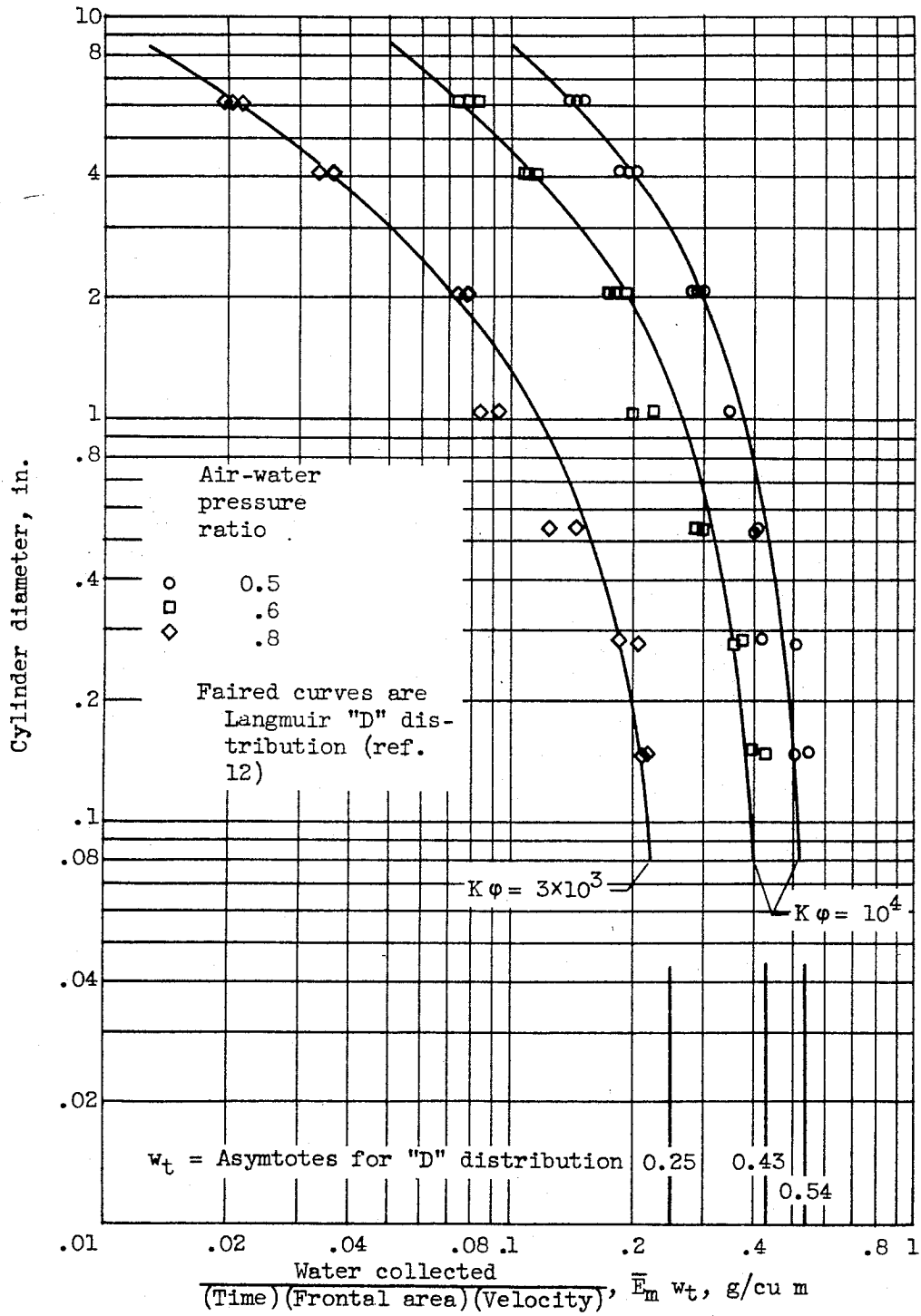
Figure 21. - Water collected by various cylinder sizes. Free-stream velocity, 152 knots; air temperature, 50° F; air pressure, 28.1 inches of mercury.
