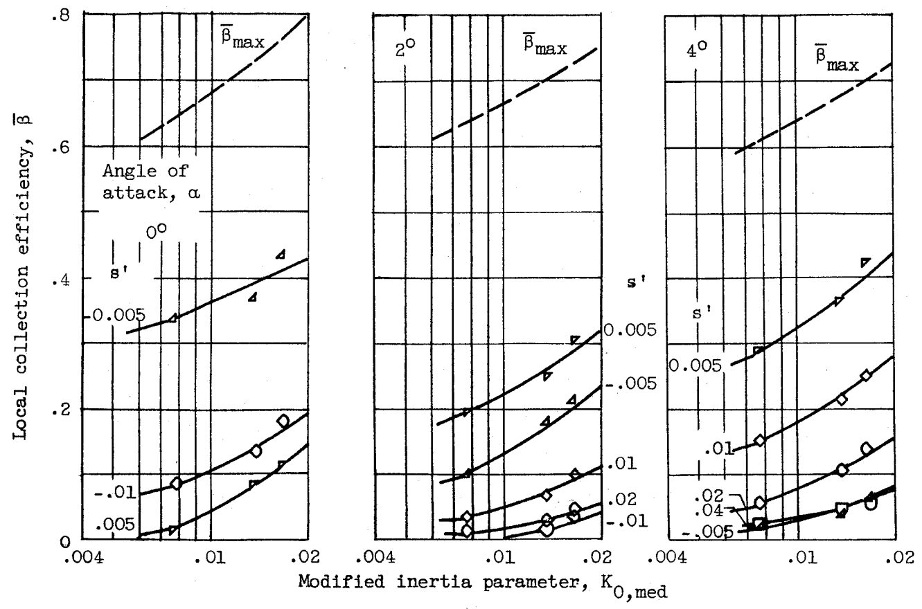
(h) NACA 65 1 -206 airfoil. Chord, 72 inches.
