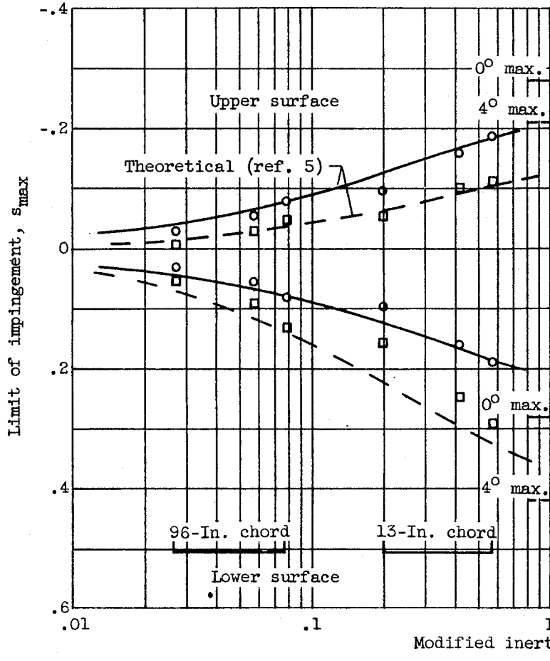
(a) Joukowski 0015 airfoil; angle of attack, 0^\circ and 4^\circ .
