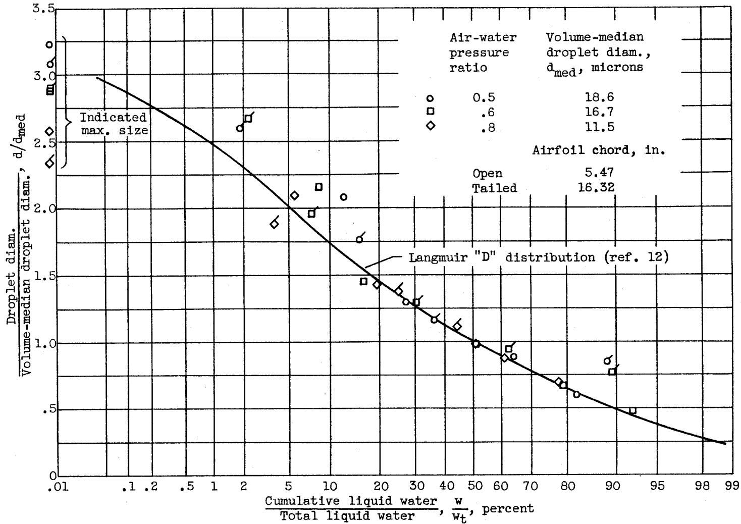
Figure 3. - Dimensionless droplet-size distribution of tunnel spray obtained on 36.5-percent Joukowski airfoil (see appendix B).
