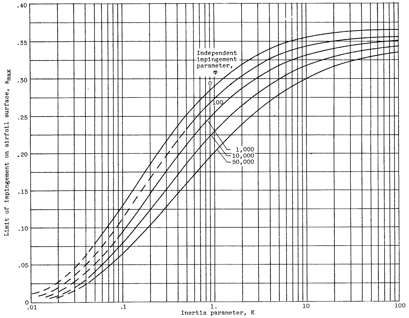
Figure 23. - Limit of impingement on upper or lower surface of 36.5-percent-thick symmetrical Joukowski airfoil. Angle of attack, 0°.
