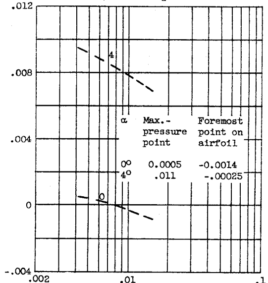
(c) NACA 632-015
