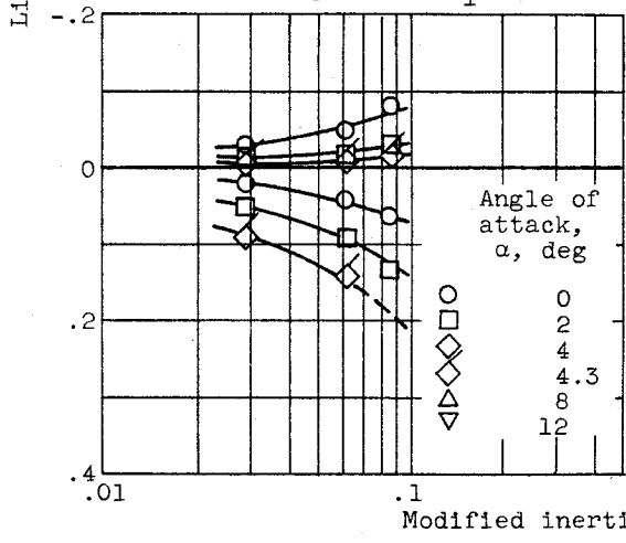
(i) NACA 65 1 -212, 35° sweep. Chord, 87.9 inches.
