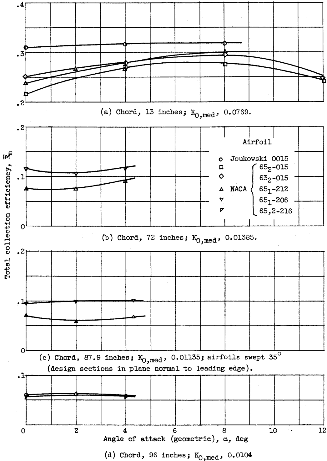
Figure 13. - Effect of angle of attack on experimental total collection efficiency of six airfoil sections. Airspeed, 152 knots; volume-median drop diameter, 16.7 microns.
