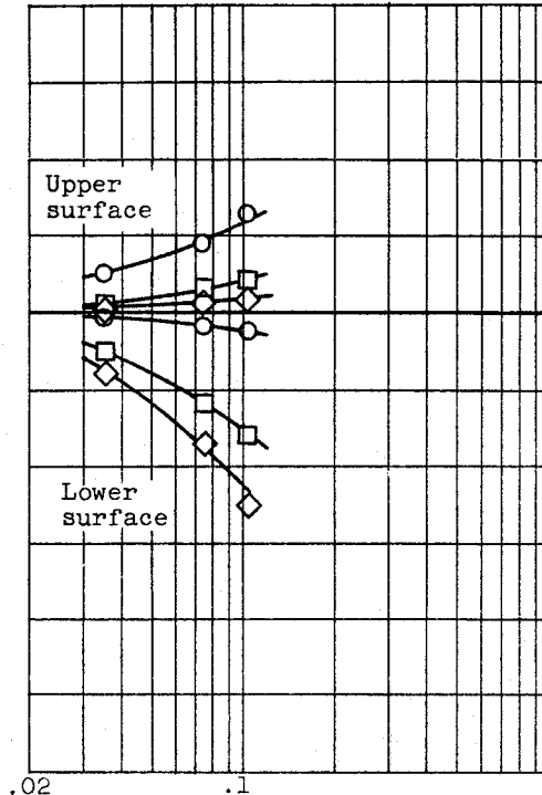
(h) NACA 65 1 -206. Chord, 72 inches.
