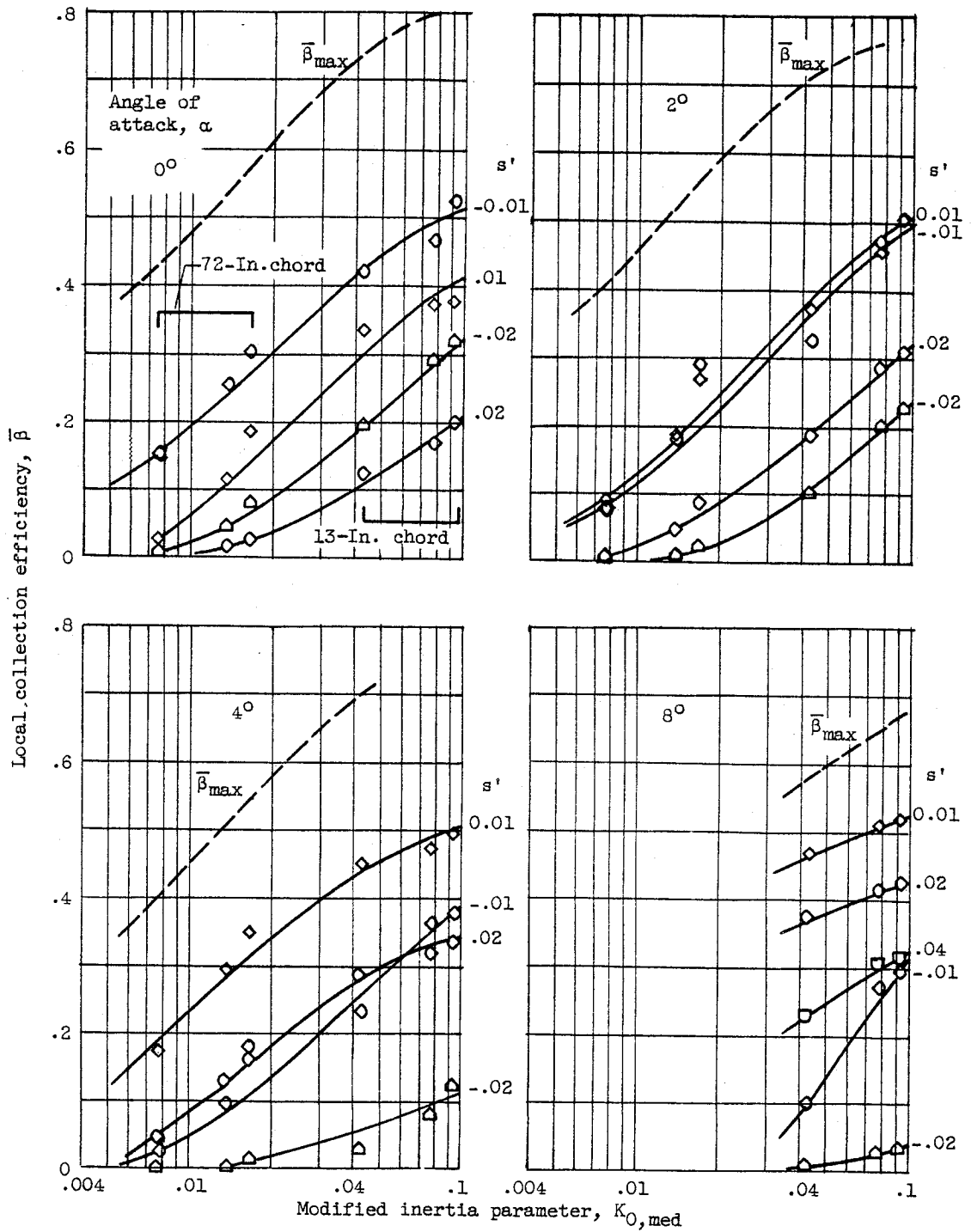
(f) and (g) NACA 65 1 -212 airfoils. Chord, 13 and 72 inches.
