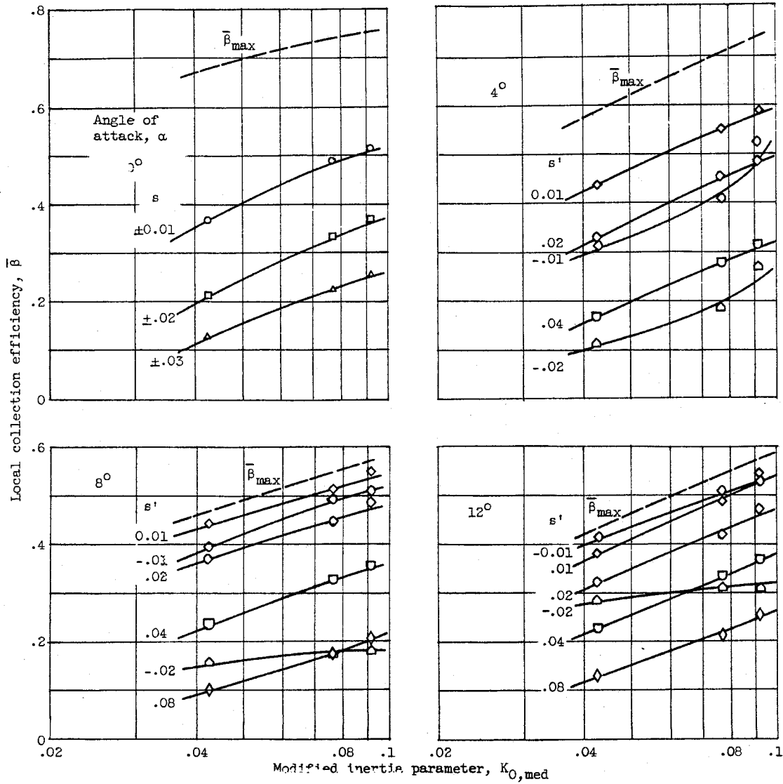
(c) NACA 63 2 -015 airfoil. Chord, 13 inches.
