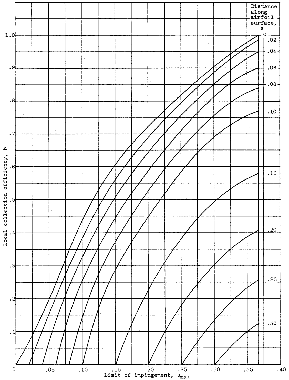
Figure 24. - Local collection efficiency of 36.5-percent-thick symmetrical Joukowski airfoil. Angle of attack, 0^\circ .
