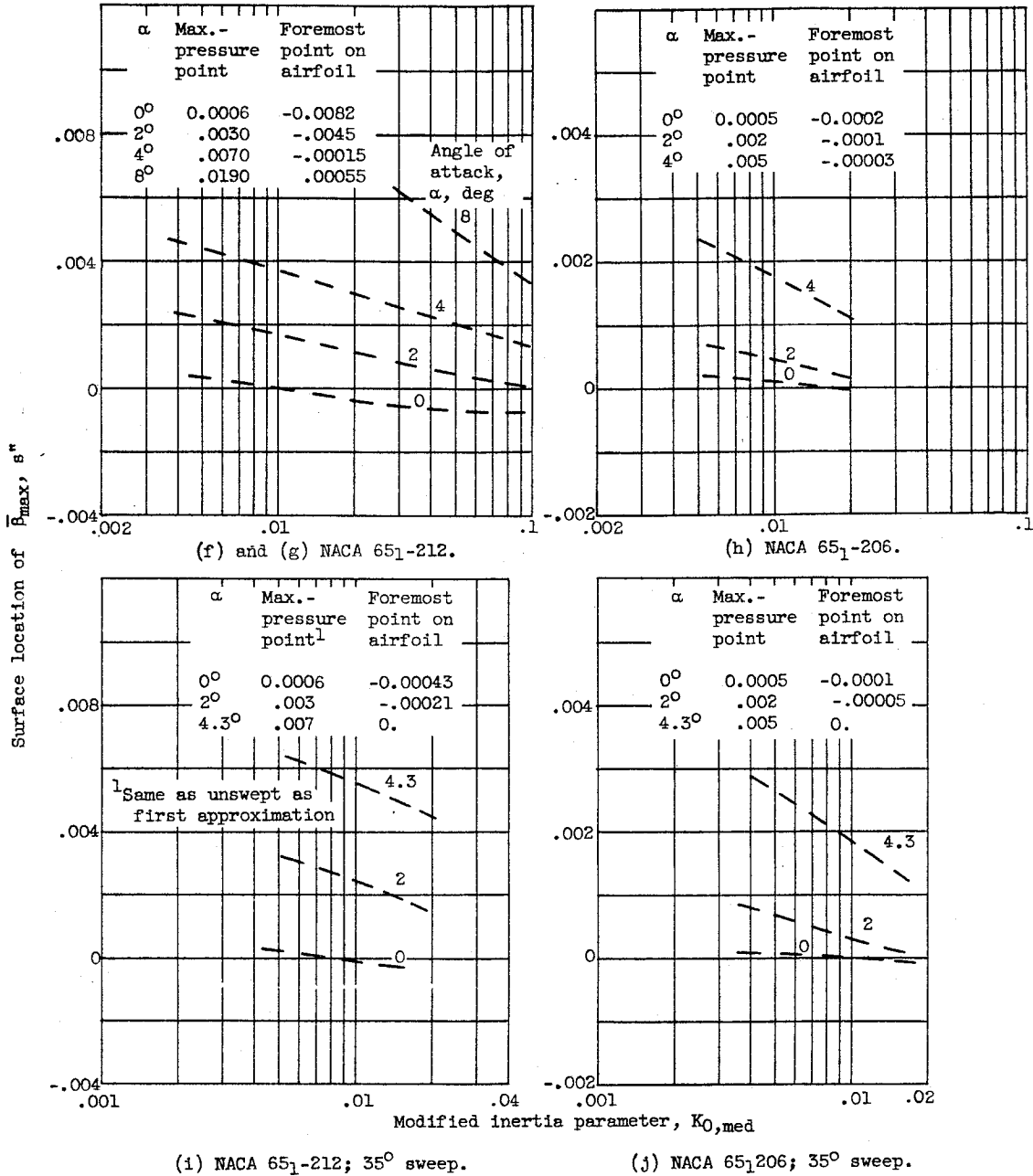
Figure 10. - Concluded. Surface location of maximum local collection efficiency as function of modified inertia parameter (max. and foremost points tabulated as s^* distance).
