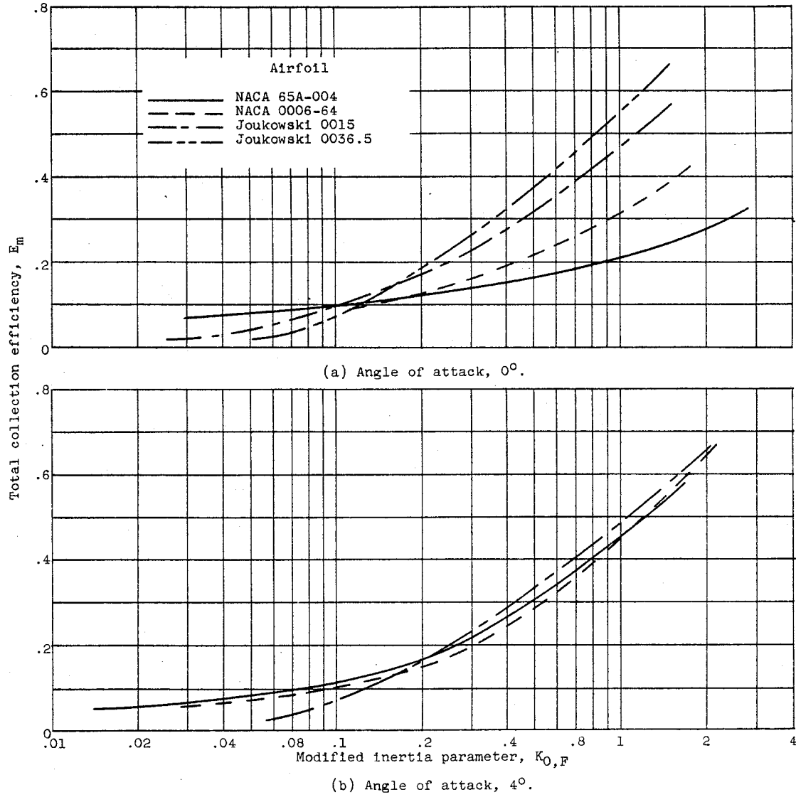
Figure 20. - Correlation of total collection efficiency with inertia parameter modified by projected height.
