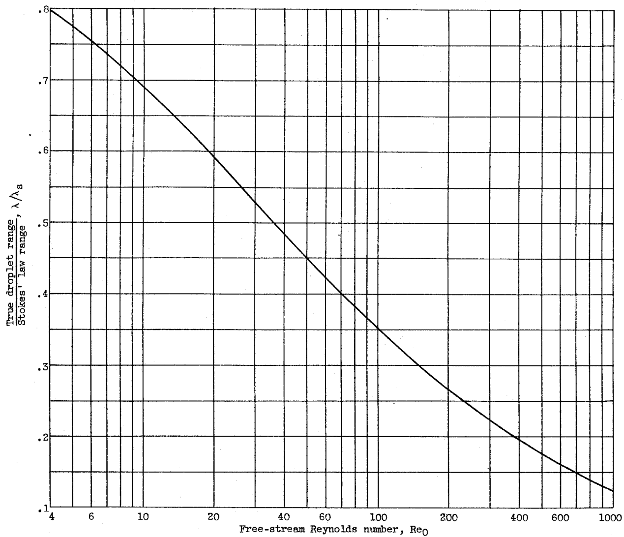
Figure 6. - Droplet range ratio as function of droplet Reynolds number (data from ref. 12).
