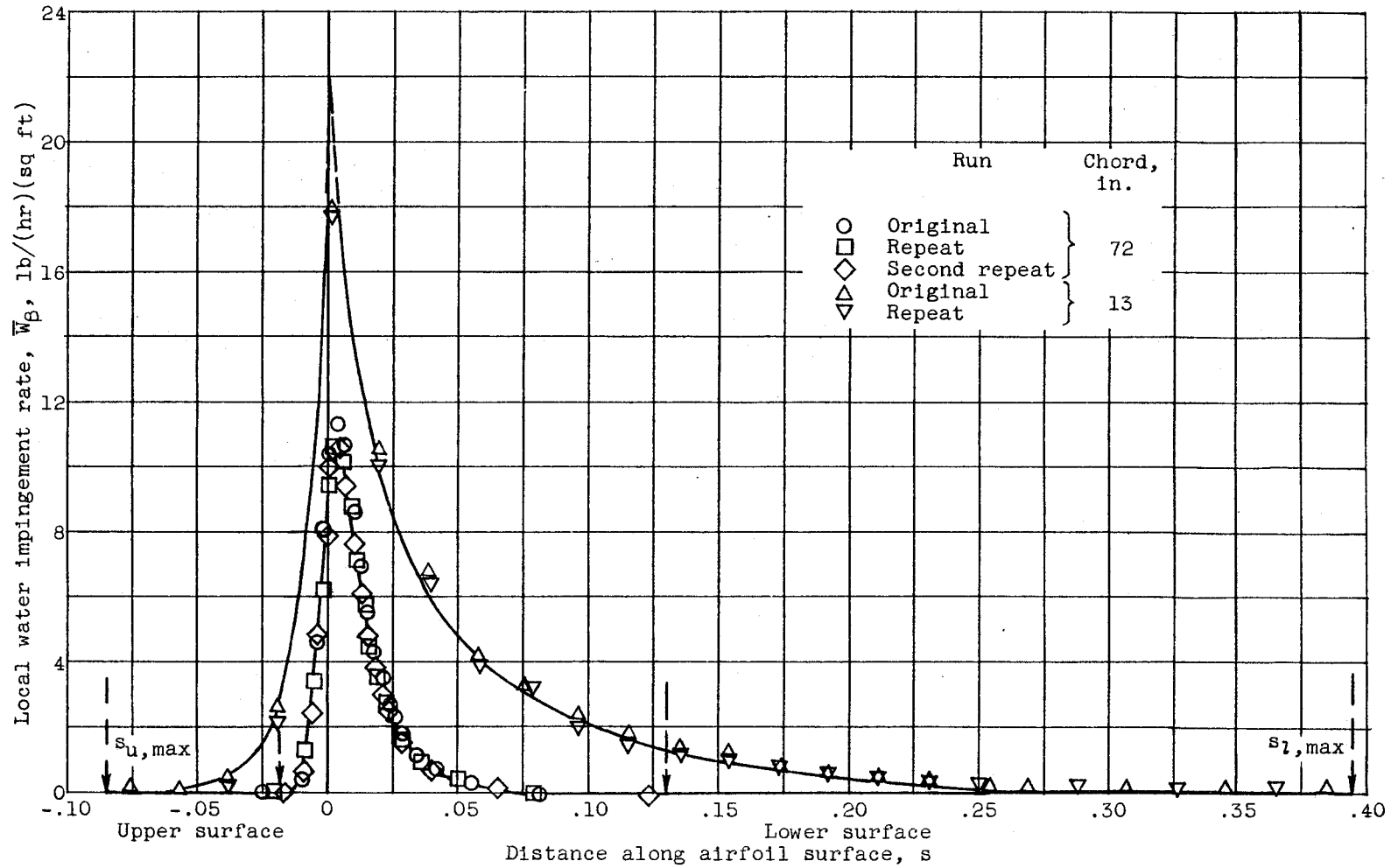
Figure 7. - Typical water impingement rates on NACA 65 1 -212 airfoil. Airspeed, 152 knots; volume-median droplet diameter, 16.7 microns; angle of attack, 4°.
