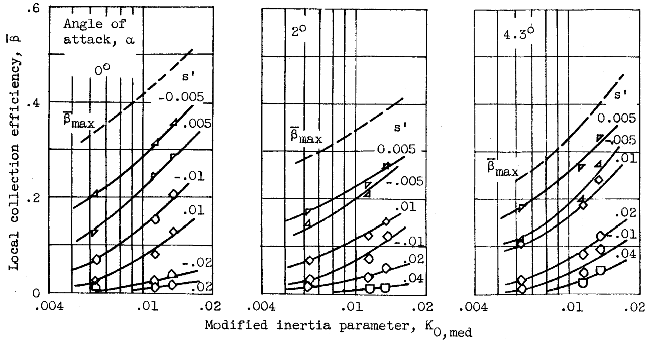
(i) NACA 65 1 -212 airfoil, swept 35° (data in free-stream direction). Chord, 87.9 inches.
