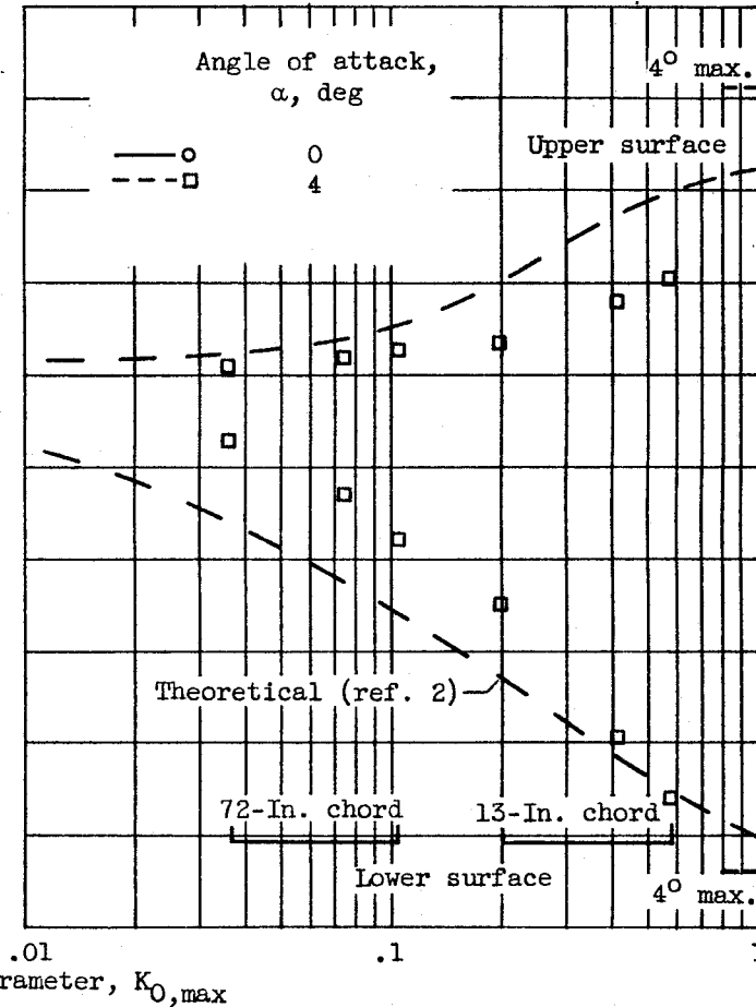
(b) NACA 65 1 -212 airfoil; angle of attack, 4^\circ .
