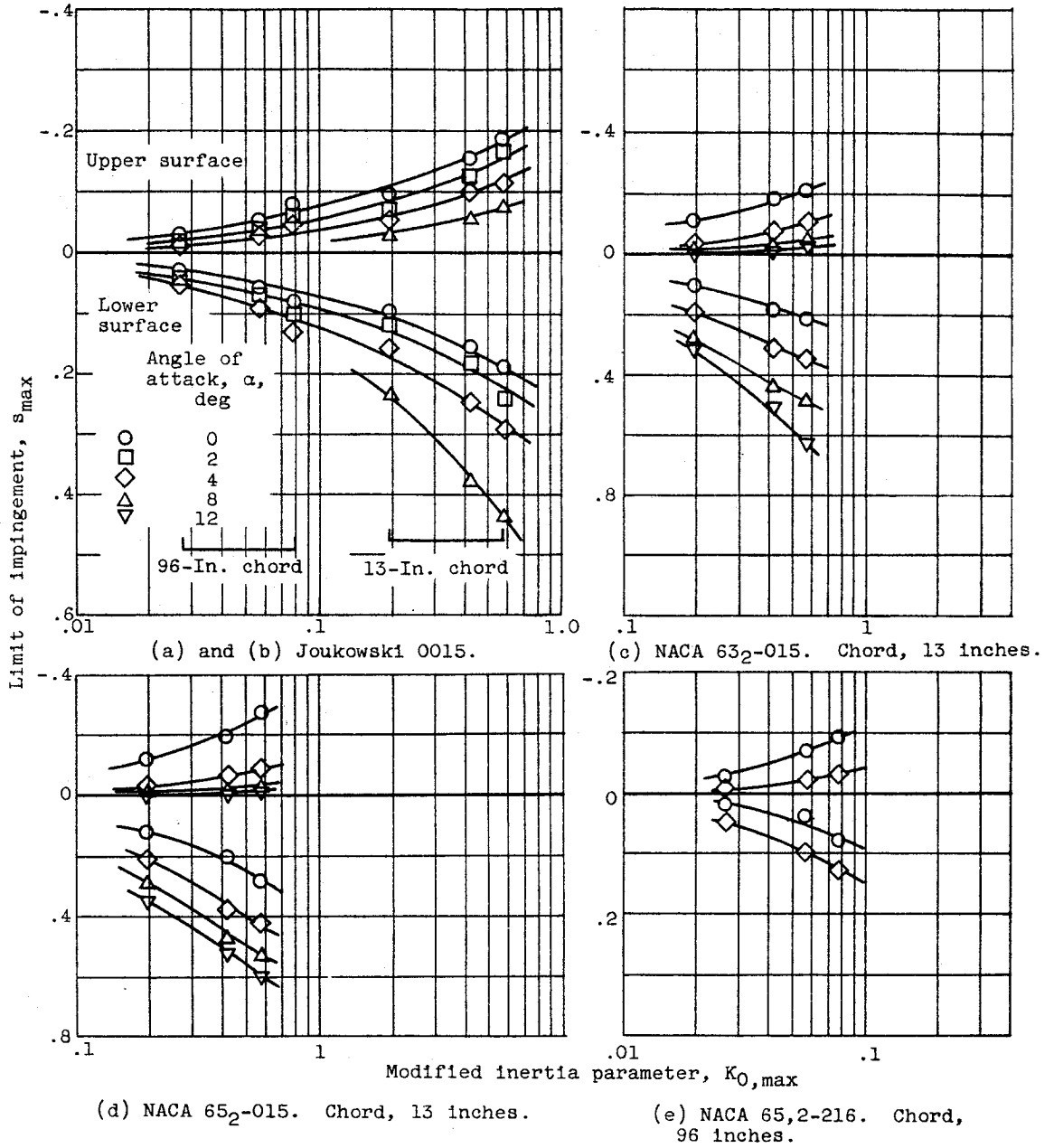
Figure 11. - Limits of impingement on airfoils as function of modified inertia parameter.
