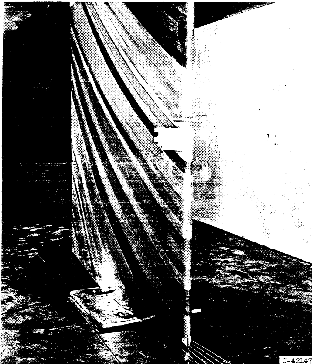
Figure 1. - Typical installation of airfoil (NACA 65 1 -212) with blotter attached, in 6- by 9-foot test section of icing tunnel.
