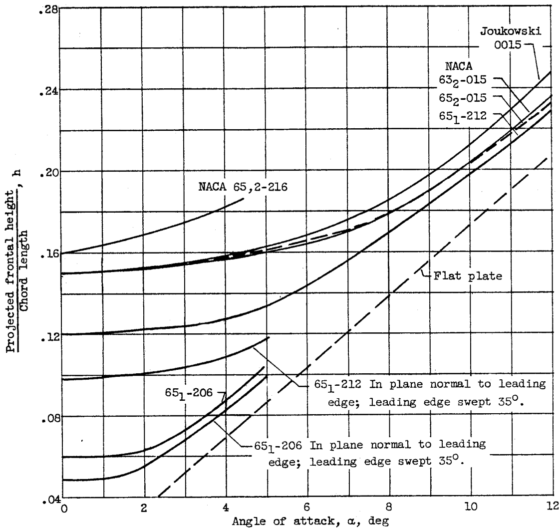
Figure 5. - Effect of angle of attack on ratio of projected height to chord length of various airfoils. (Reference is free-stream-velocity direction.)
