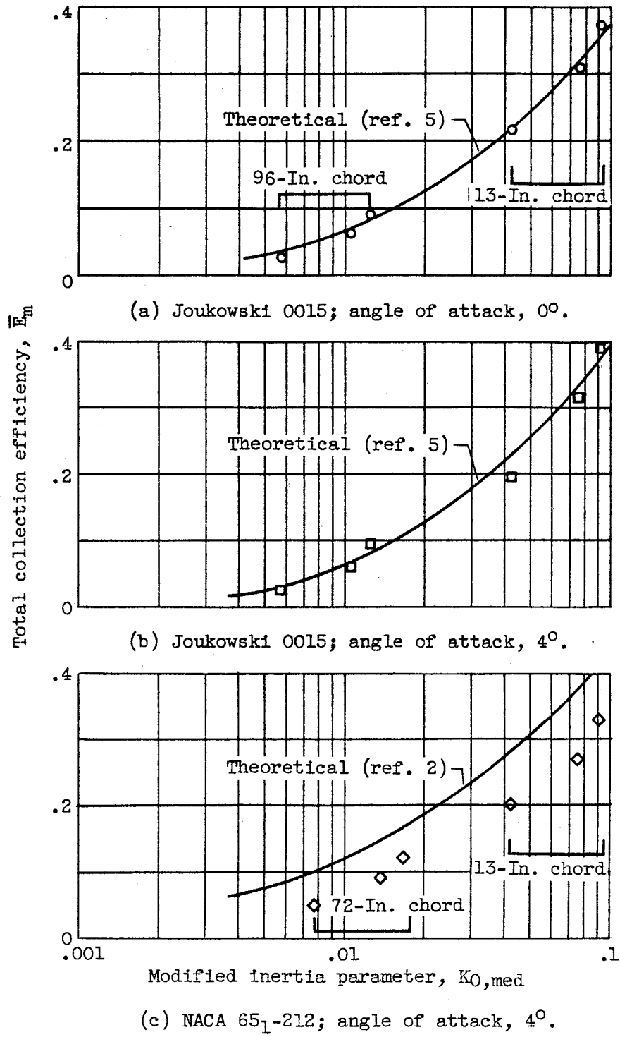
Figure 17. - Comparison of experimental and theoretical total collection efficiencies.
