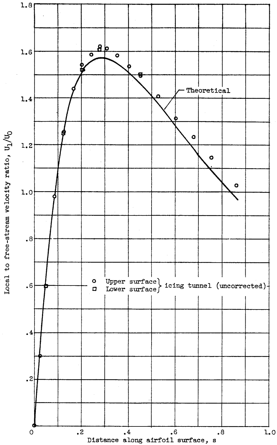
Figure 22. - Local velocity distribution on 36.5-percent-thick symmetrical Joukowski airfoil. Angle of attack, 0^\circ ; chord, 16.32 inches; airspeed, 152 knots; pressure, 28.1 inches of mercury; temperature, 50^\circ F.
