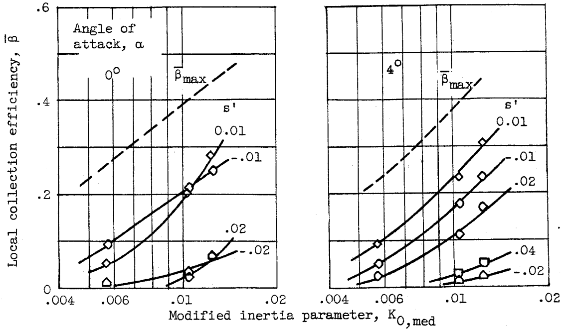
(e) NACA 65,2-216 airfoil. Chord, 96 inches.
