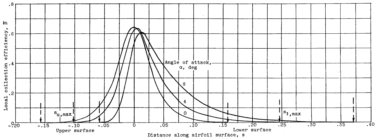
(a) Angle of attack effect. Joukowski 0015 airfoil; 13-inch chord.
