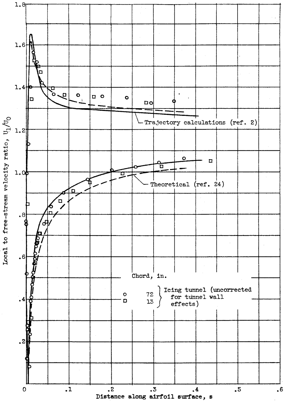
(b) NACA 65 1 -212 airfoil; angle of attack, 4°.
