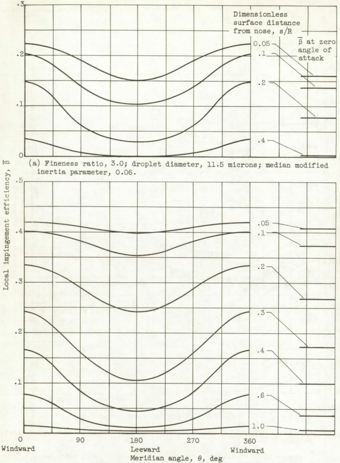
(b) Fineness ratio, 3.0; droplet diameter, 18.6 microns; median modified inertia parameter, 0.12.
