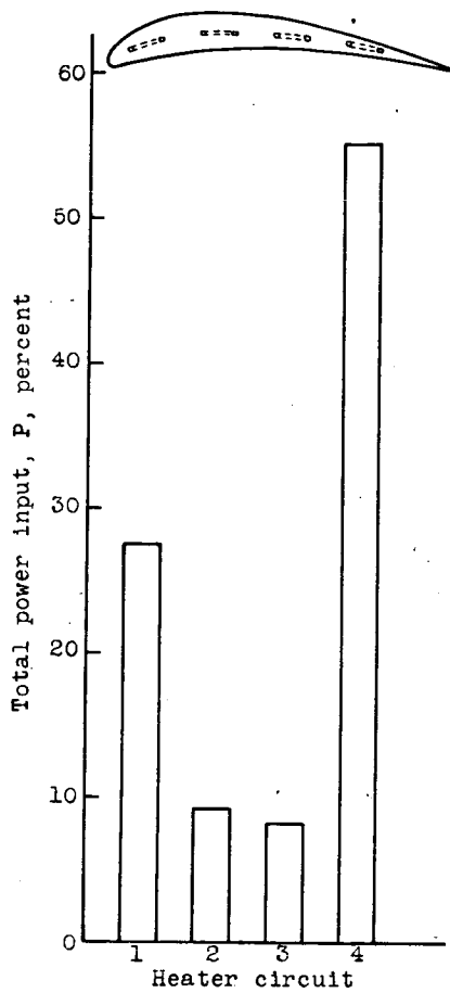
Figure 11. - Minimum average total power per heater for icing protection with continuous heating.
