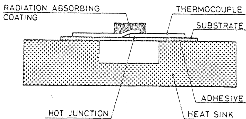
FIG.11-THIN FILM THERMOPILE
