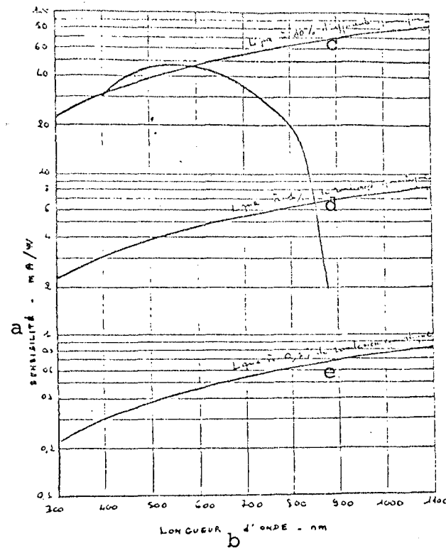
Figure 4 Typical Spectral Response of an S20R Photocathode
