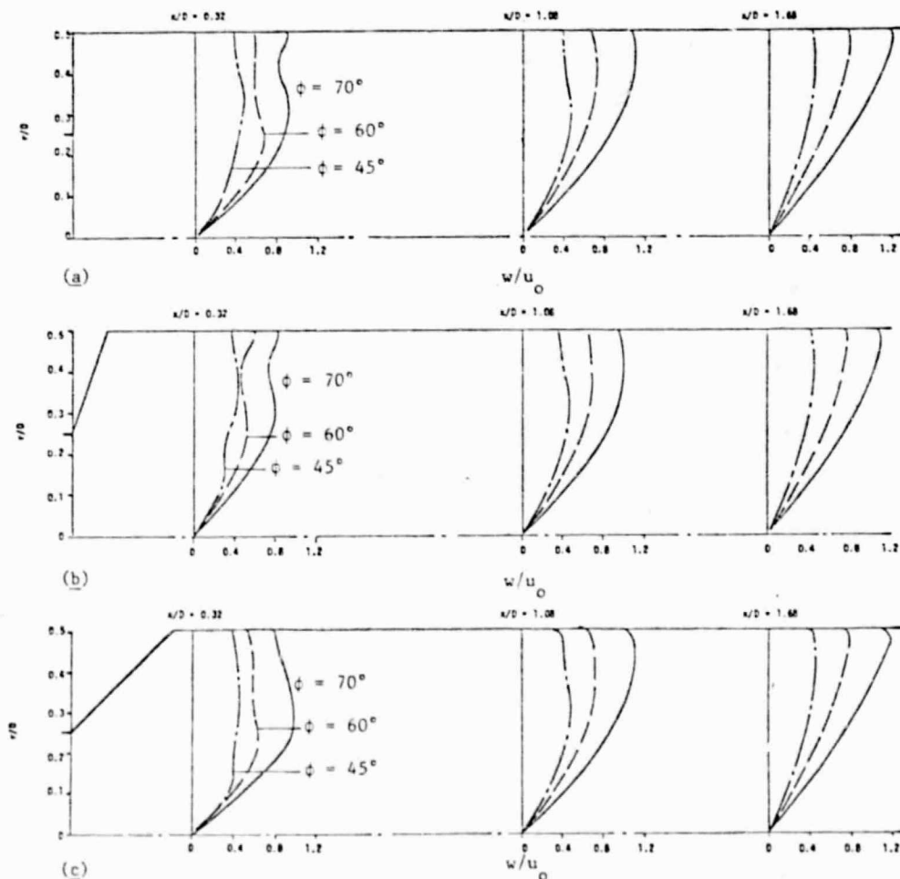
Fig. 6. Predicted swirl velocity profiles for Re_d = 1.26 \times 10^5 showing the effect of swirl vane angle \phi for wall expansion angles \alpha : (a) 90^\circ , (b) 70^\circ , and (c) 45^\circ
