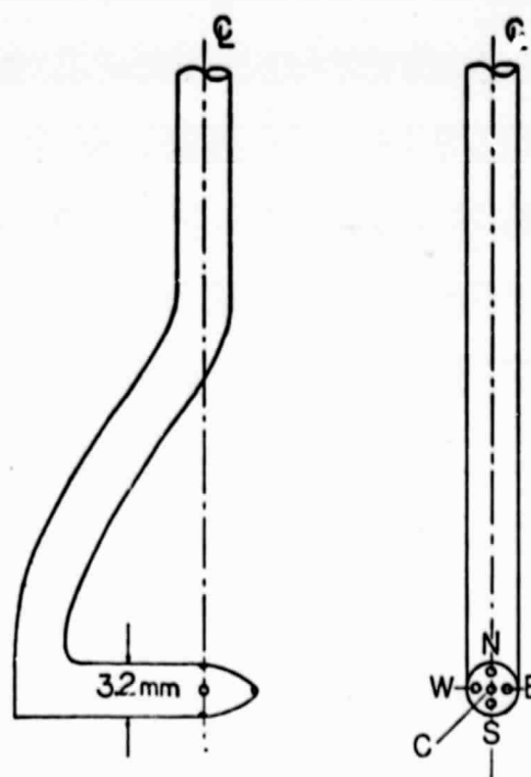
Fig. 3 Five-hole pitot probe.
