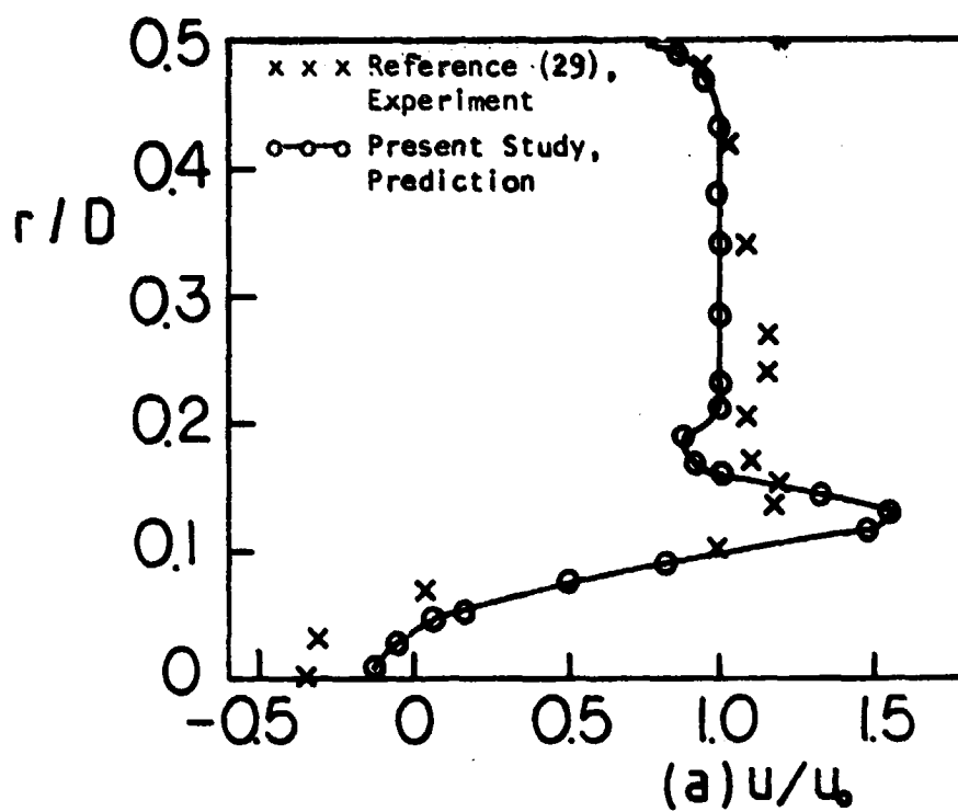
Figure 54. Velocity Profiles at x/D = 0.274 ( x = 4 cm) for the Counterswirling Coannular Pipe Flow Test Case (a) Axial Velocity and (b) Swirl Velocity
