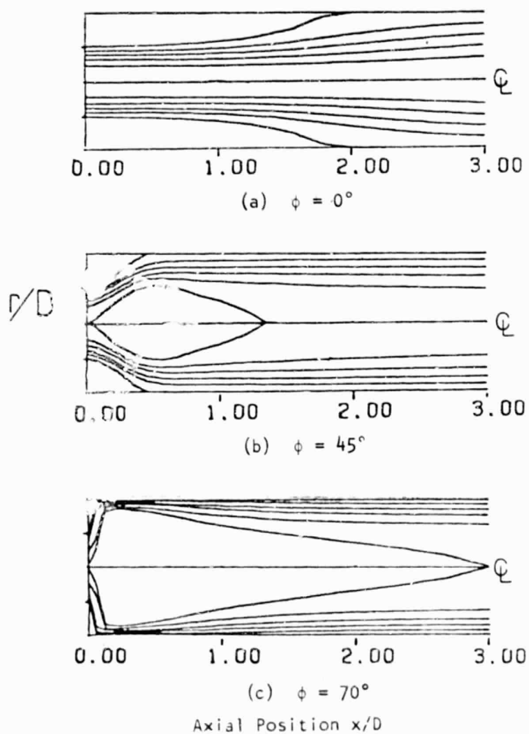
Figure 30. Predicted Streamline Plots With Wall Expansion Angle \alpha = 90^\circ for Swirl Vane Angles: (a) \phi = 0^\circ , (b) \phi = 45^\circ , and (c) \phi = 70^\circ
