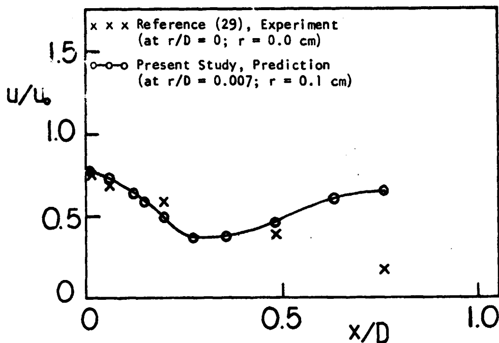
Figure 59. Centerline Axial Velocity Development for the Coswirling Coannular Pipe Flow Test Case
