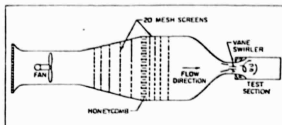
Fig. 2 Schematic of flow facility.
