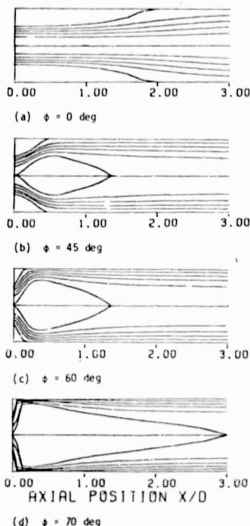
Fig. 5. Predicted streamline plots for a wall expansion angle \alpha = 90^\circ for various swirl vane angles \phi , nonreacting flowfield.
