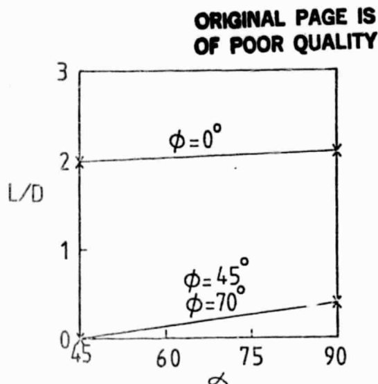
Fig. 10 Experimental effect of wall expansion angle \alpha and swirl vane angle \phi on corner recirculation zone length.
