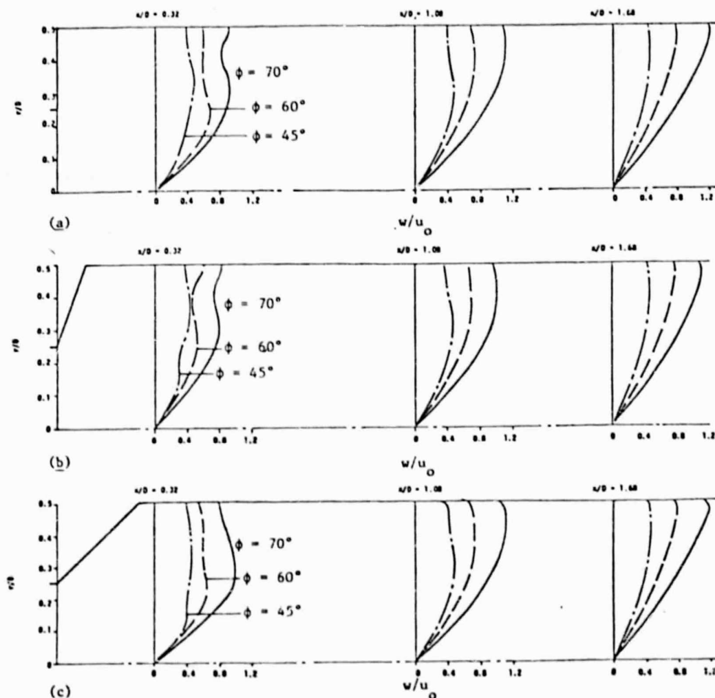
Fig. 8. Predicted swirl velocity profiles showing the effect of swirl vane angle \phi for wall expansion angles \alpha : (a) 90°, (b) 70°, and (c) 45°, nonreacting flowfield.
