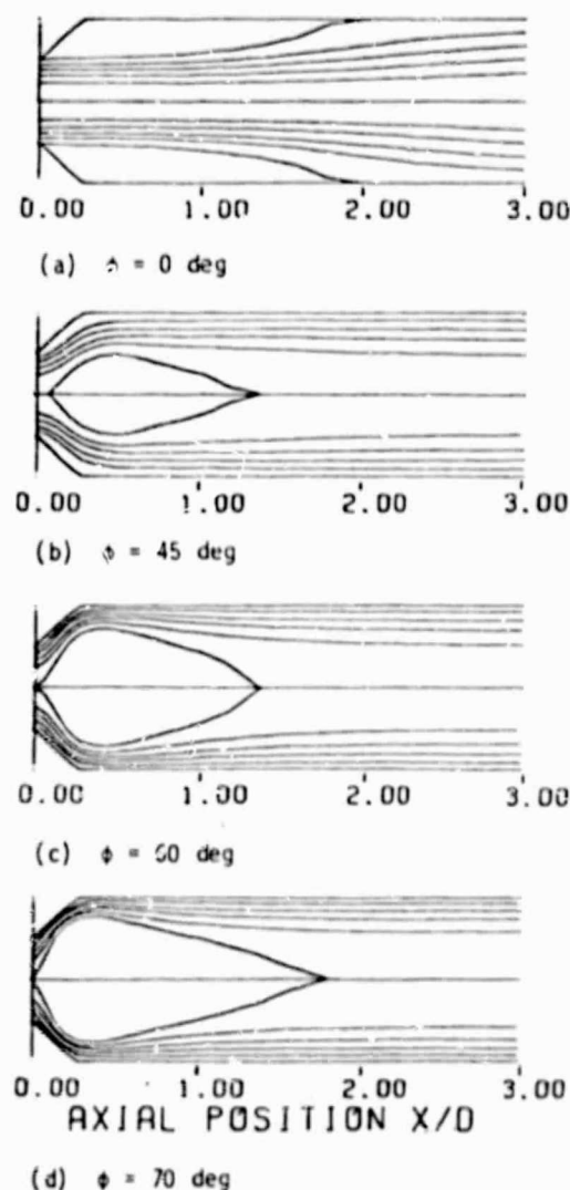
Fig. 6. Predicted streamline plots for a wall expansion angle \alpha = 45^\circ for various swirl vane angles \phi , nonreacting flowfield.
