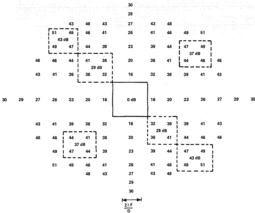
Figure 4.- Crosstalk from square subfacets.
