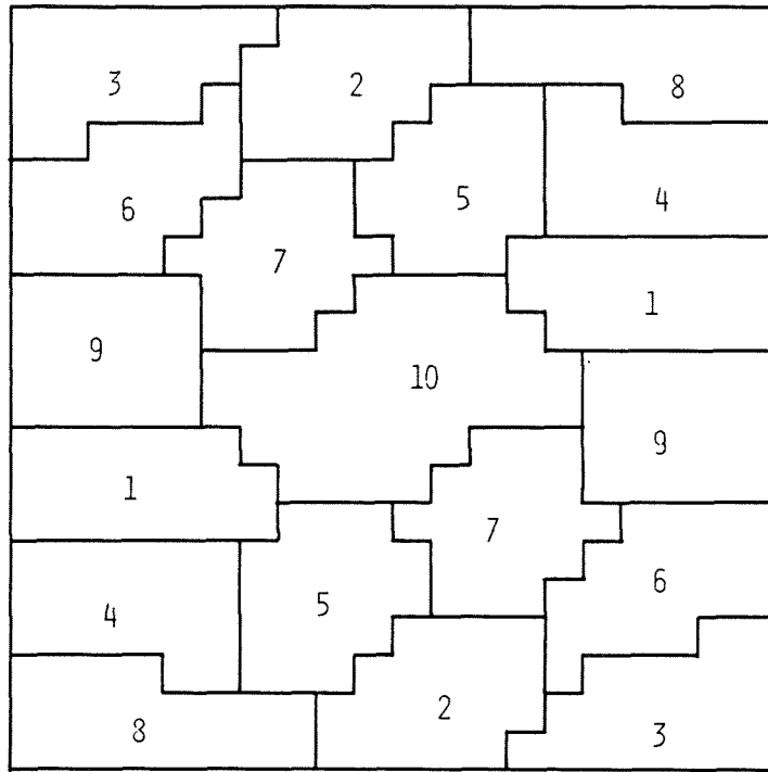
Figure 3.- PCGH design showing facet boundaries. (Fringes within facets not shown.)
