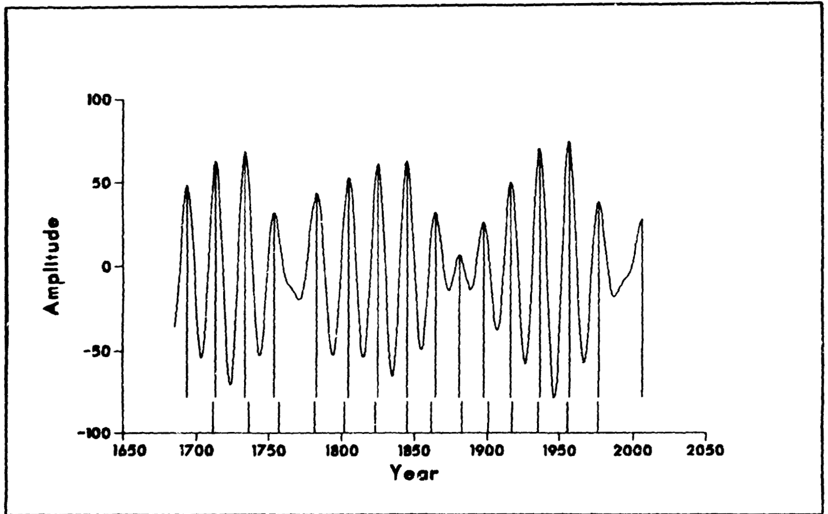
Figure 4. Beat wave between a constant 18.61 year period representing the lunar nodal tide cycle and the 22.279 year corrected Hale magnetic sunspot cycle with amplitude adjusted to fit the recorded sunspot activity. The long vertical lines mark the peaks of the beat wave, the short marks below them mark the times of maximum drought from Mitchell, Stockton and Meko.
