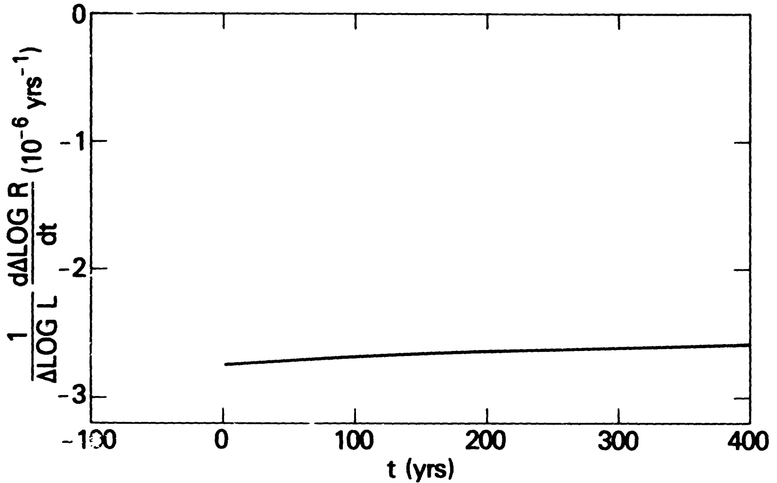
Figure 9. Time dependence of the ratio H = (\Delta \log L)^{-1} \frac{d \Delta \log R}{dt} shortly after the perturbation \Delta \alpha = 0.01 within the solar convective envelope
