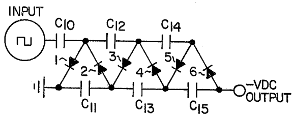
FIG. 4 PRIOR ART
