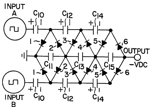
FIG. 5 PRIOR ART OF FIG. 4 BACK TO BACK
