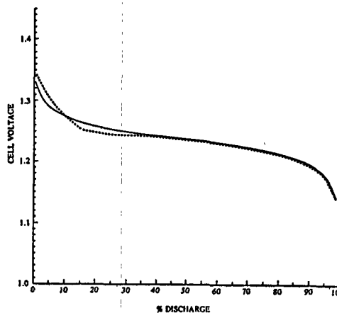
Figure 2. Calculated discharge curve based on the modified thermodynamic model, equation (9). The broken curve is experimental data.
