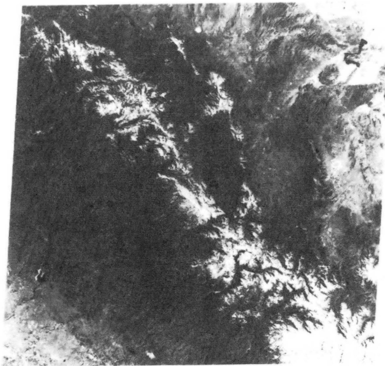
15 APRIL 1977 AVERAGE SNOWLINE ELEVATION = 6700 FT.
