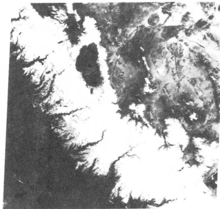
22 APRIL 1978 AVERAGE SNOWLINE ELEVATION = 4900 FT.
