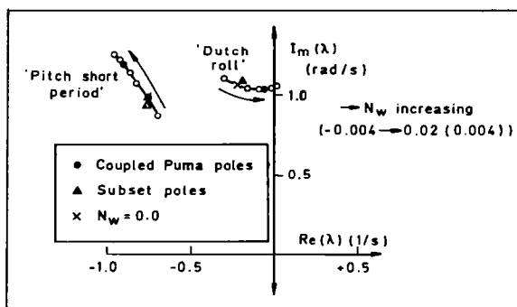
Fig 6 Root loci for fast oscillatory modes with varying yawing moment due to incidence ( N_w )
