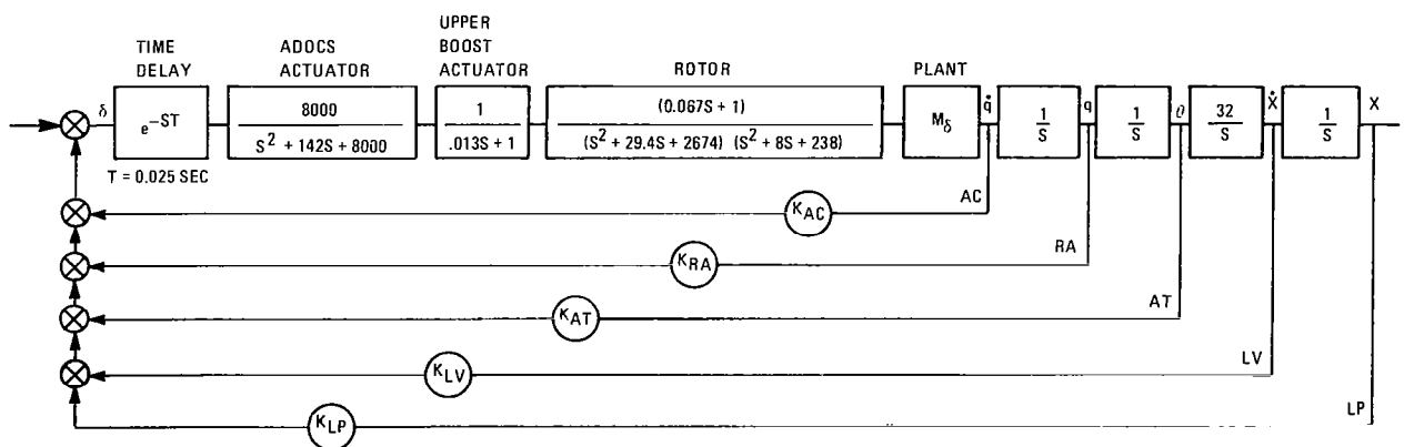
Figure 8 Helicopter/Stability Augmentation System Model-Longitudinal Axis
