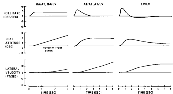
Figure 9 Lateral Response to Step Force Input
