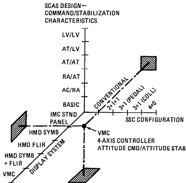
Figure 1 Three-Dimensional Flight Control System Description
