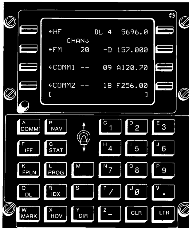
Fig. 3. Control display unit (COMM radio control display).
