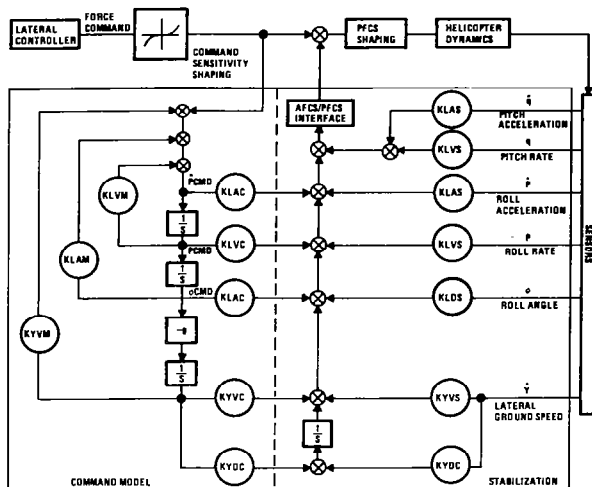
Figure 7 Lateral Axis Stability and Control Augmentation System
