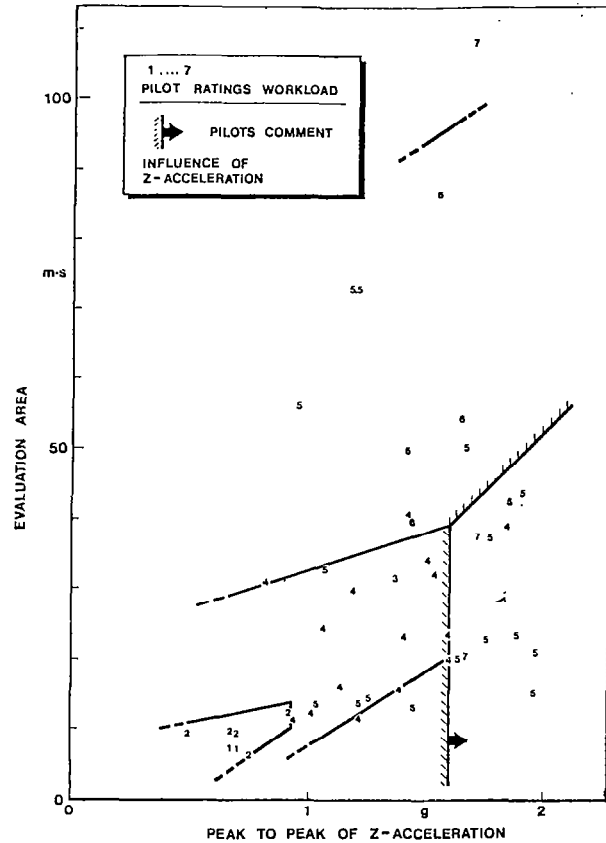
Fig. 12 Pilot rating trends with z-acceleration and evaluation area
