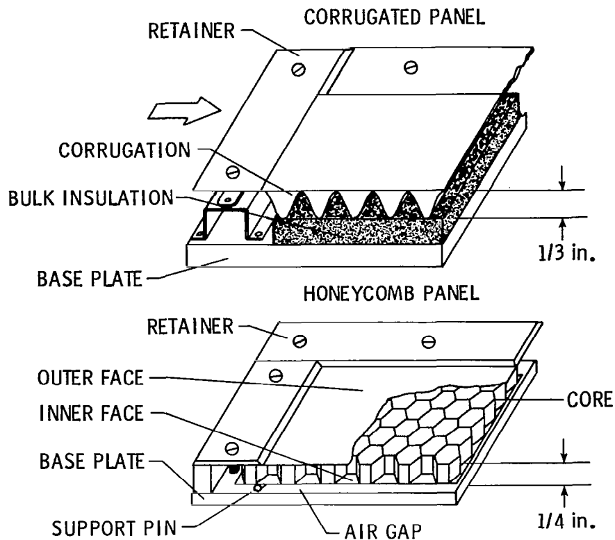
Figure 21.- Insulating panels.
