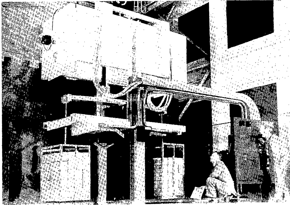
Figure 23.- Creep test equipment.
