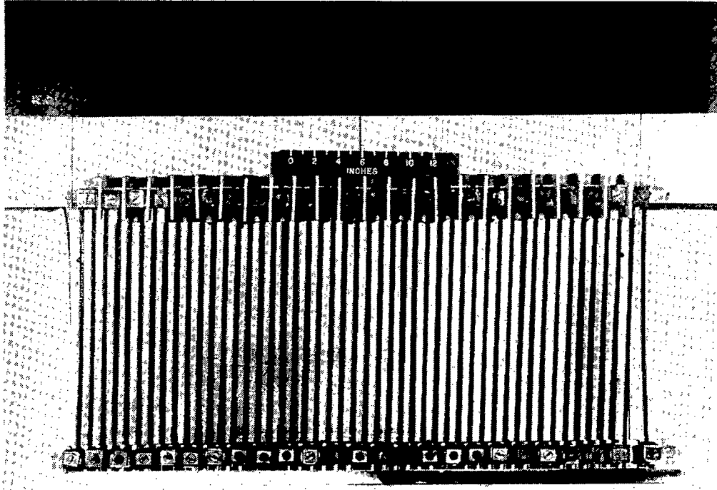
Figure 24.- Carbon-rod heat radiator.
