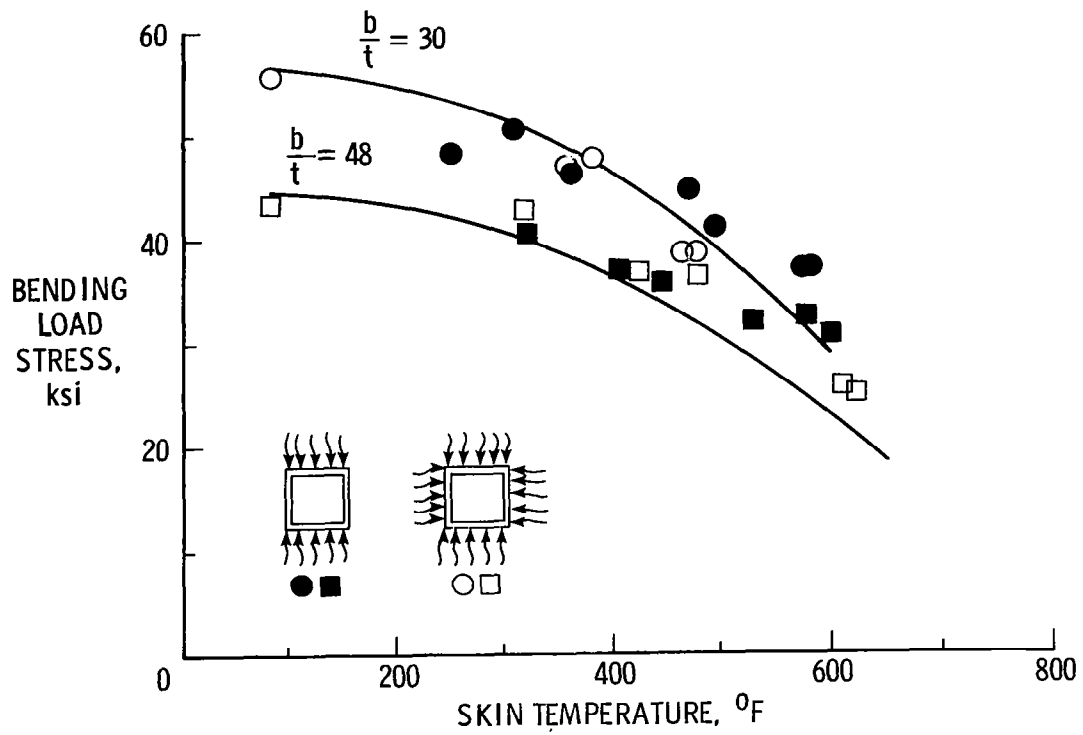
Figure 15. Rapid-heating effects on failure of 2014-T6 aluminum alloy beams. T = 100^\circ\text{F}/\text{sec} .
