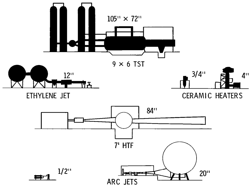
Figure 26.- Operational (black) and planned hot jets and tunnels in April 1959.
