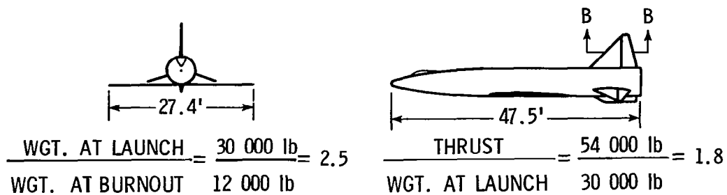
Figure 27.- Principal features of proposed X-15 research airplane defined during 1954.
