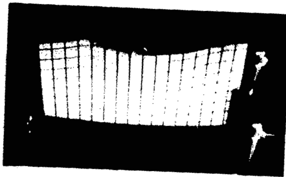
Figure 19.- Jet test of wing structure.
