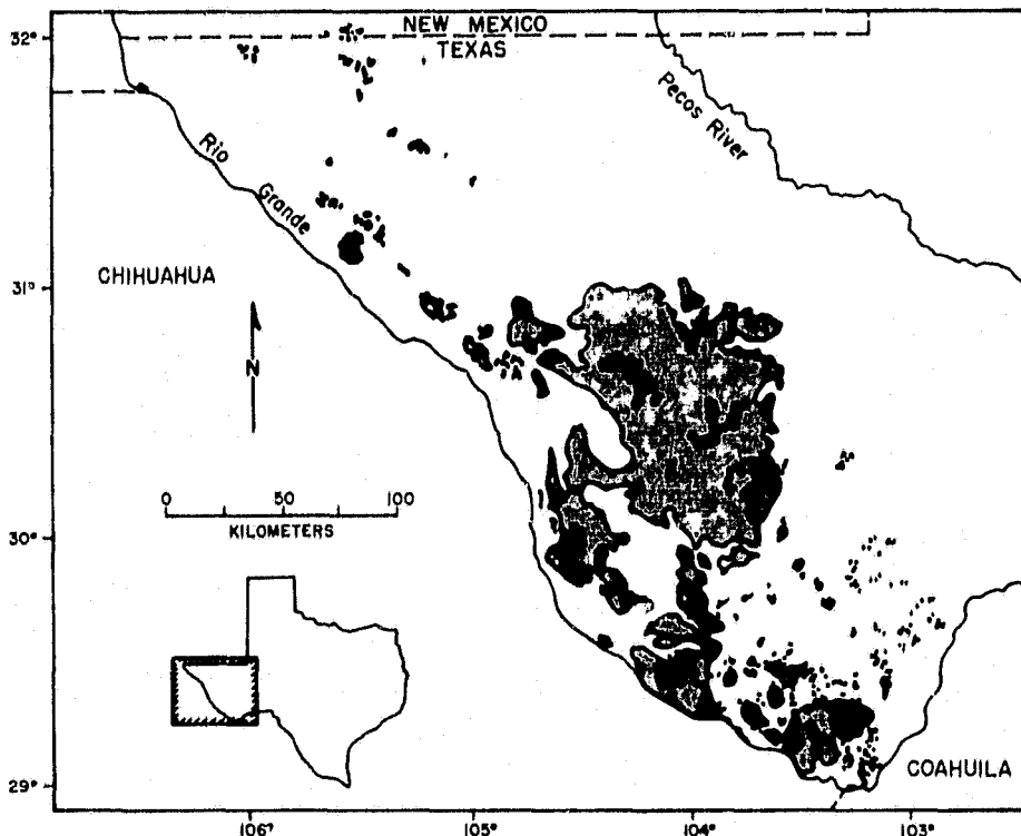
Figure 1. Distribution of Cenozoic igneous rocks, Trans-Pecos magmatic province. Intrusive rocks are shown in black; lavas and pyroclastic rocks are shown by stippled pattern. (Barker, 1977)
