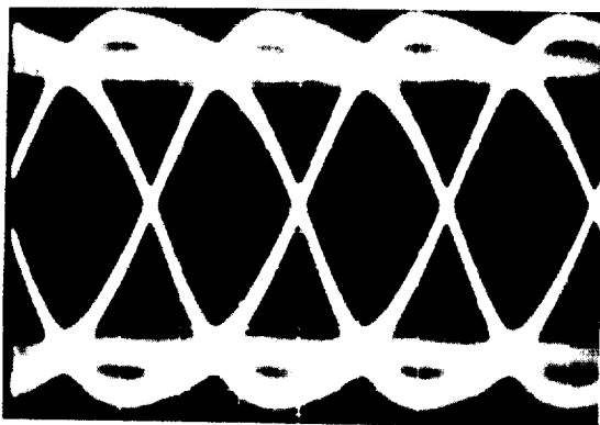
Figure 10-5.—Delay modulation.
