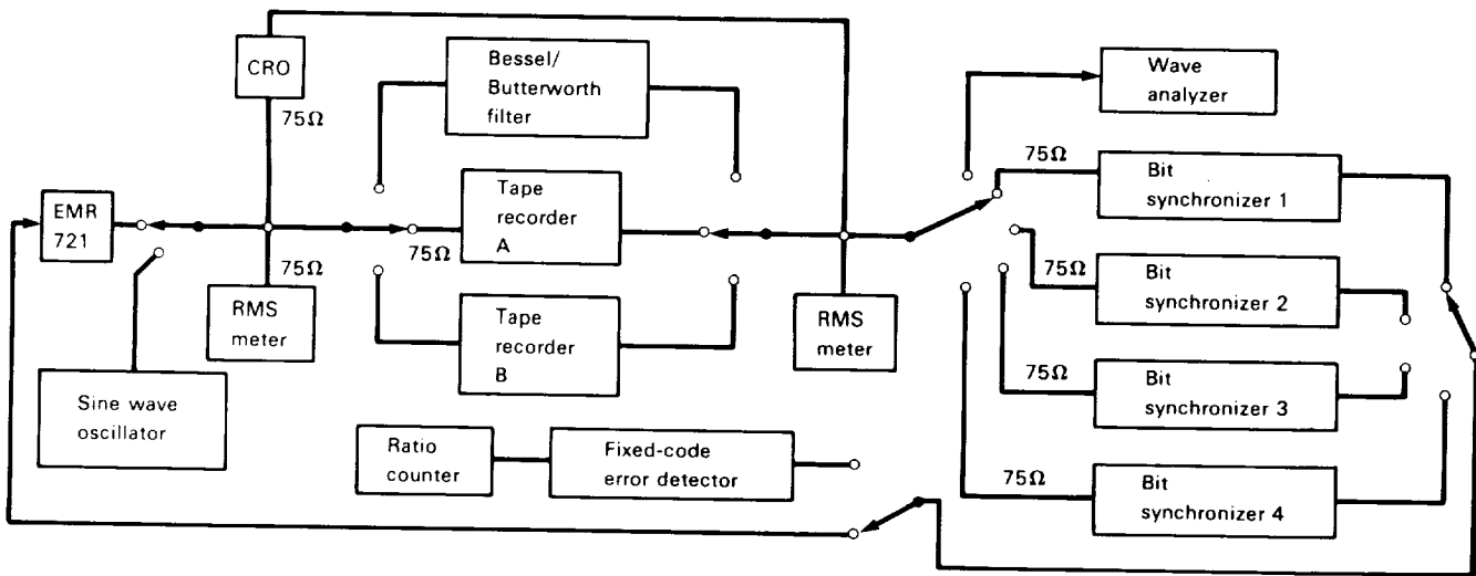
Figure 10-3.—Test configuration (ref. 10-5).
