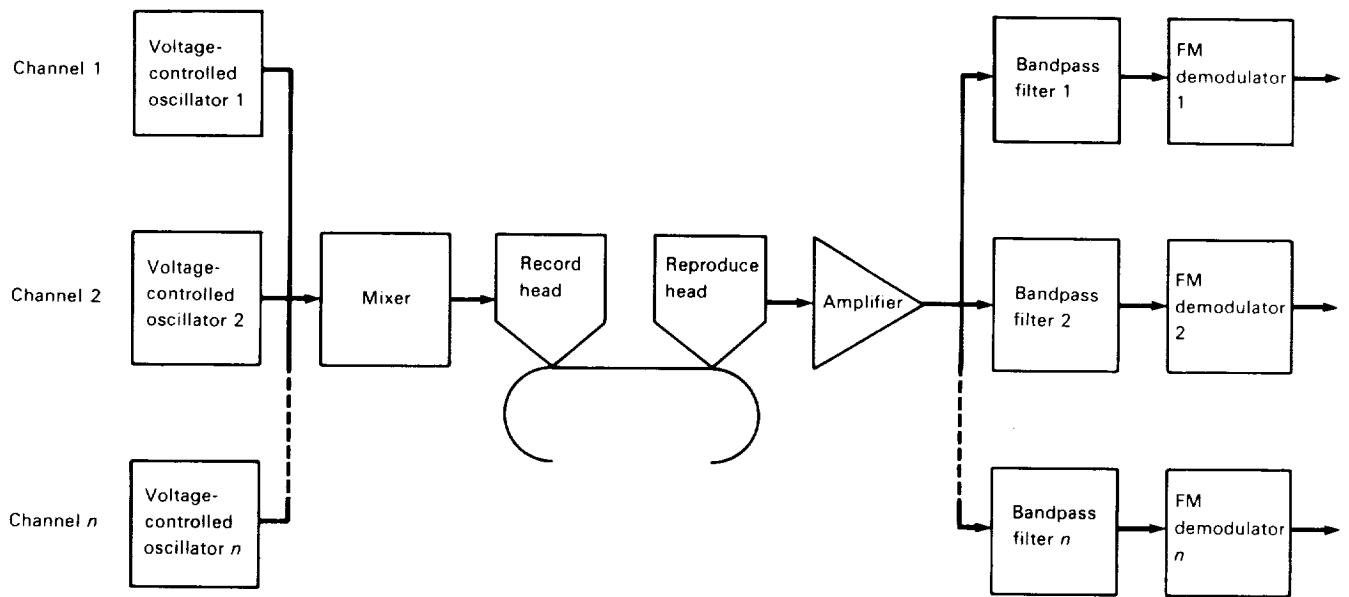
Figure 9-4.—FM multiplex.
