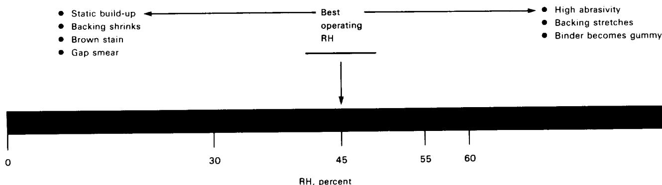
Figure B-10.—Effect of relative humidity on magnetic tape and transport.
