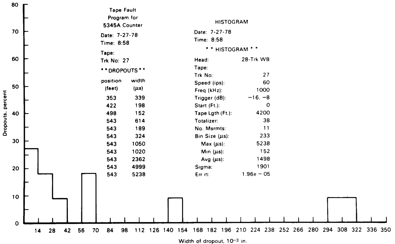
Figure 4-3.—Plotter output.
