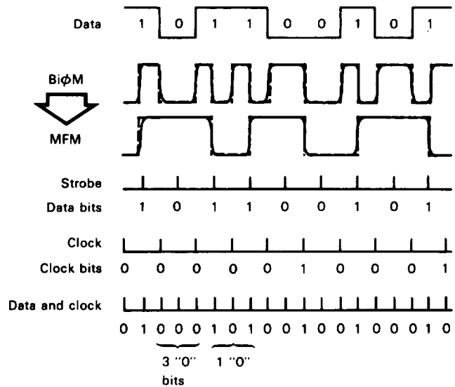
Figure 8-13.—MFM recording.
