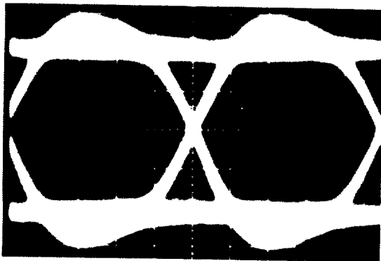
Figure 10-4.—NRZ-L.
