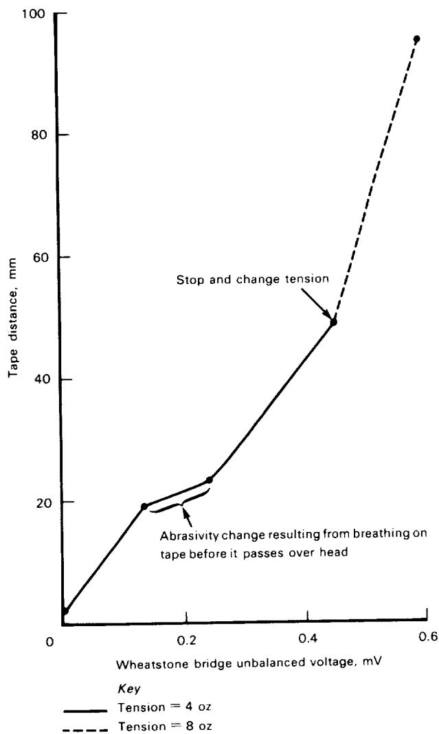
Figure 3-6.—Typical readout showing effect of humidity change with thin film method of measuring head wear. (Tape width = 1/2 in.; tape speed = 7 1/2 in./s; Temperature (ambient room) = 21° C; relative humidity (ambient) = 63 percent; chart speed: 30 mm/min.)
