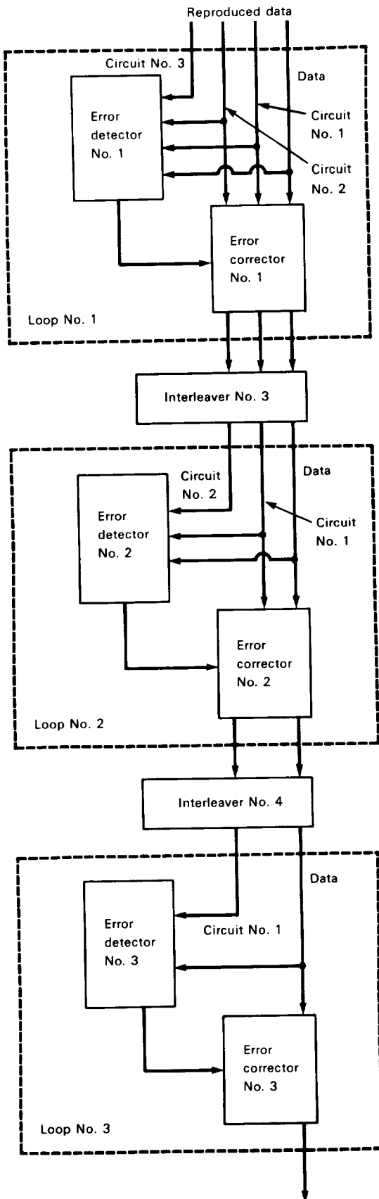
Figure 10-13.—EDAC decoder.
