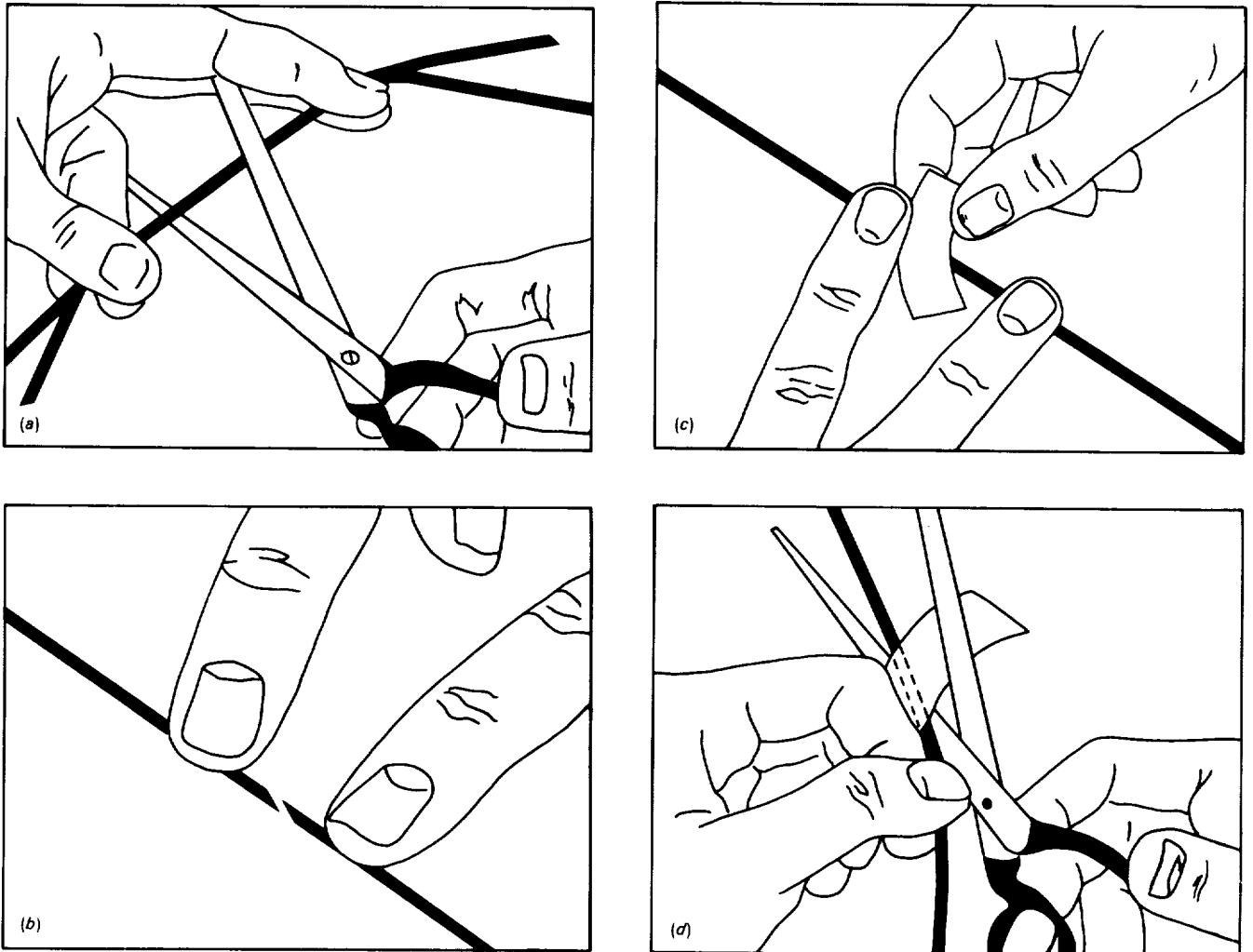
Figure B-14.—Making tight, noise-free splices. (a) Overlap the two ends and cut. (b) Align both ends, uncoated side up. (c) Cover with splicing tape. (d) Trim excess splicing tape.
