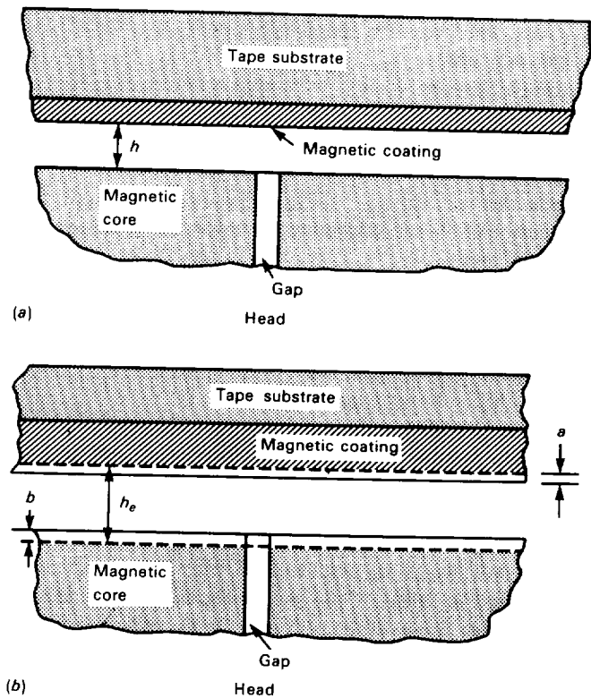
Figure C-15.—Head-to-tape separation. (a) Mechanical. (b) Effective. a = nonmagnetic or low permeability coating on tape surface; b = nonmagnetic coating on head surface; h_e = h + a + b .
