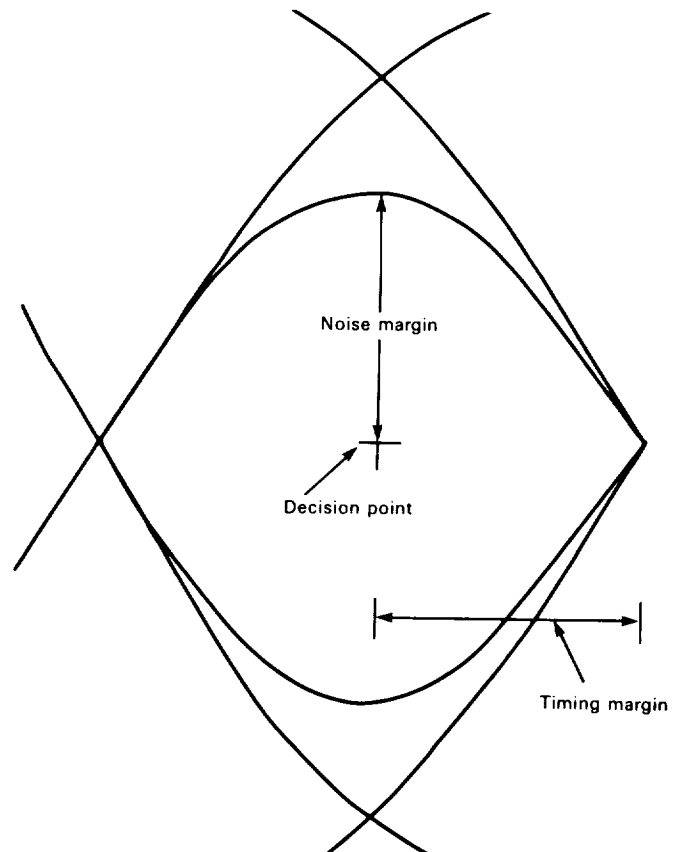
Figure 10-6.—Eye pattern.
