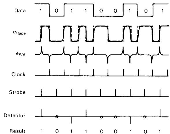
Figure 8-10.— \text{Bi}\phi\text{M} recording.
