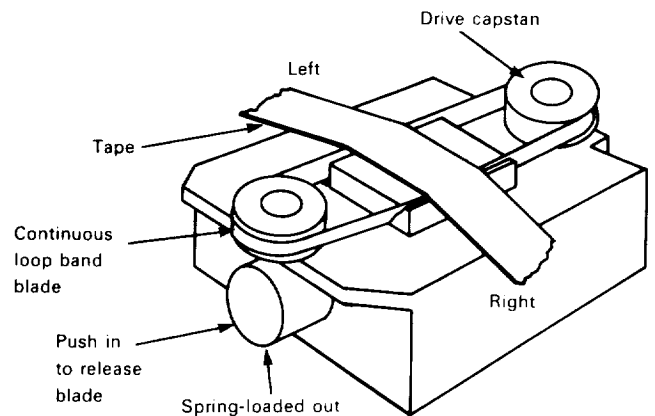
Figure 6-2.—GKI endless loop band blade cleaner.
