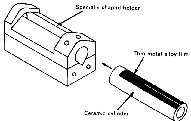
Figure 3-5.—Dummy head configuration.
