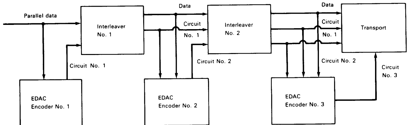
Figure 10-12.—EDAC encoder. (CT = correction track.)
