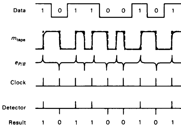
Figure 8-11.—BIϕL recording.
