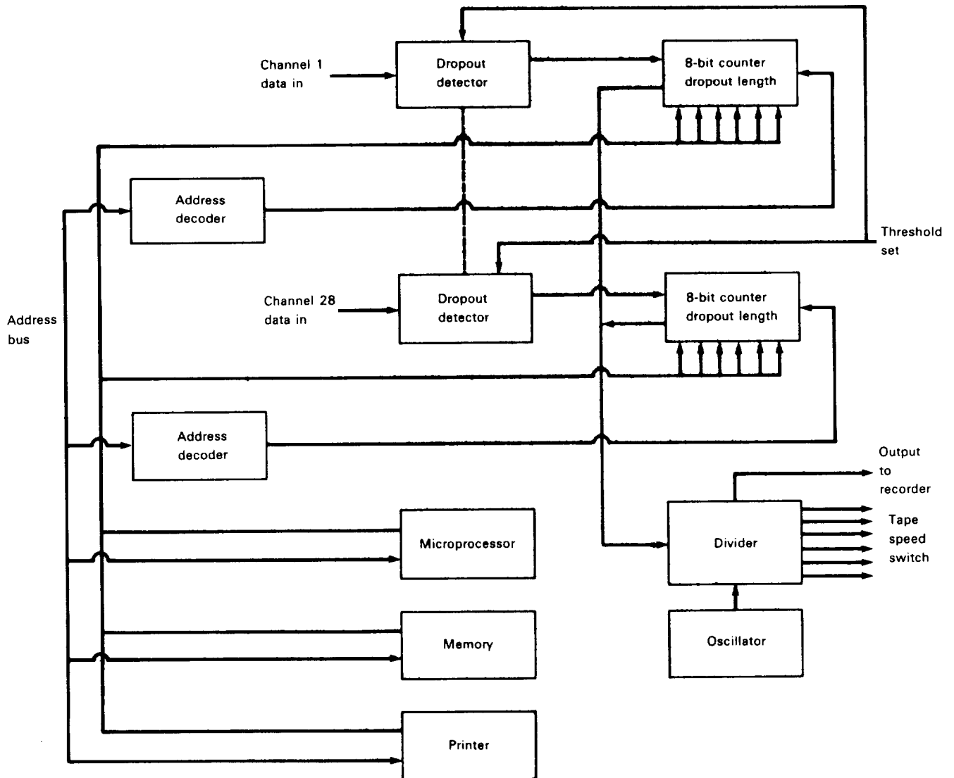
Figure 10-9.—Dropout tester.
