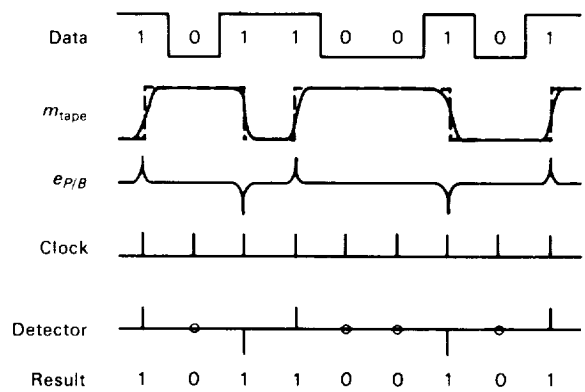
Figure 8-9.—NRZI recording.
