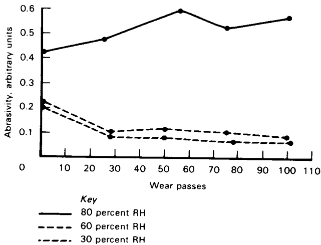
Figure 3-2.—Head wear of Ampex 797A recording tape measured using the radicon technique.
