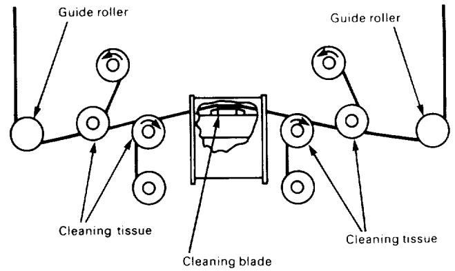
Figure 6-1.—Tape path.
