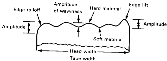
Figure C-3.—Schematic diagram of wavyness, edge rolloff, and edge lift.
