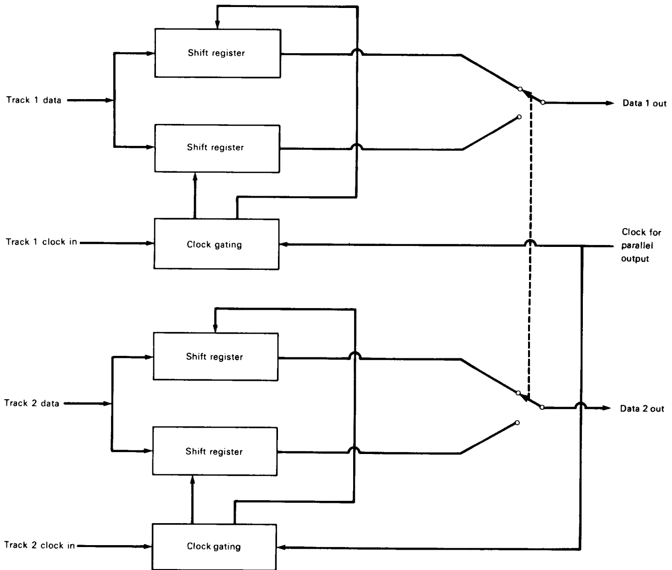
Figure 10-1.—“Ping-pong” buffer.
