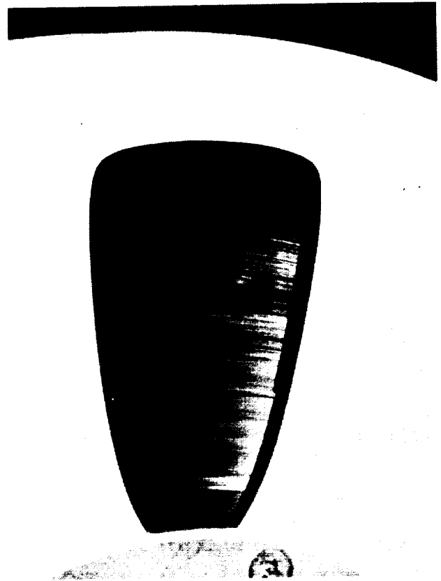
Figure 5-8.—Windowed tape pack. Windows are see-through air gaps in tape winding.
