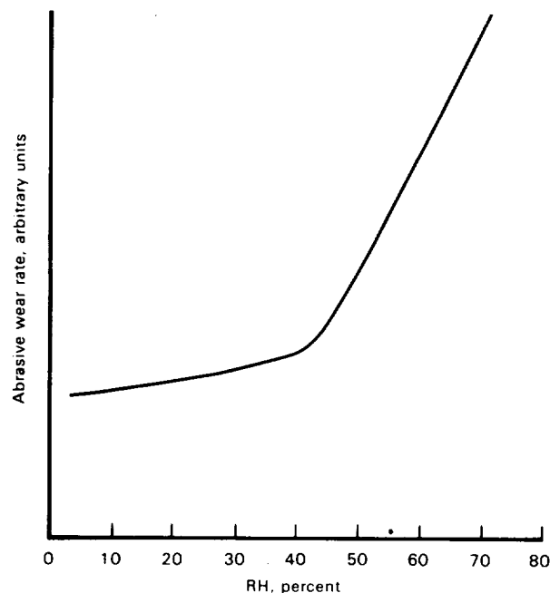
Figure 2-4.—Head wear as a function of RH.
