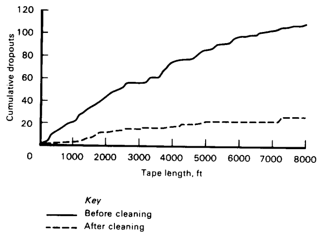
Figure 10-10.—Dropout test on tape (type A) performed at 120 in./s and 1 MHz.
