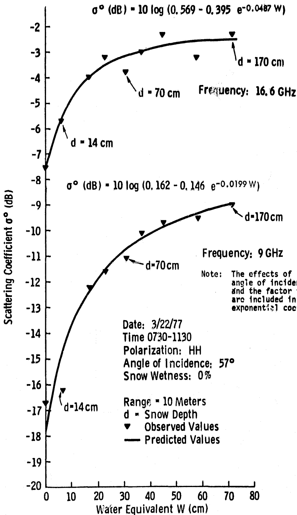
Figure III-17.- Scattering coefficient response to snow water equivalent (after Ulaby and Stiles, 1980).
