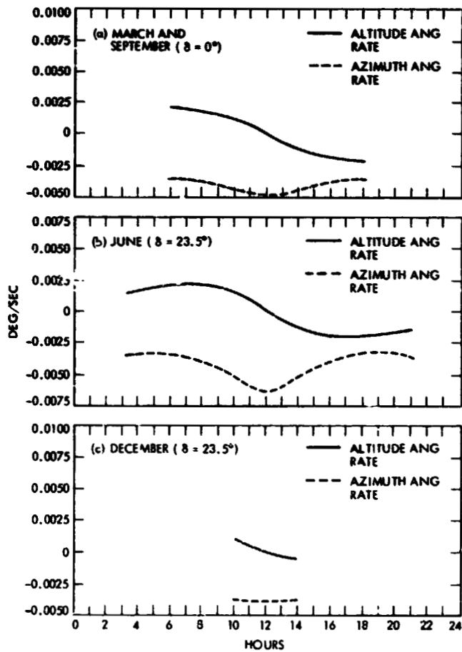
Fig. 8. Rates of solar angles for 60.00 deg north latitude
