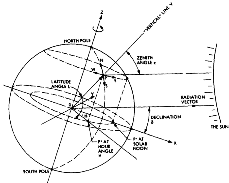
Fig. 2. Earth-sun angles
