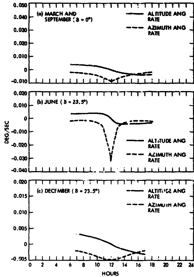
Fig. 7. Rates of solar angles for 30.00 deg north latitude
