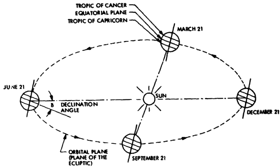
Fig. 1. The earth's motion around the sun
