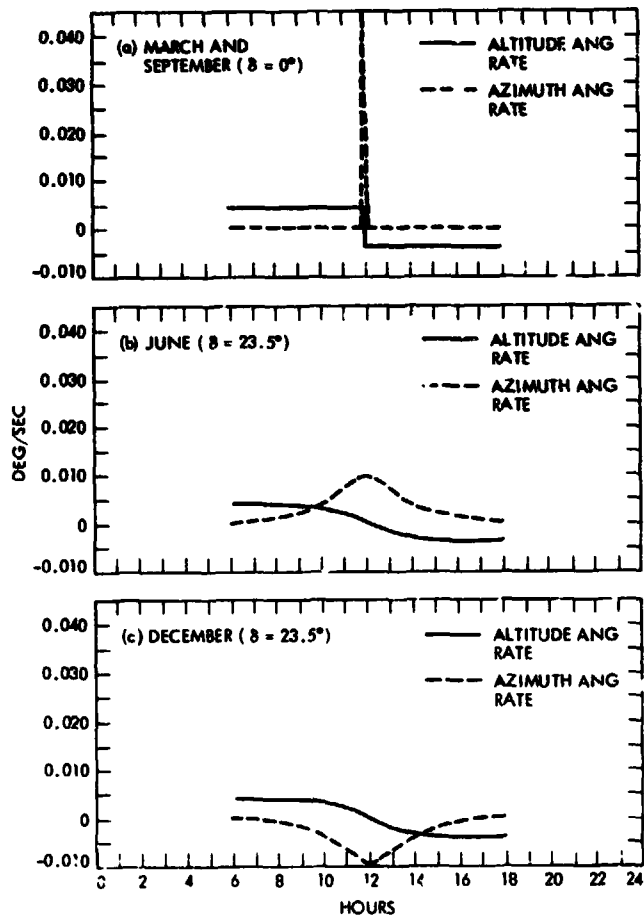
Fig. 6. Rate of solar angles for the equator
