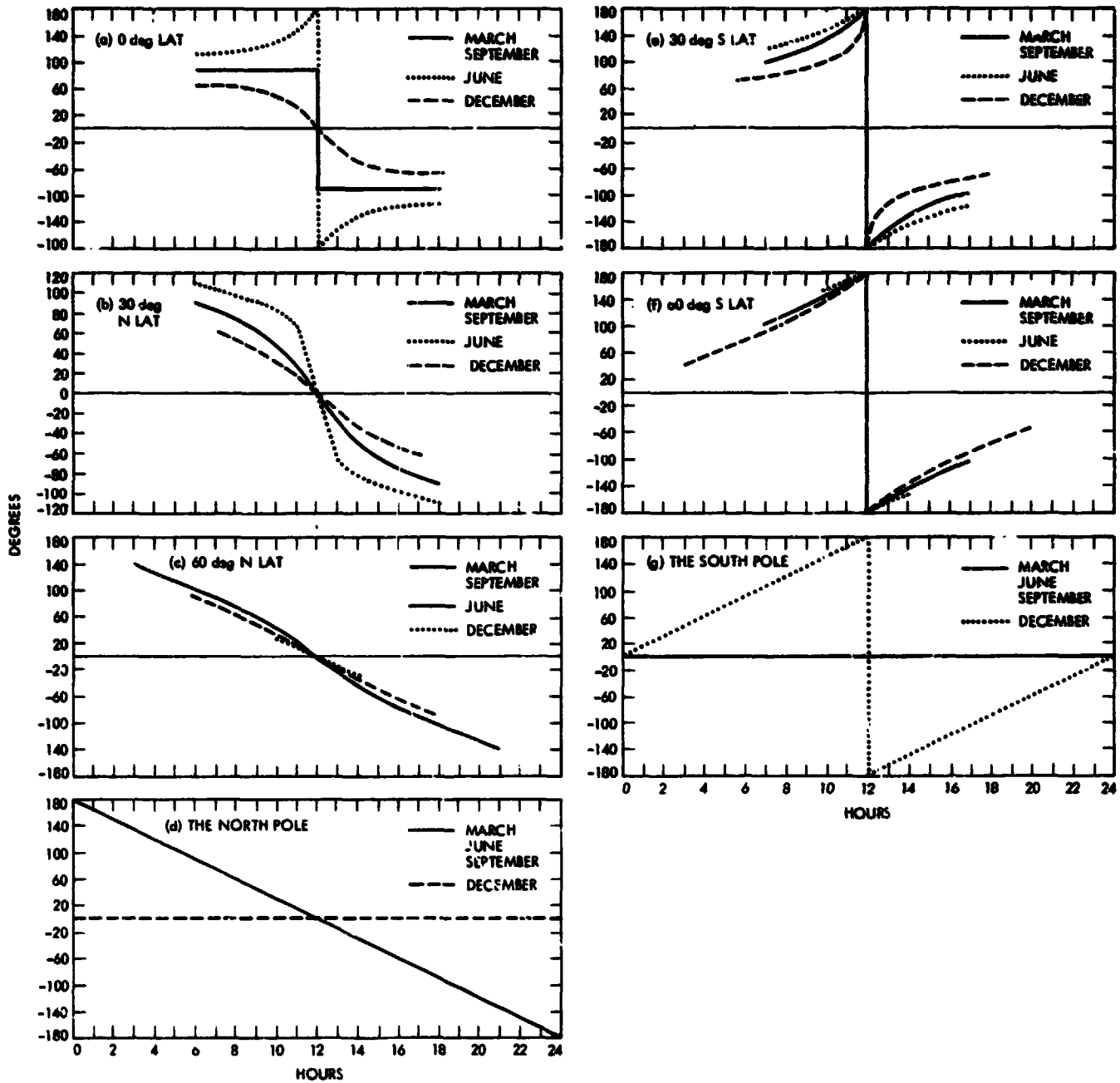
Fig. 8. Comparison of solar azimuth angles for seven different latitudes
