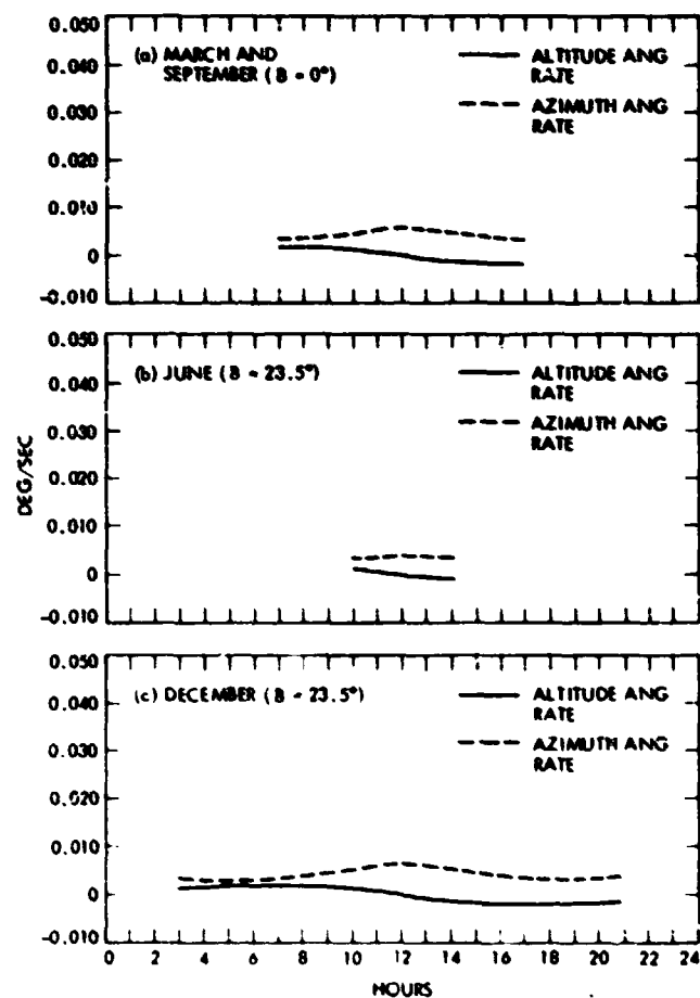
Fig. 10. Rates of solar angles for 60.00 deg south latitude
