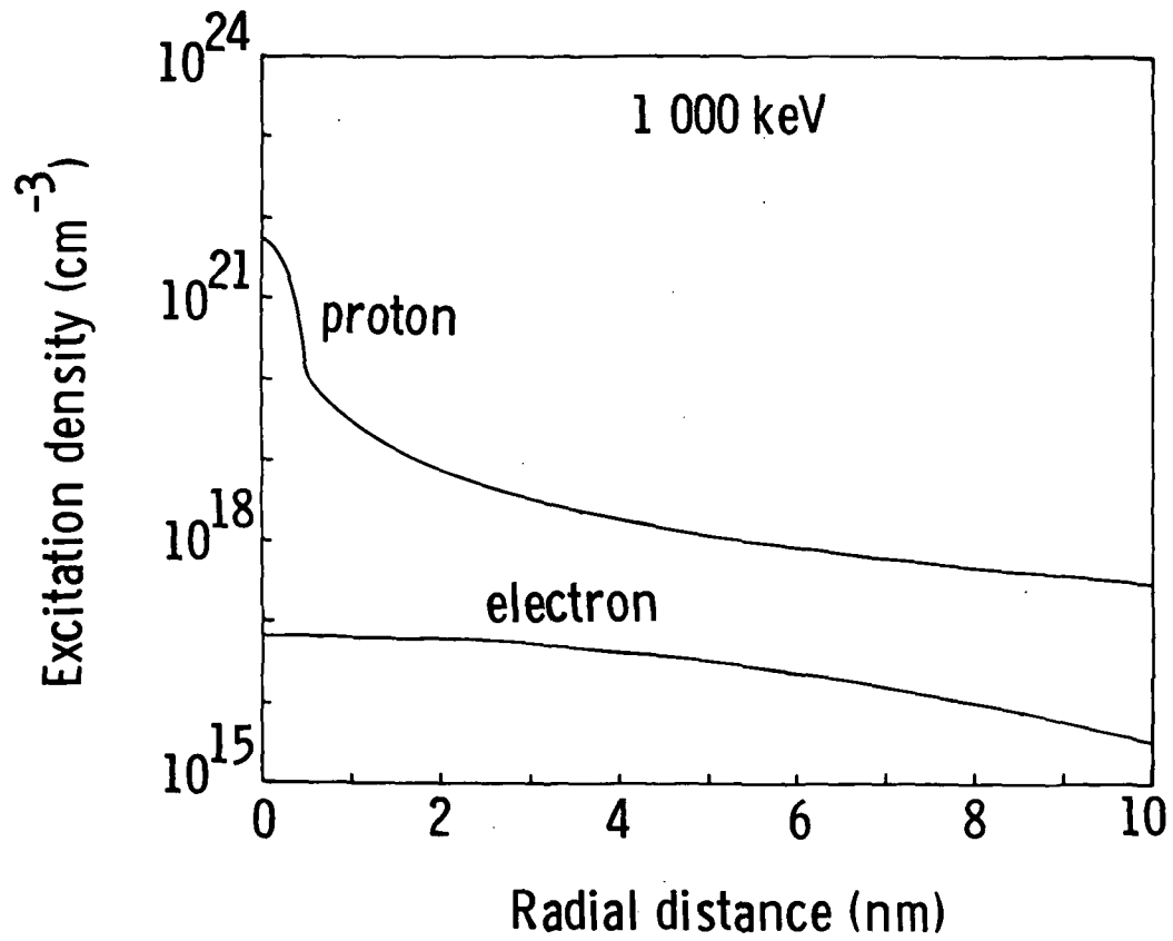
Fig. 13. Excitation density near 1 000 keV particle path.
