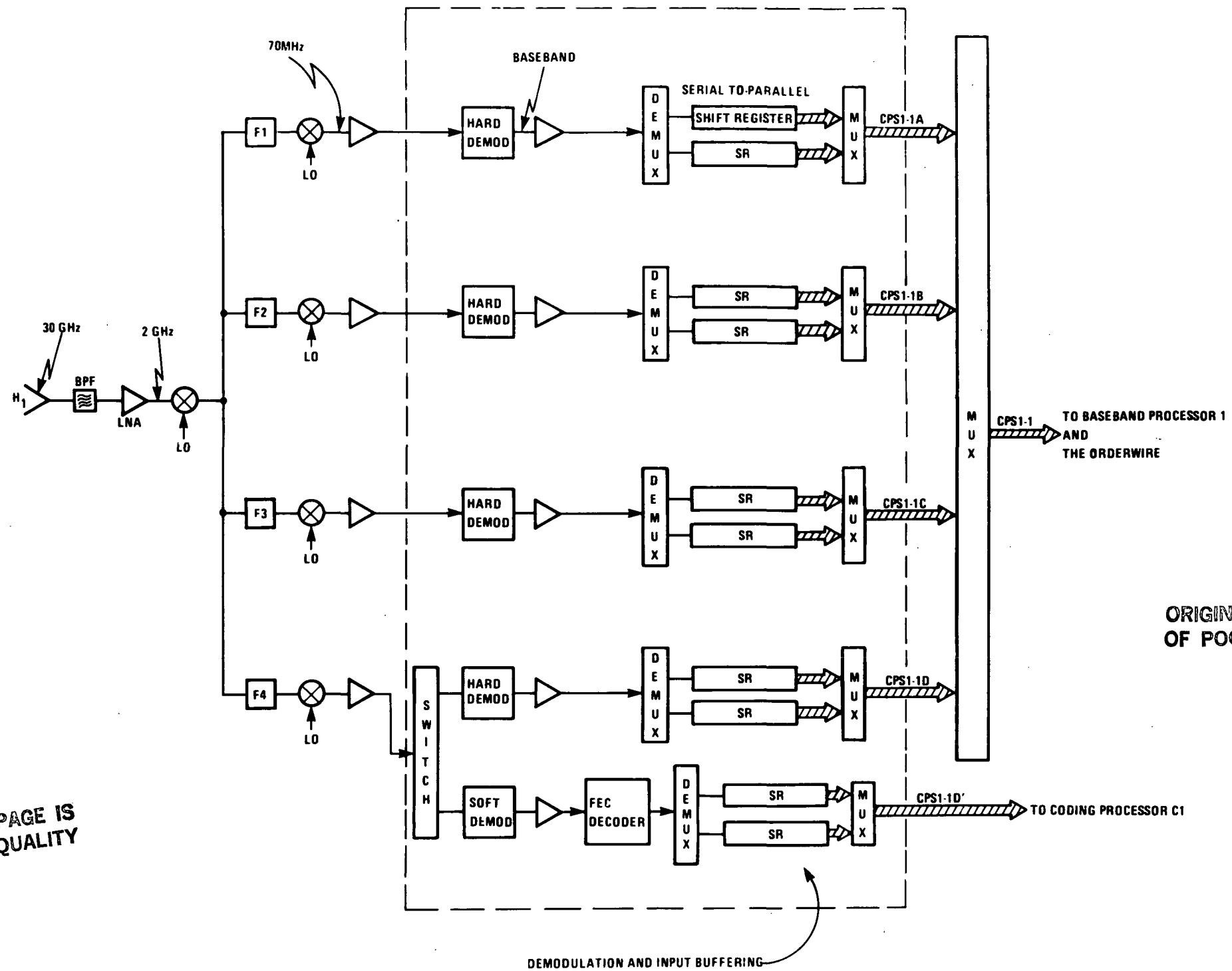
Figure 7-7. Demodulators and Input Buffering
