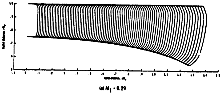
Figure 4-47. - Computed streamwise velocity profiles for diffuser flow.
