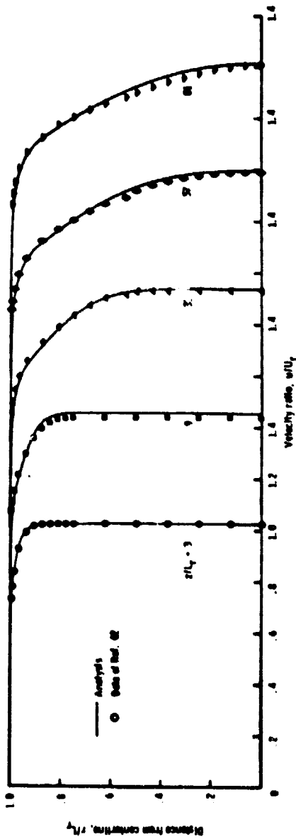
Figure 4-26. - Computed and experimental velocity profiles in turbulent developing pipe flow, Cebeci-Smith turbulence model.
