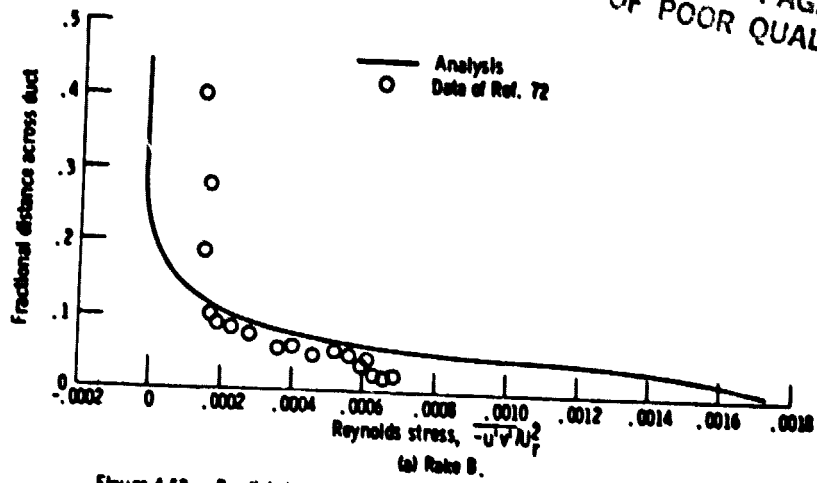
Figure 4-52 - Predicted and experimental Reynolds stress profiles for diffuser flow, M_f = 0.29 .
