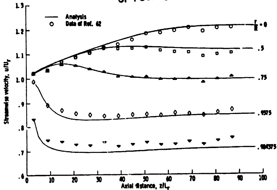
Figure 4-24. - Computed and experimental streamwise velocities in turbulent developing pipe flow, Cebeci-Smith turbulence model.
