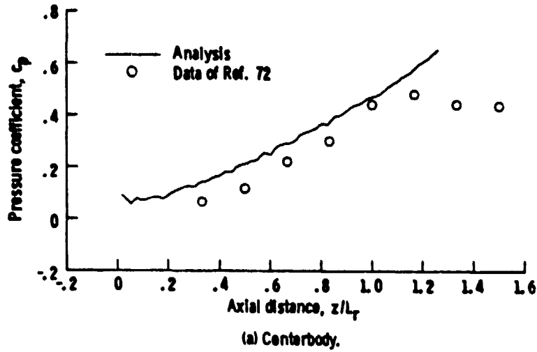
Figure 4-44. - Imposed pressure coefficients compared with data for diffuser flow, M_1 = 0.29 .
