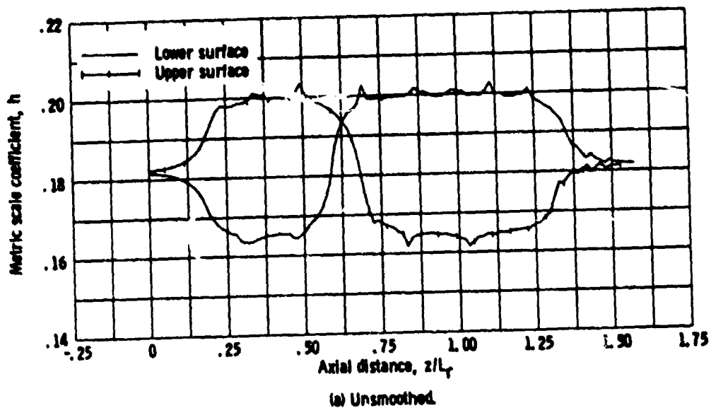
Figure 4-33. - Metric scale coefficients for S-shaped duct flow.
