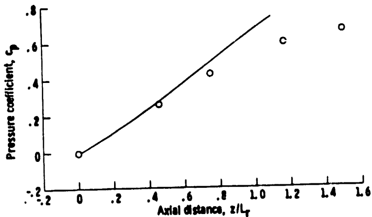
(b) Cowl.
