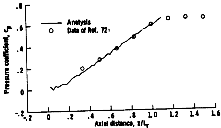
(a) Centerbody.
