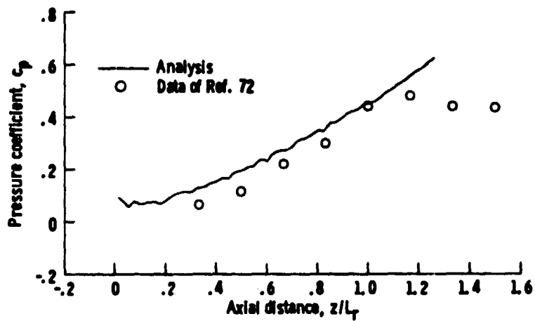
(a) Centerbody.
