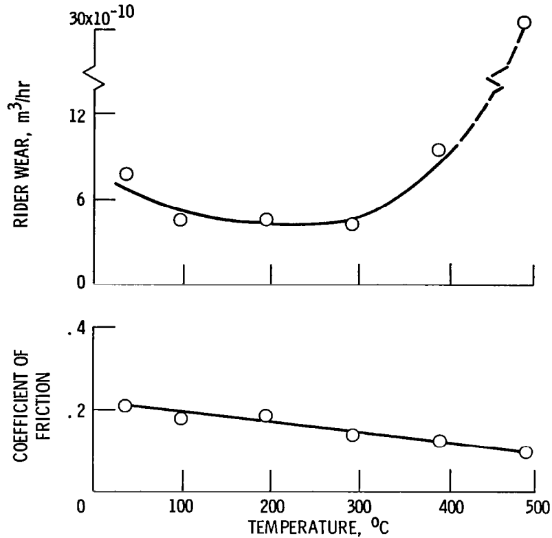
Figure 5.- Friction and wear of cobalt alloy sliding on itself at various temperatures and lubricated with a chlorinated fluorocarbon.
