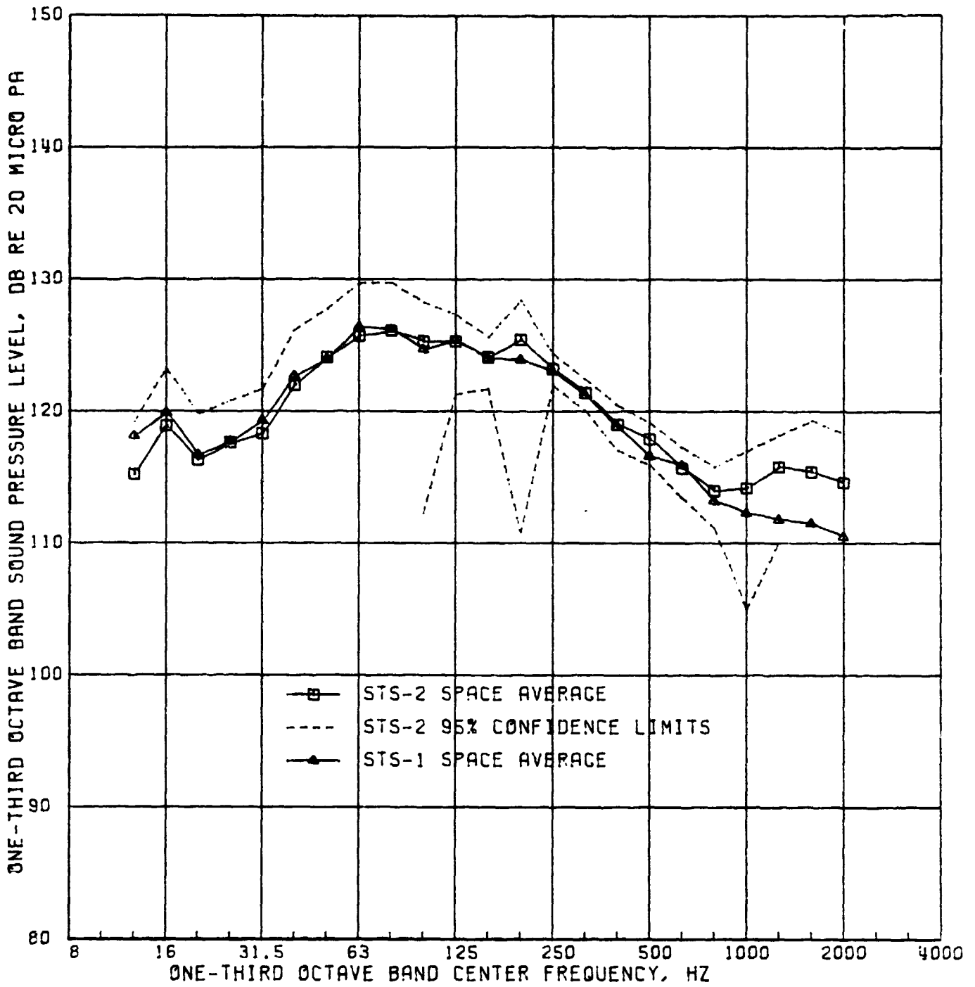
FIGURE 9. ALTERNATIVE ESTIMATE OF SPACE-AVERAGE SOUND PRESSURE LEVELS IN PAYLOAD BAY FOR STS-2
