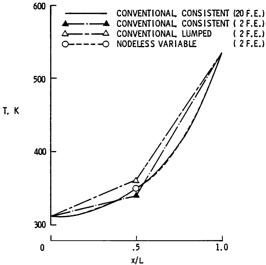
(b) COMPARATIVE TEMPERATURE DISTRIBUTIONS
