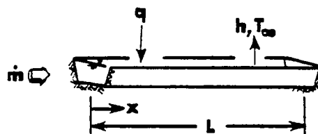
Case 8. FLOW PASSAGE
