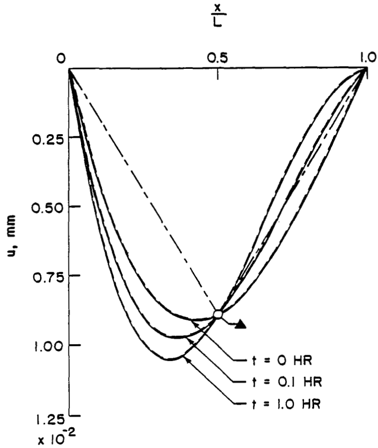
(c) COMPARATIVE DISPLACEMENT DISTRIBUTIONS
