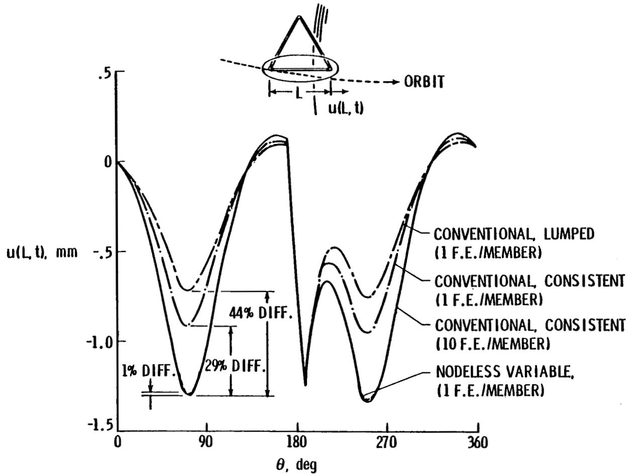
(c) Comparative displacements of a three member orbiting truss.
