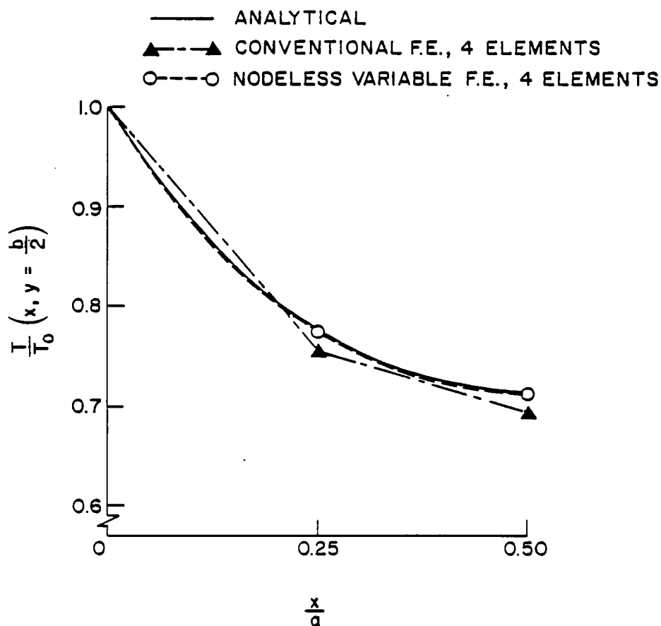
(c) COMPARATIVE TEMPERATURE DISTRIBUTIONS ALONG y = \frac{b}{2} .
