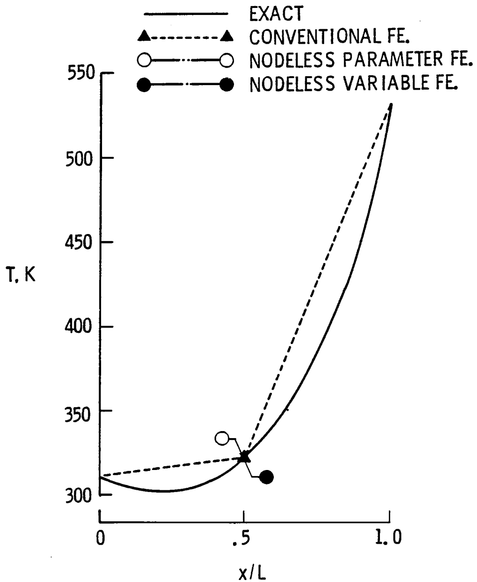
(b) Comparative temperature distributions at t = 0 s.
