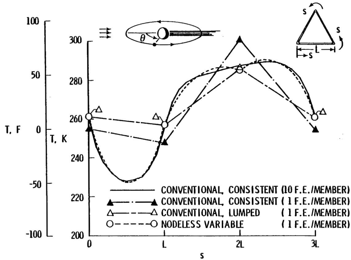
(b) Comparative temperature distribution of a three member orbiting truss at \theta = 60 degrees.
