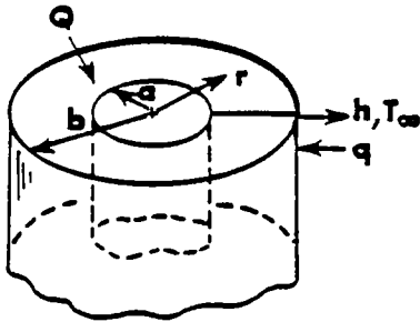
Case 3. HOLLOW CYLINDER
