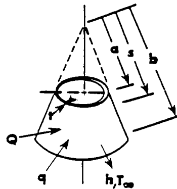
Case 6. CONICAL SHELL
