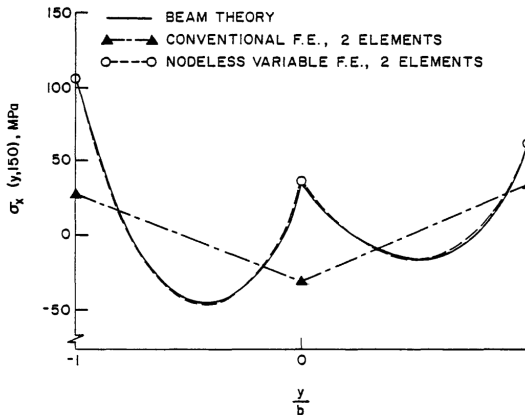
(c) COMPARATIVE THERMAL STRESS DISTRIBUTIONS ALONG CHORDWISE DIRECTION, t = 150 s.
