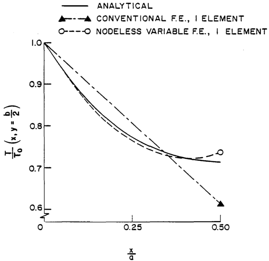
(b) COMPARATIVE TEMPERATURE DISTRIBUTIONS ALONG y = \frac{b}{2} .
