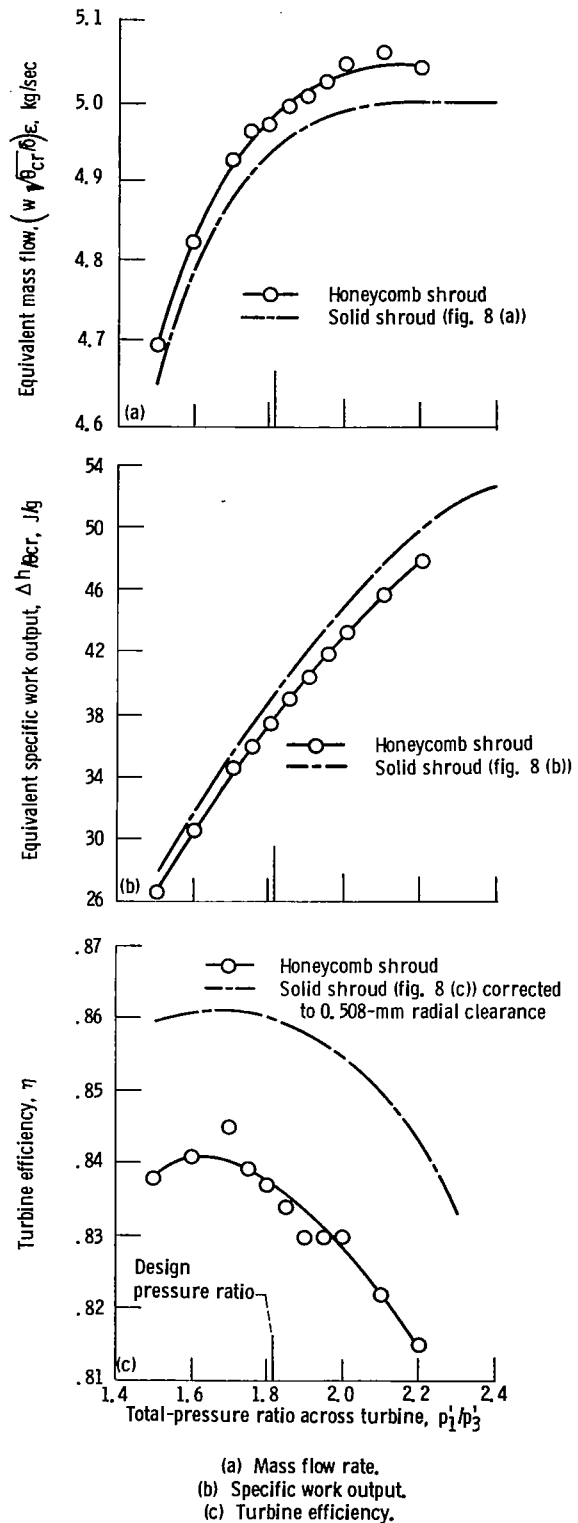
Figure 9. - Effect of honeycomb shroud on turbine performance with no coolant flow at design speed.
