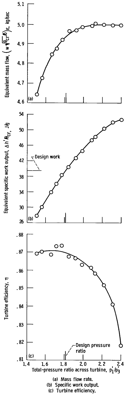
Figure 8. - Performance of turbine with solid rotor shroud at design speed.
