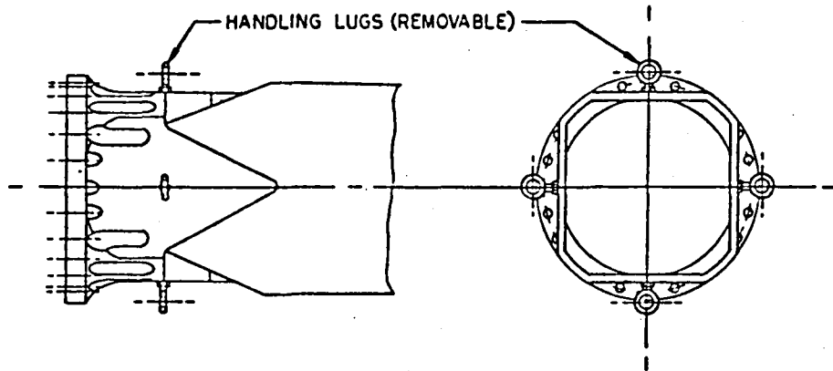
FIGURE 34 - ROOT END HANDLING POINTS
