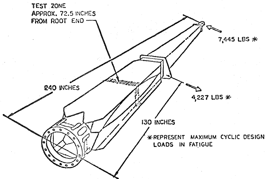
FIGURE 36 - ROOT END TEST BEAM
