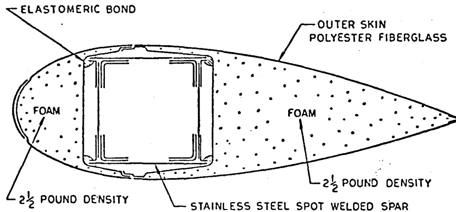
FIGURE 7 - TYPICAL SECTION WIND TURBINE BLADE
