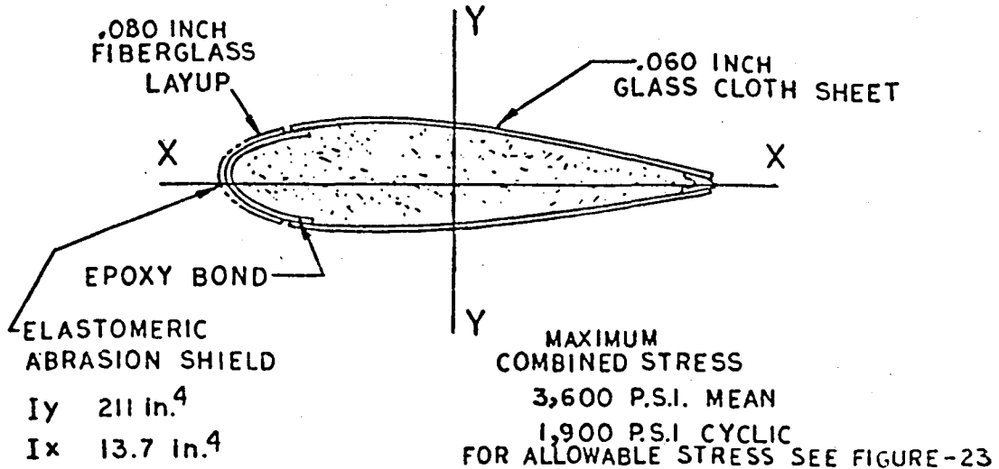
FIGURE 28 - SECTION FIBERGLASS OF TIP EXTENSION
