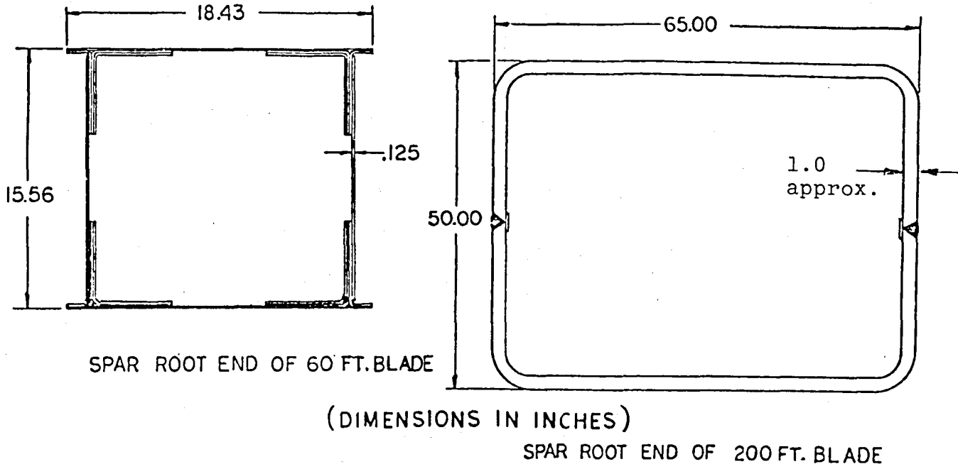
FIGURE 14 - SPAR ROOT END OF 60 FT. AND 200 FT. BLADE
