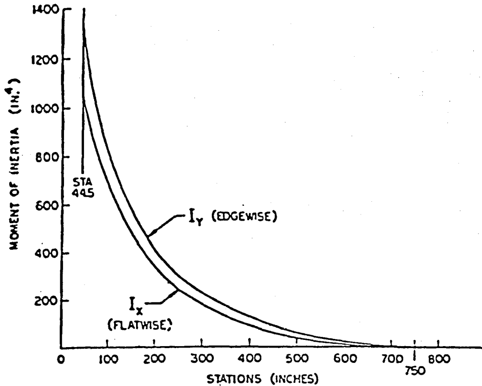
FIGURE 27 - SPAR MOMENT OF INERTIA
