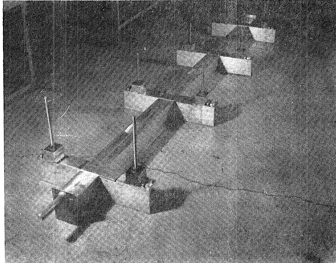
FIGURE 39 - TEMPORARY FIXTURE FOR TEST BEAM SIDE AND TOP PLATE ASSEMBLIES
