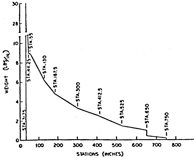
FIGURE 24 - BLADE MASS DISTRIBUTION
