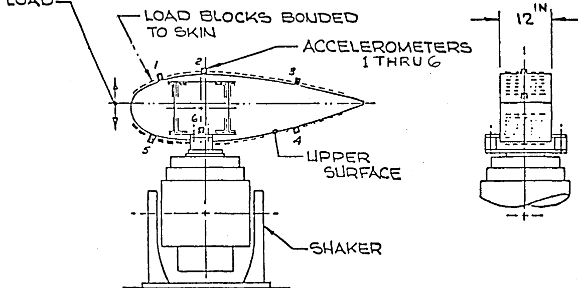
FIGURE 19 - AERODYNAMIC LOADING OF BONDING SURFACES
