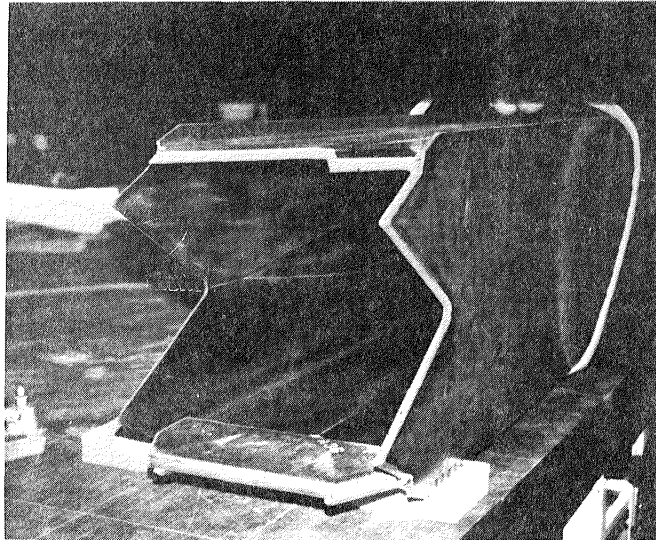
FIGURE 41 - ASSEMBLED BOX SPAR
