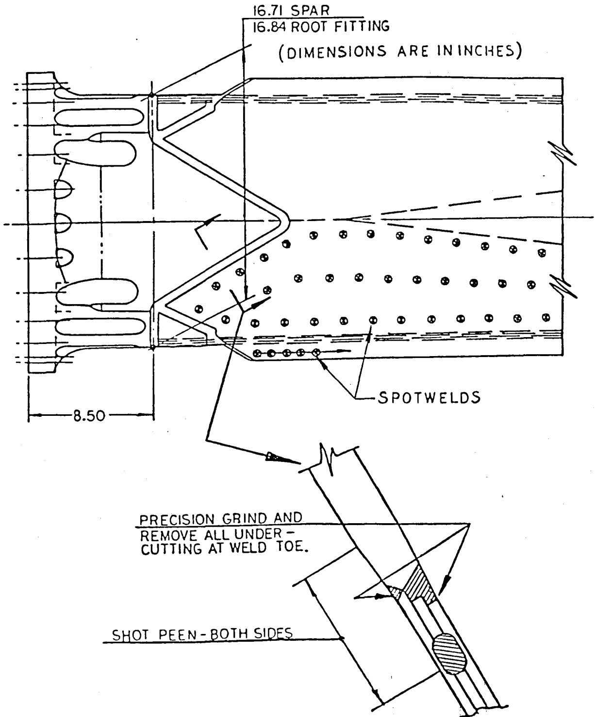
FIGURE 30 - ROOT END - SPAR CONFIGURATION
