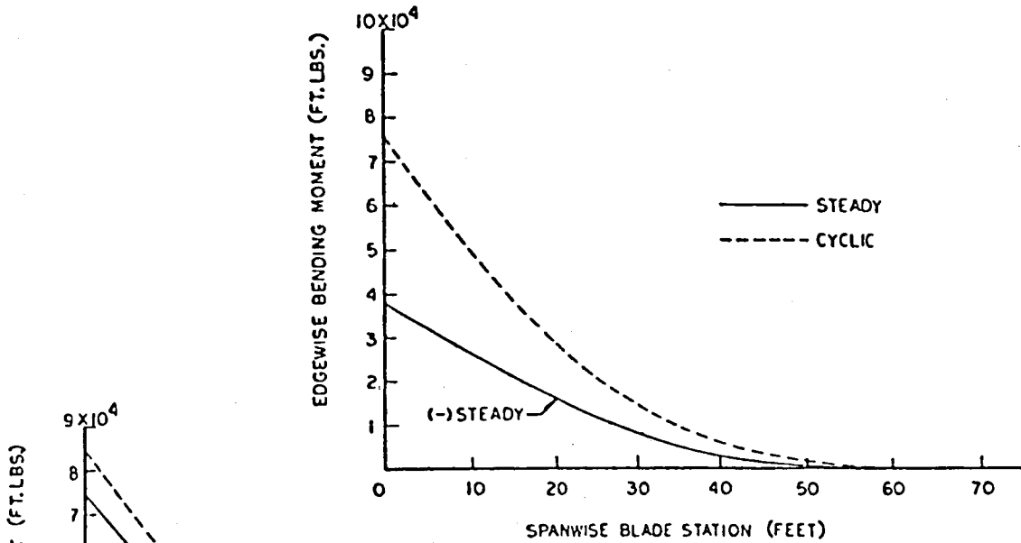
FIGURE 25 - EDGEWISE BENDING LOADS
