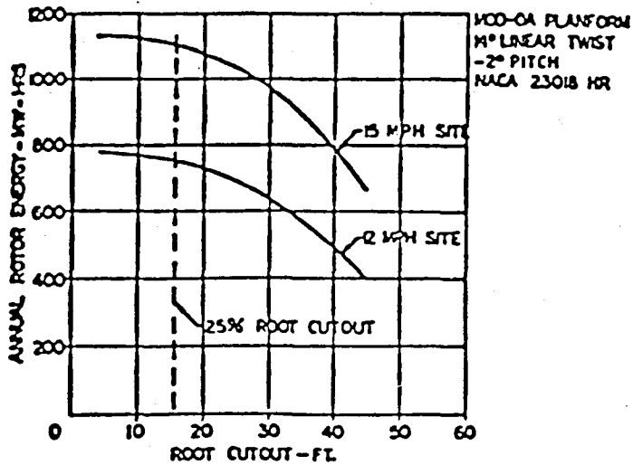
FIGURE 2 - EFFECT OF ROOT CUTOUT ON ANNUAL ENERGY
