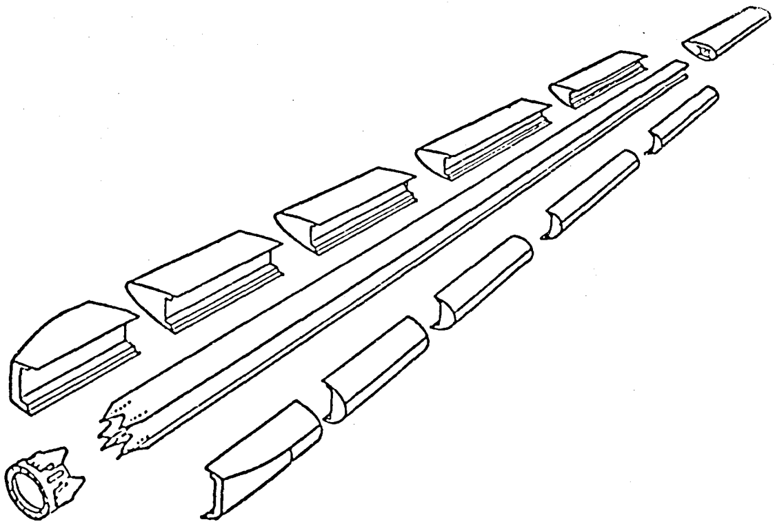
FIGURE 9 - MAJOR SUB-ASSEMBLY
