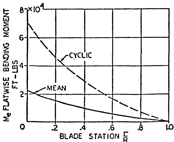
FIGURE 3 - FLATWISE & EDGEWISE BENDING MOMENT DISTRIBUTIONS
