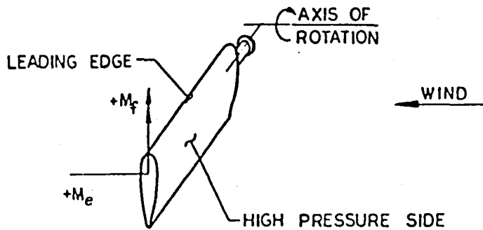
FIGURE 5 - BENDING MOMENT SIGNS CONVENTIONS
