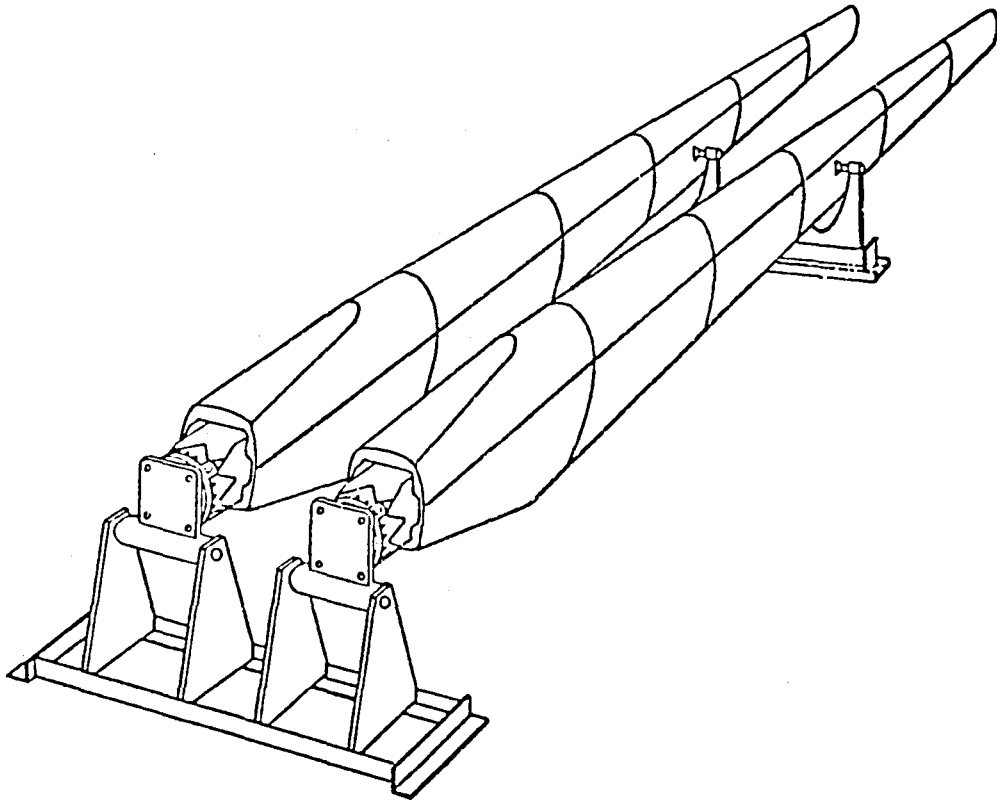
FIGURE 33 - SHIPPING FIXTURE ARRANGEMENT
