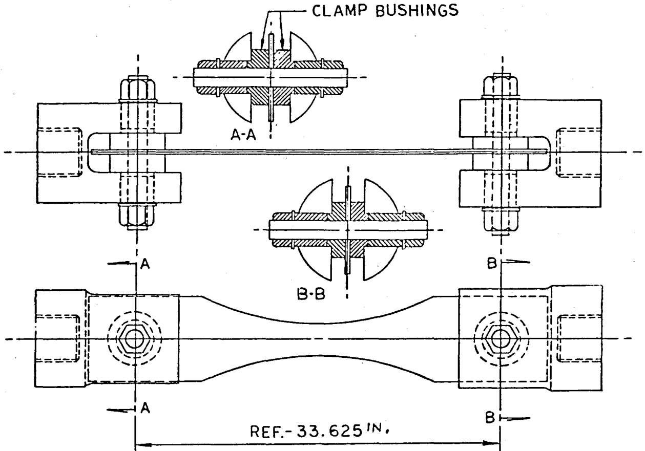
FIGURE 16 - TYPICAL FATIGUE SPECIMEN CONFIGURATION
