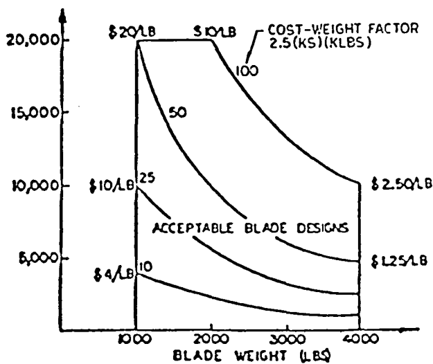
FIGURE 6 - BLADE WEIGHT VERSUS BLADE COST
