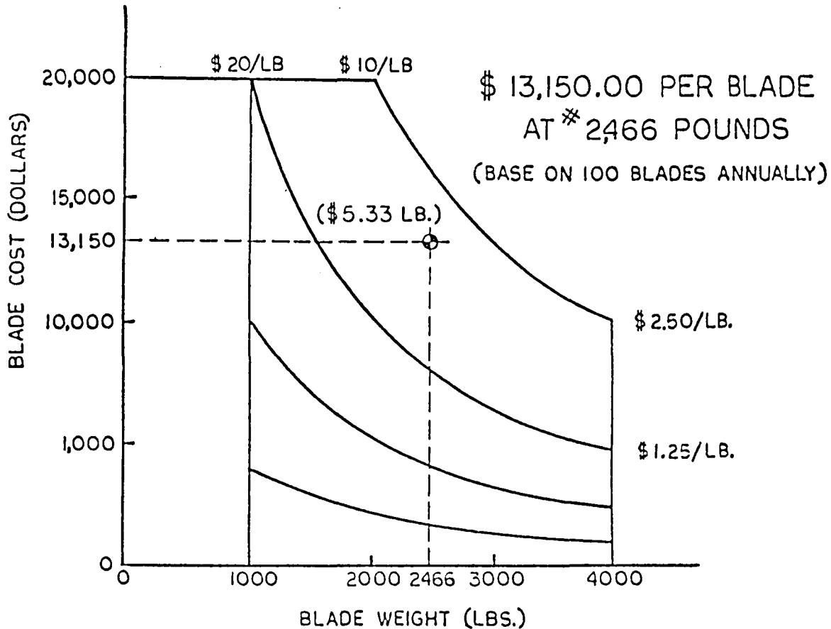
COST VERSUS WEIGHT DIAGRAM (COST CURVES FROM BASIC N A S A DATA)
