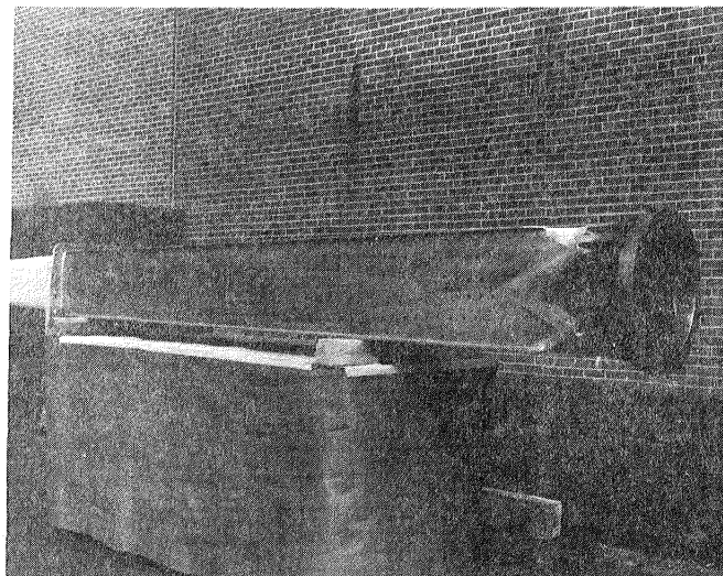
FIGURE 42 - ARC WELDING CONFIGURATION OF 4130 ROOT END FITTING TO STAINLESS STEEL BOX SPAR
