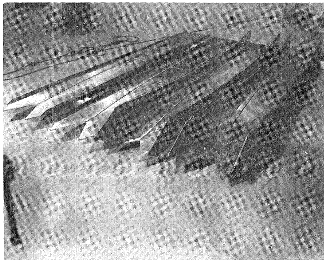
FIGURE 40 - FOUR ASSEMBLIES READY FOR BOX SPAR
