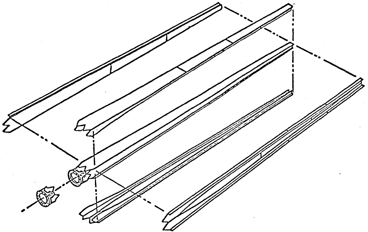
FIGURE 8 - EXPLODED SPAR ASSEMBLY
