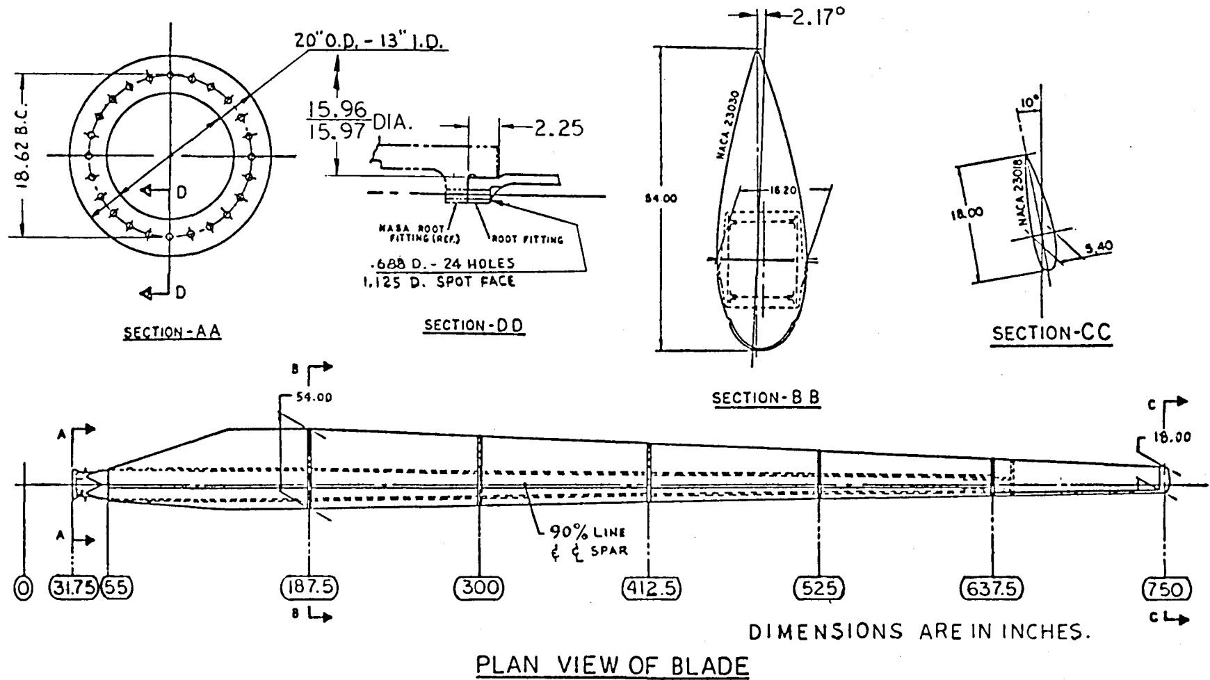
FIGURE 29 - 62 FT. BLADE CONFIGURATION
