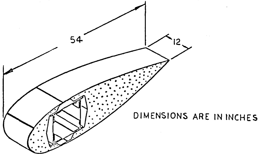
FIGURE 18 - TEST SPECIMEN AERODYNAMIC SURFACE
