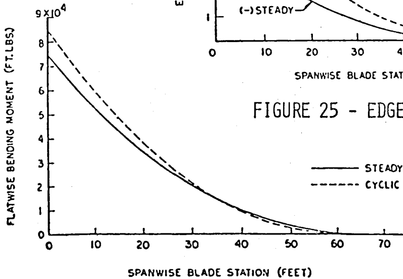
FIGURE 26 - FLATWISE BENDING LOADS
