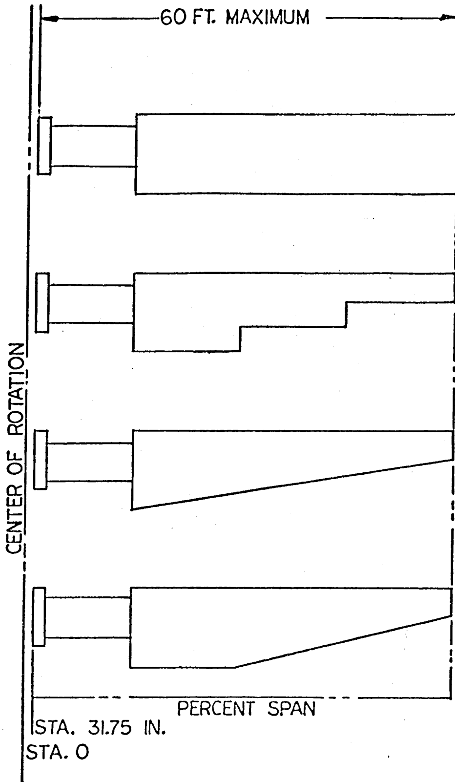
FIGURE 1 - ACCEPTABLE BLADE PLANFORMS
