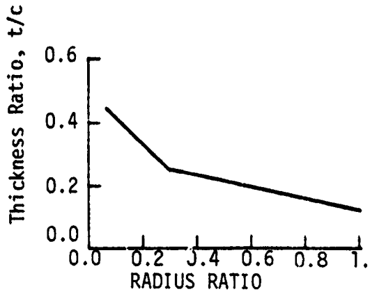
Figure 4. Thickness to Chord Ratio for Twisted Aluminum Blade
