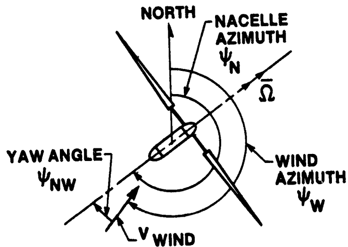
Figure 6. Mod-0 Wind Turbine Sign Convention
