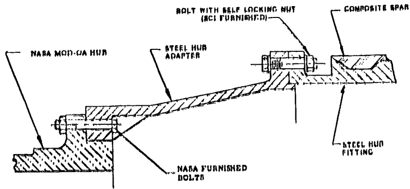
FIGURE 4 HUB ADAPTER DETAILS
