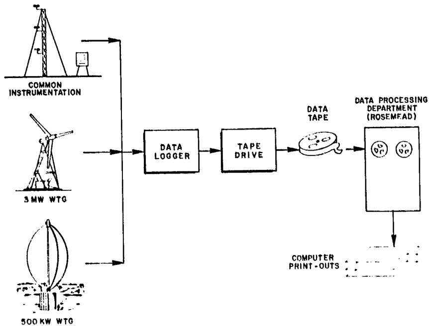
Figure 4: Edison Data Acquisition System
