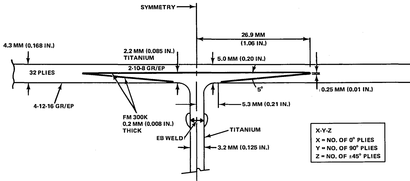
Figure 4 Concept C Detail, Scarf Joint
