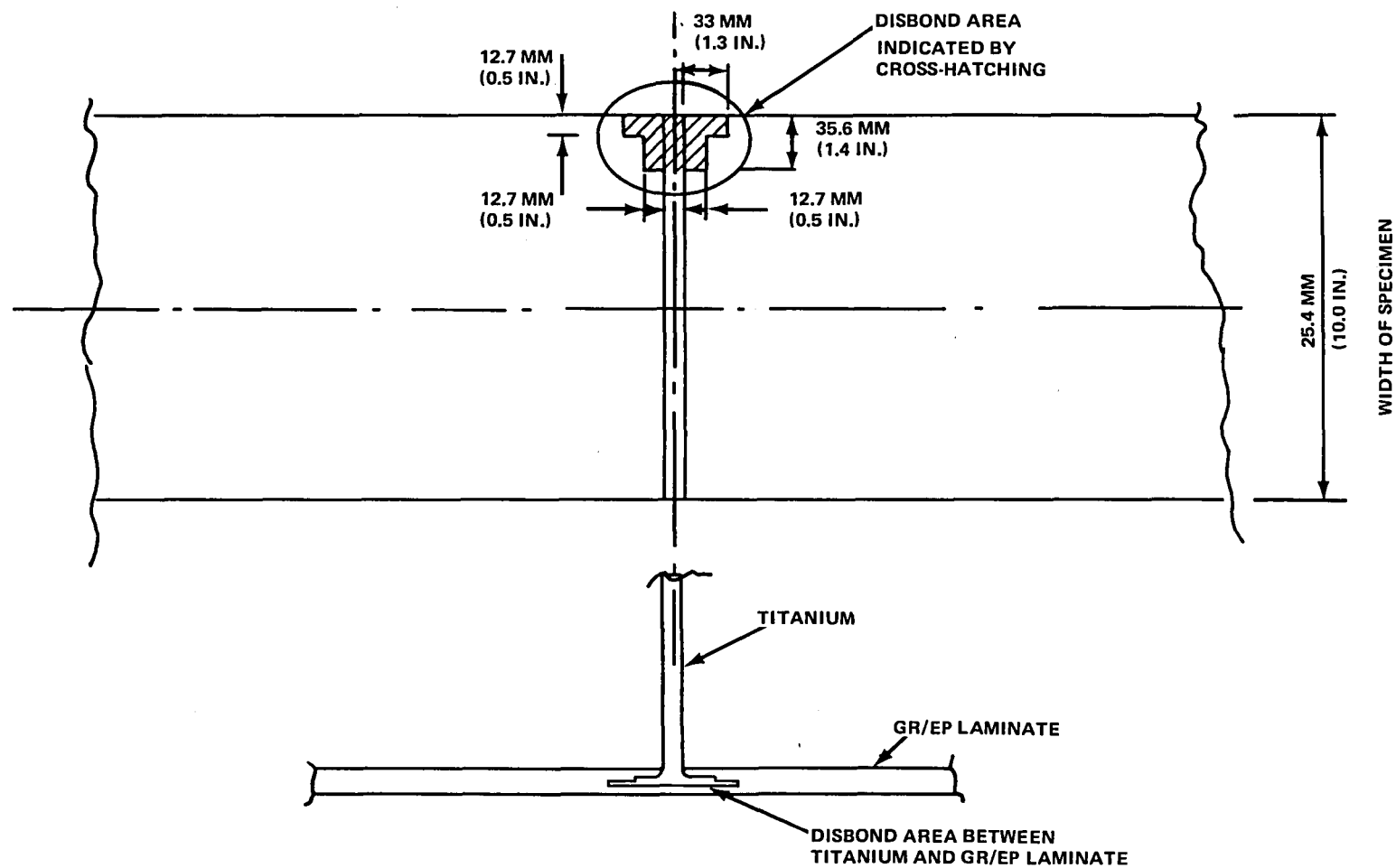
Figure 15 Ultrasonically Detected Void Area
