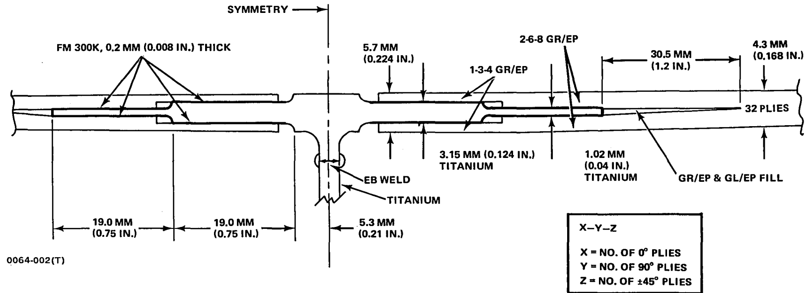
Figure 2 Concept A Detail, Two-Side Stepped Joint
