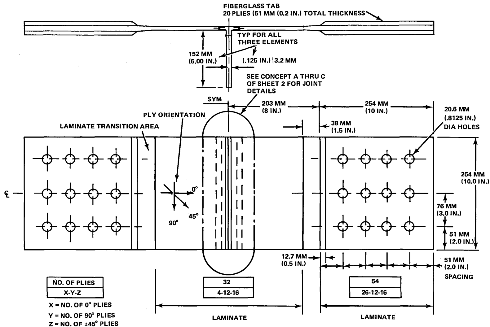
Figure 1 Specimen Configuration
