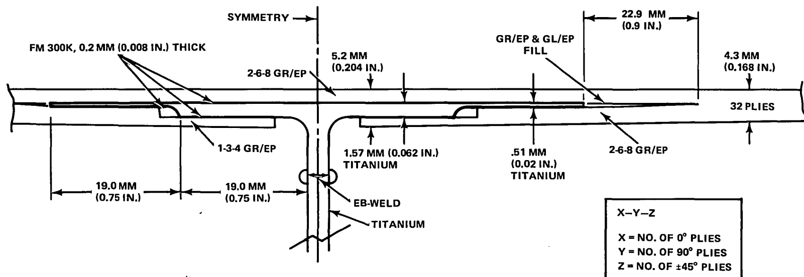
Figure 3 Concept B Detail, One-Side Stepped Joint
