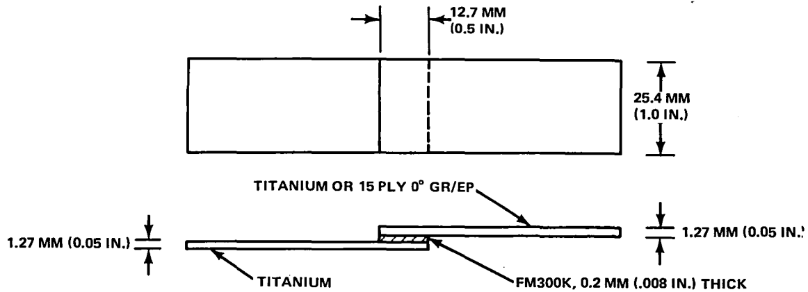
Figure 14 Verification Lap Shear Specimen
