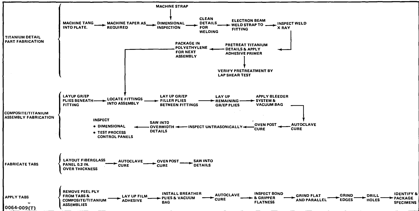
Figure 9 Manufacturing Flow
