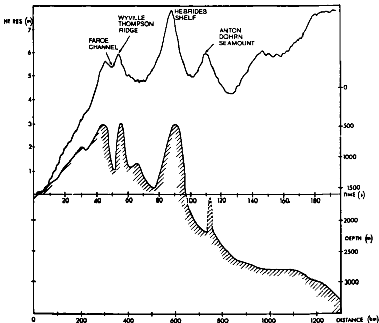
Figure 3 A Seasat pass over the eastern North Atlantic, showing the residual sea-level anomalies after removal of other signals. The surface shows a strong and geophysically useful correlation with bottom topography.
