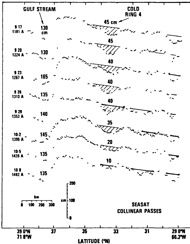
Figure 2 Seasat "frozen orbit" passes over the western North Atlantic. The Gulf Stream dynamic trough and ridge are clearly depicted, along with a cold ring that was identified positively by ship observations. Other structures are seen that may also be rings.
