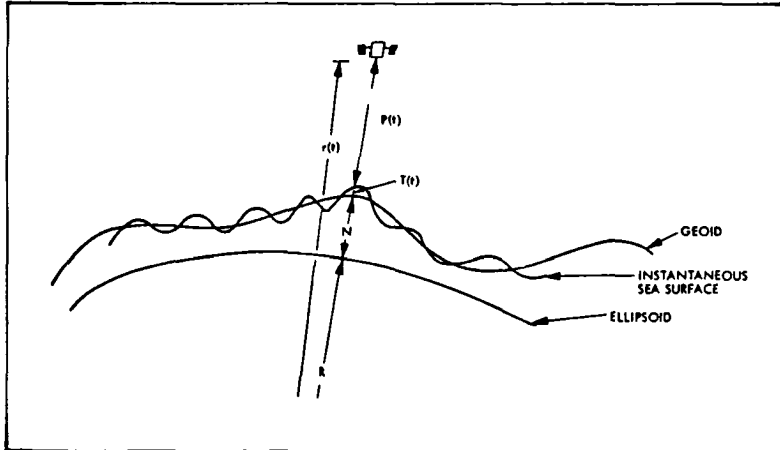
Figure 1 Schematic view of the geometry of the satellite altimeter vis-à-vis the reference ellipsoid (related to the geometric shape of the earth, the geoid (based on the actual distribution of the earth's gravity field), and the instantaneous sea surface
