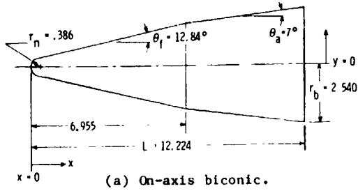
Fig. 1 Planform view and dimensions of models. All dimensions in cm.
