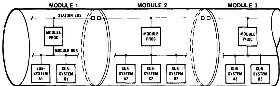
Figure 3-17. Distributed Processor Architecture
