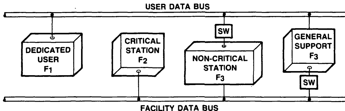
Figure 3-14. Dual Bus Structure
