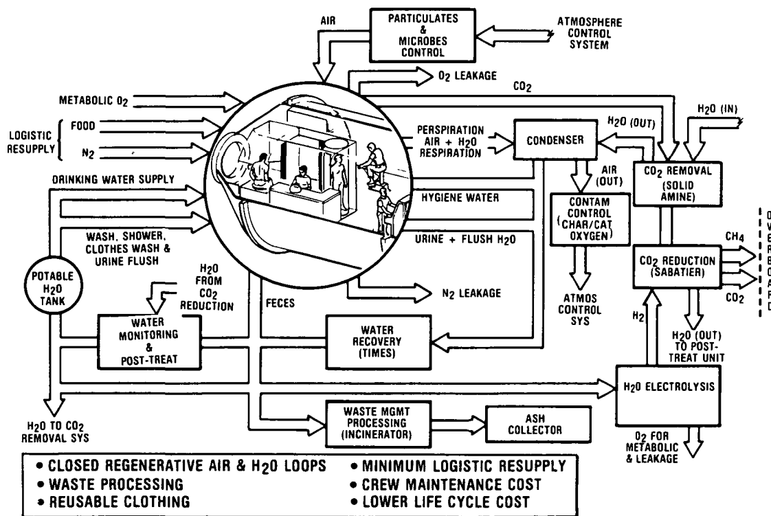
Figure 3-7. ECLSS Architecture
