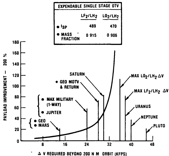
Figure 4-21. Fluorine Propellant Benefits
