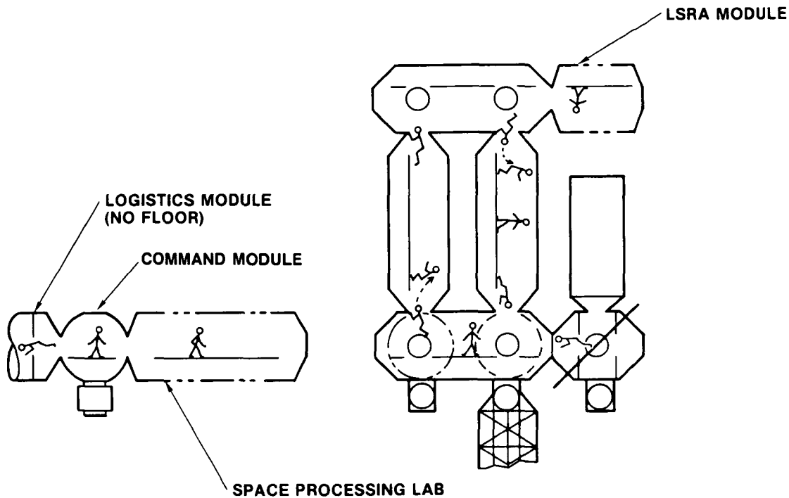
Figure 2-6. Growth Station Floor Arrangement
