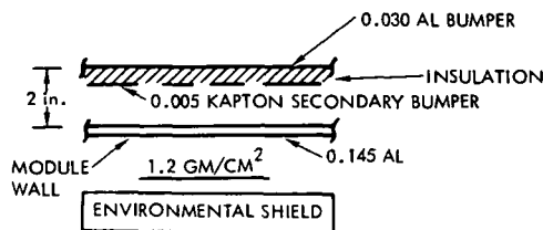
Figure 2-4. Standardized Module Concept
