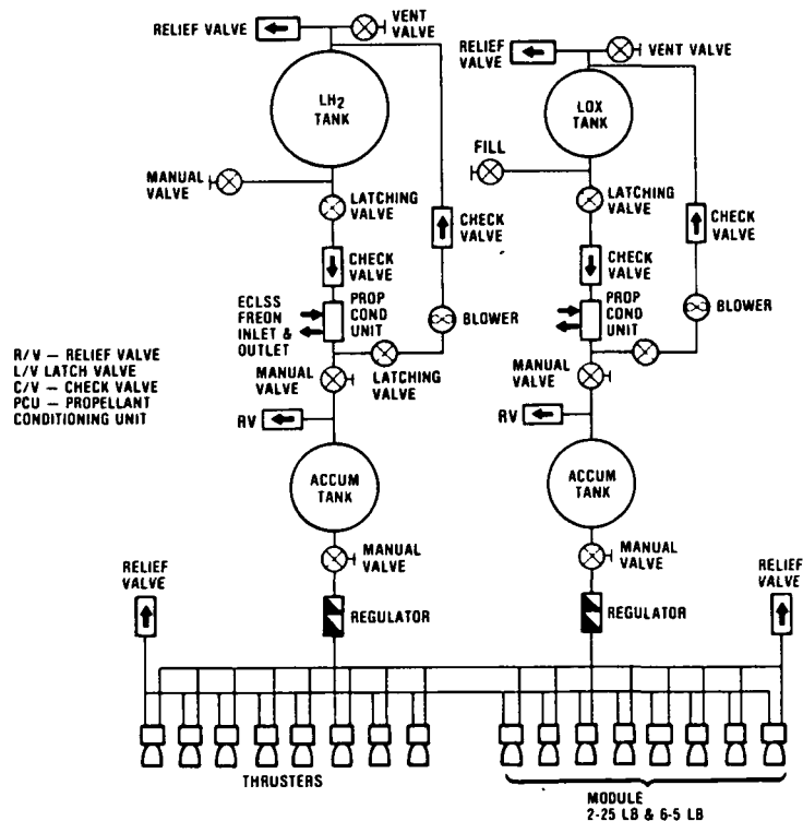
Figure 3-9. LO_2/LH RCS Schematic (Typical)
