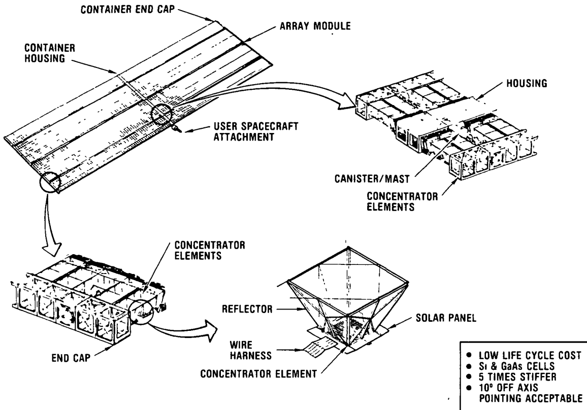
Figure 3-3. Low Concentration Solar Array Design
