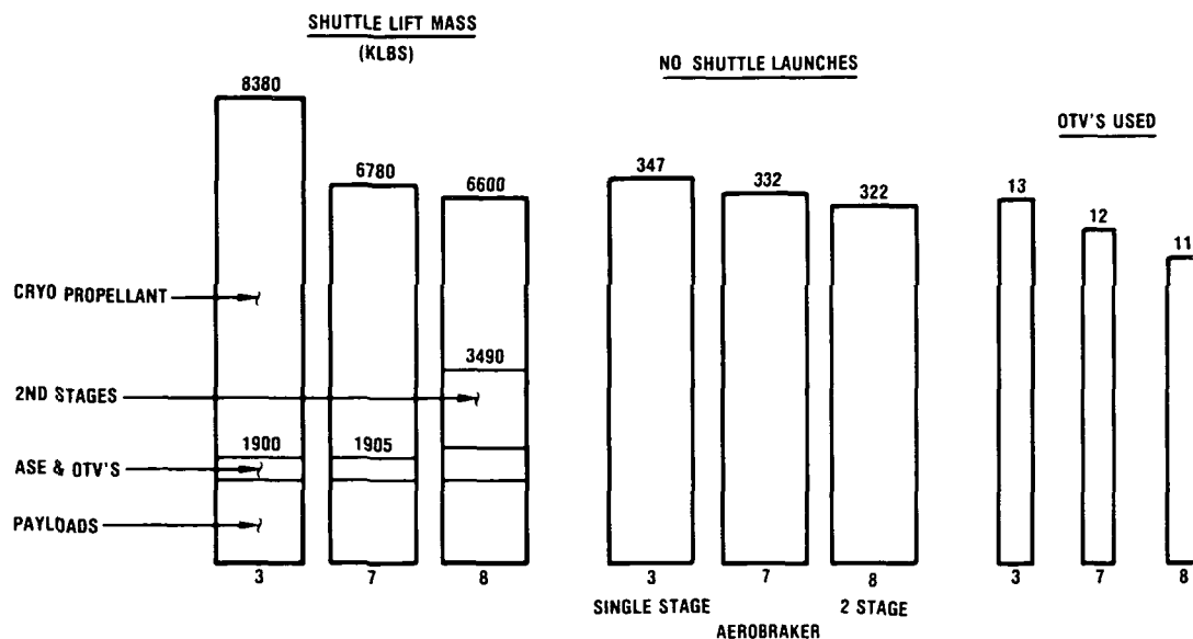
Figure 1-24. OTV Candidate Comparisons
