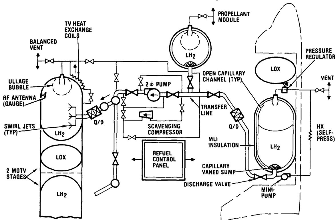
Figure 3-23. Cryo Propellant Handling and Storage Facility
