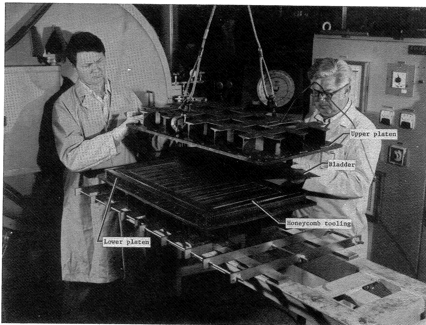
Figure 8.- Titanium-clad Borsic/aluminum panel assembly and tooling for brazing.
