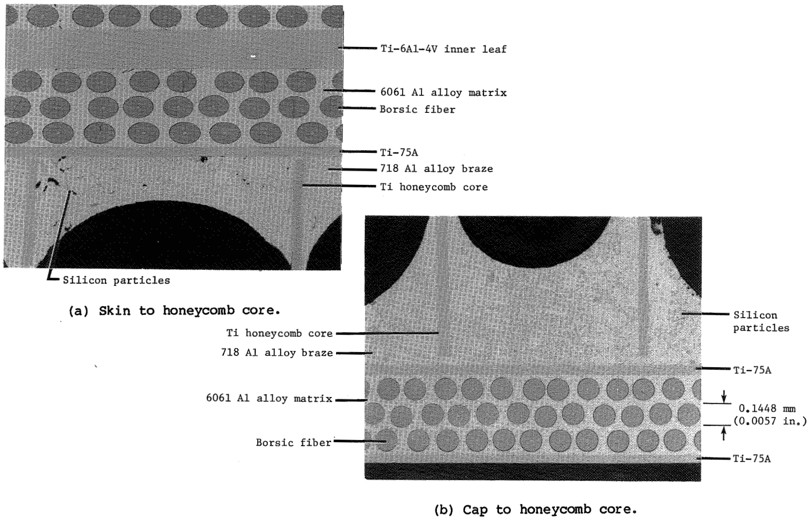
Figure 16.- Photomicrographs of typical skin-stringer braze joints.
