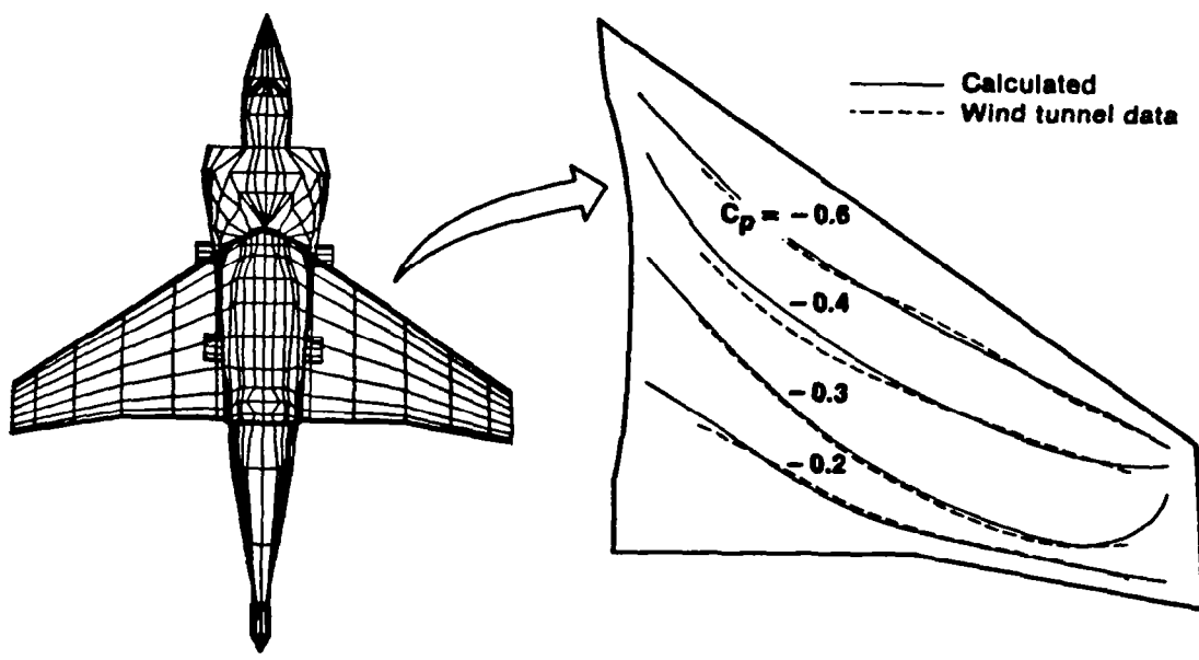
YAV-8B Surface Panel Modeling
