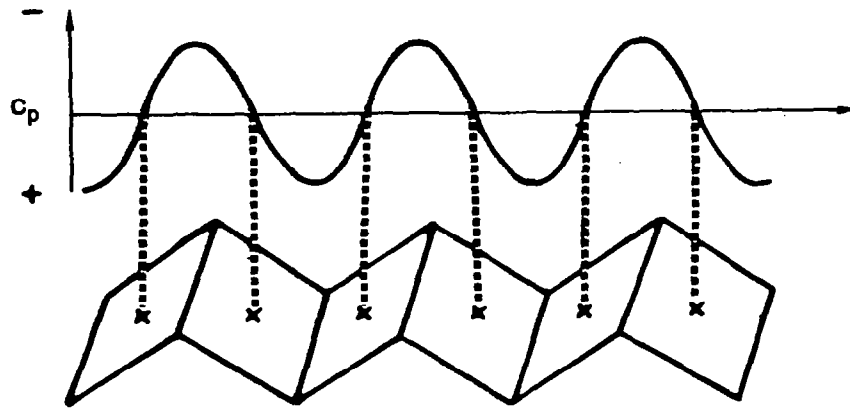
Pressure at Panel Center Does Not Control Streamwise Slope Oscillations
