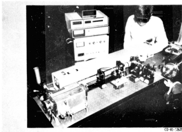
Fig. 8 Line-of-sight laser anemometer for measuring radial component of flow in an axial-flow machine.
