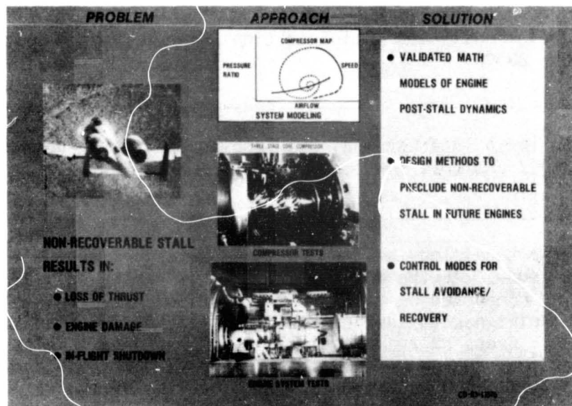
Fig. 18 Stall recovery research.
