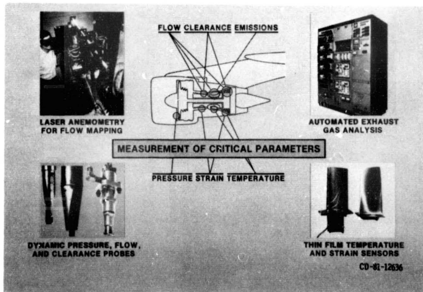
Fig. 7 Advanced instrumentation for propulsion research.
