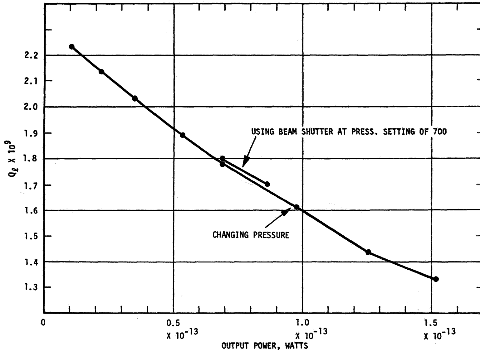
Figure 5. SAO-14 Line Q vs Output Power
