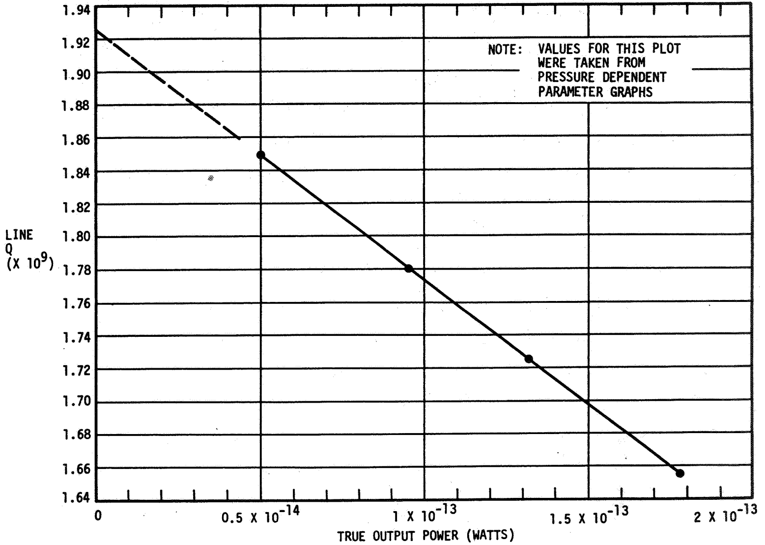
Figure 6. NR-4 Line Q vs Output Power
