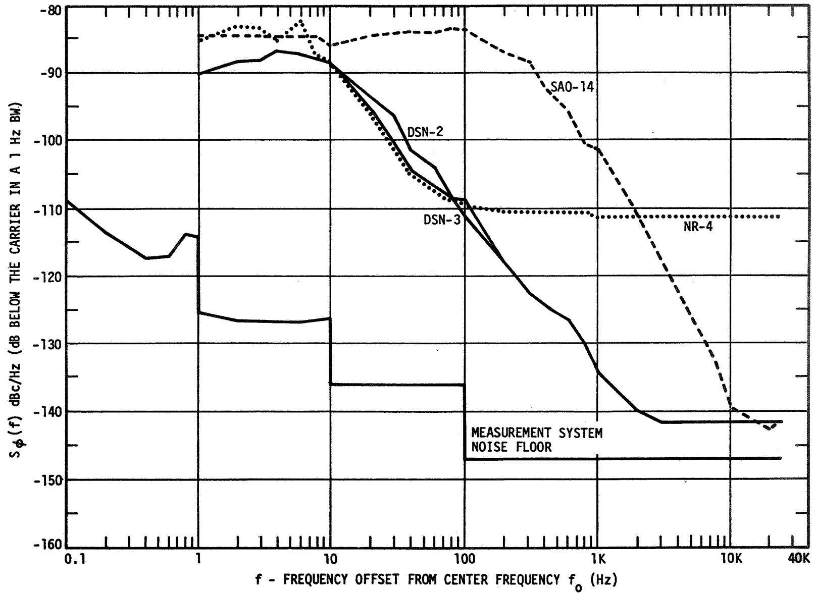
Figure 22. 100 MHz Phase Noise
