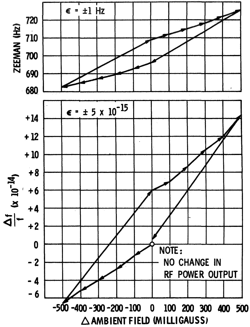
Figure 8. SAO-14 Magnetic Field Test - 1st Series
