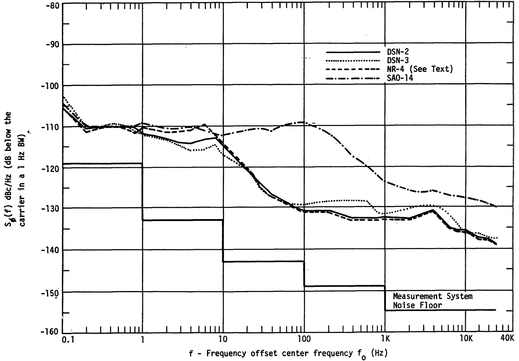
Figure 23. 5 MHz Phase Noise
