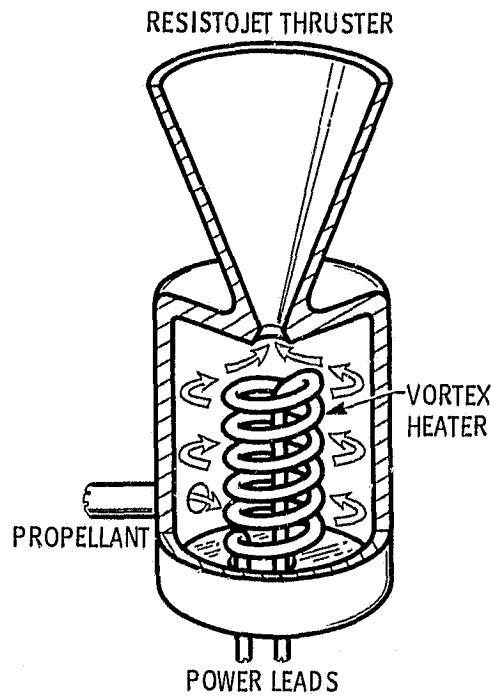
Figure 5. - Typical resistojet design concept.
