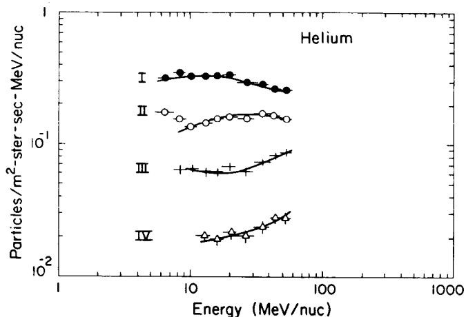
Fig. 7. Helium spectra measured during four time periods.
