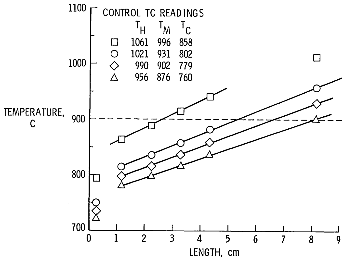
5. Typical temperature profiles in a boron nitride sample for different furnace settings.
