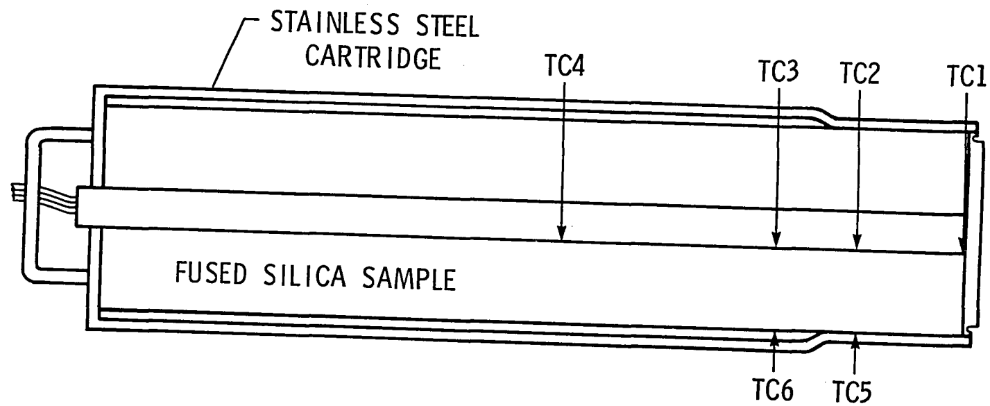
6. Schematic of the fused silica sample showing thermocouple placement.
