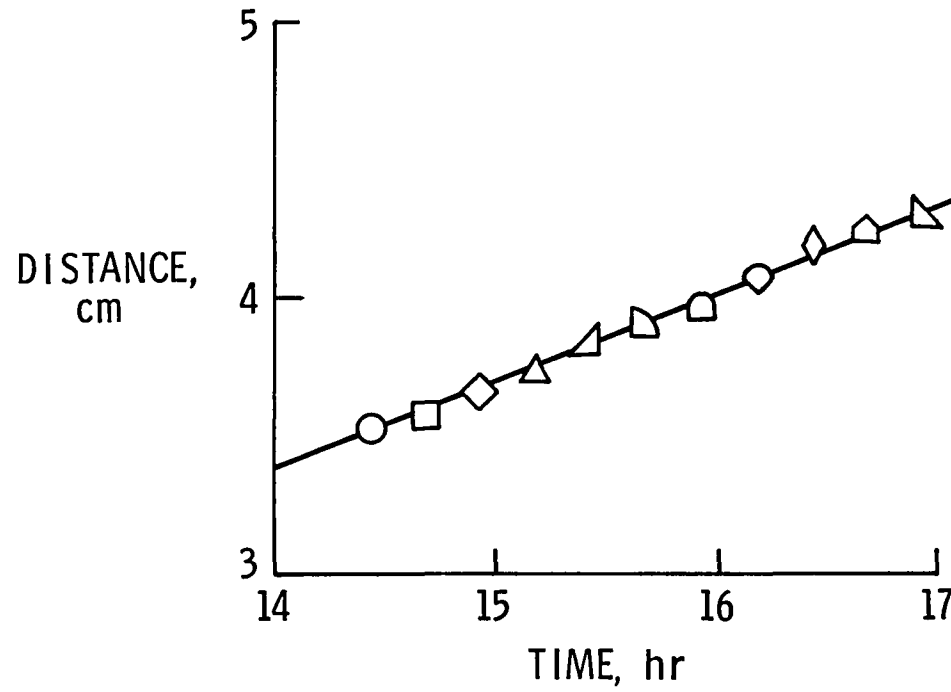
8. Interface position as a function of time showing the constant rate of change of the 900^{\circ}\text{C} temperature for this region of the furnace.
