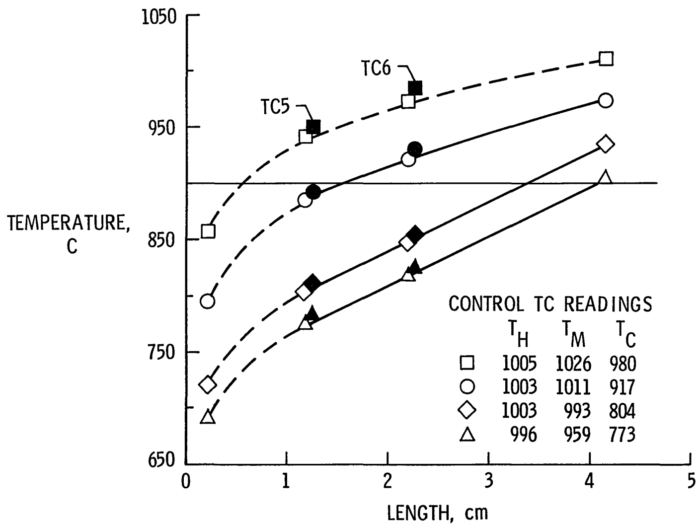
7. Typical temperature profiles in the fused silica sample for various furnace settings. The darkened symbols indicate the temperatures for thermocouples 5 and 6 which are along the outside of the sample rather than along the axis. Therefore, they give an indication of the small radial temperature gradients.
