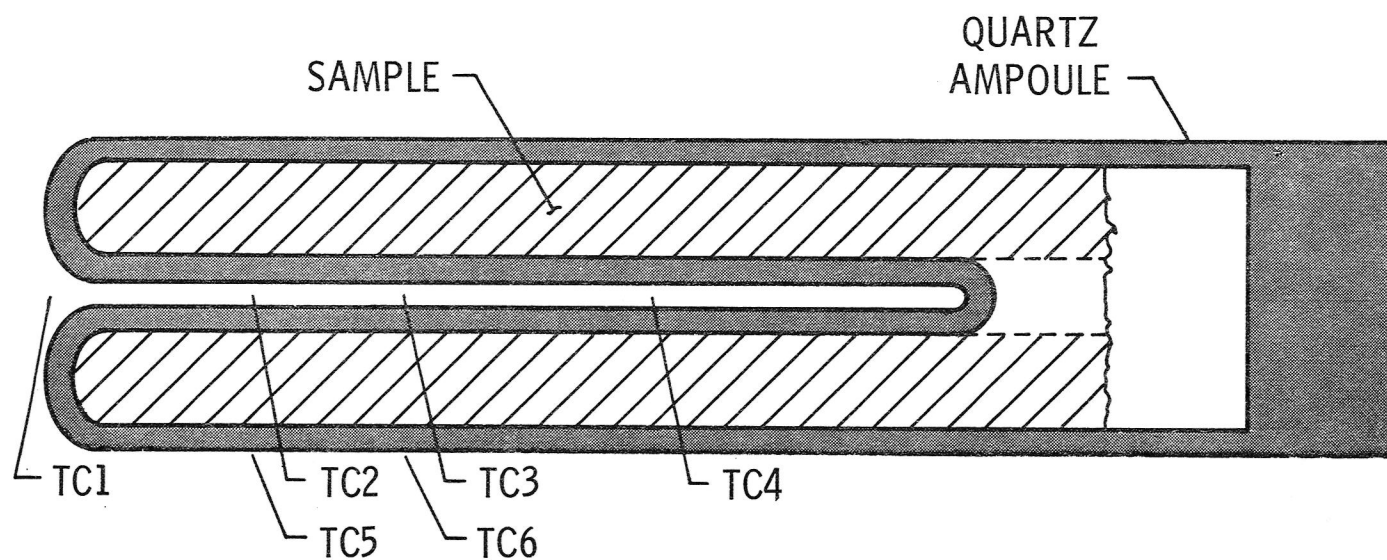
9. Schematic of a fused silica ampoule containing a lead-tin-telluride sample used for furnace evaluation. Thermocouple positions are indicated. The capillary is in the center of the sample.
