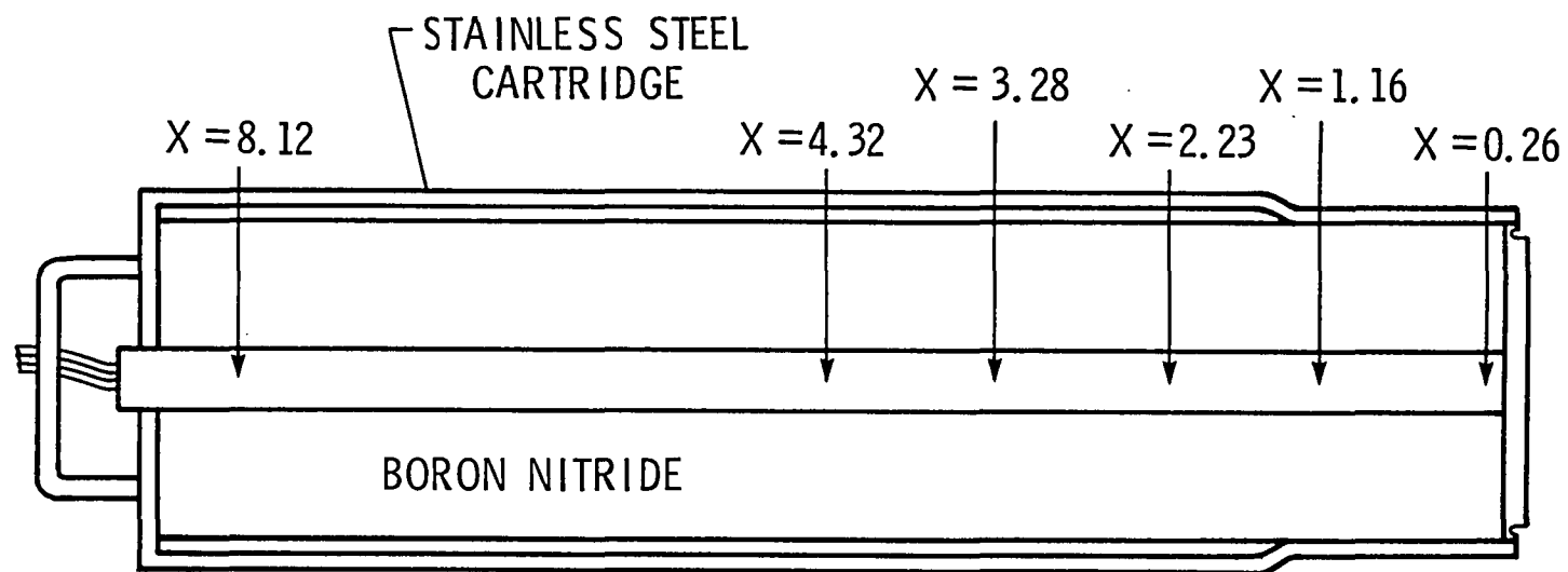
4. Cartridge for the boron nitride sample showing thermocouple placement. Dimensions are in cm.
