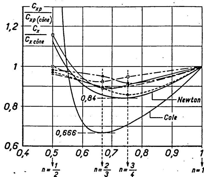
Fig. 11: \lambda = 2.13 Experiments of Kubota. \square M = 7.7 R_L/cm = 6.8, 10^4
