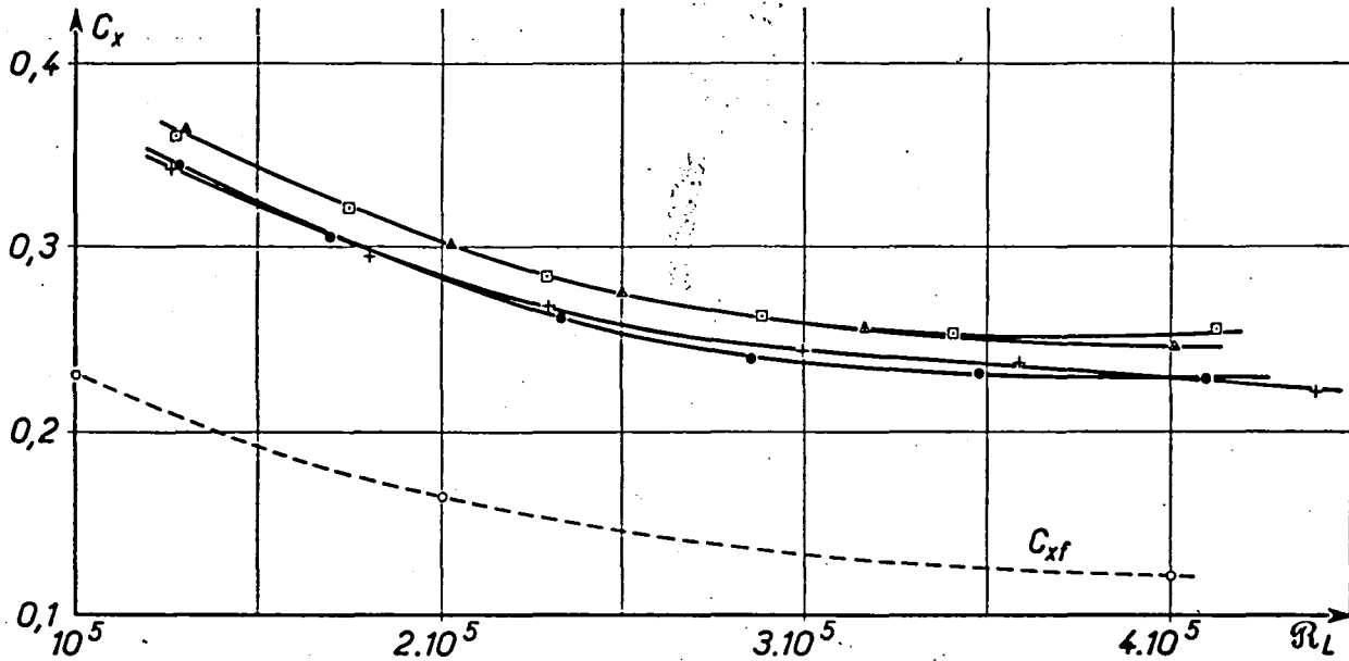
Fig. 7. — M \approx 3,75 p_t = 0,3 à 2 atm. \Delta n = 1 \square n = 1/2 \bullet n = 2/3 + n = 3/4 .
