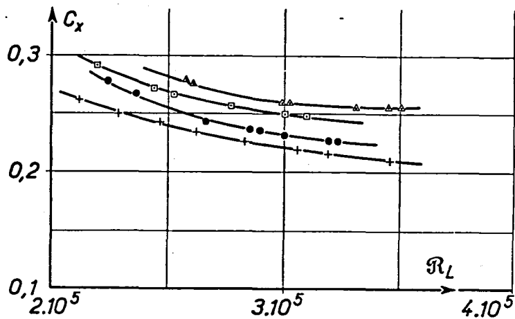
Fig. 9. — M = 5,3 \Delta n = 1 \square n = 1/2 \bullet n = 2/3 + n = 3/4 .
