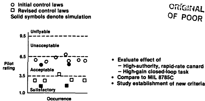
Fig. 15 Flying-qualities assessments.
