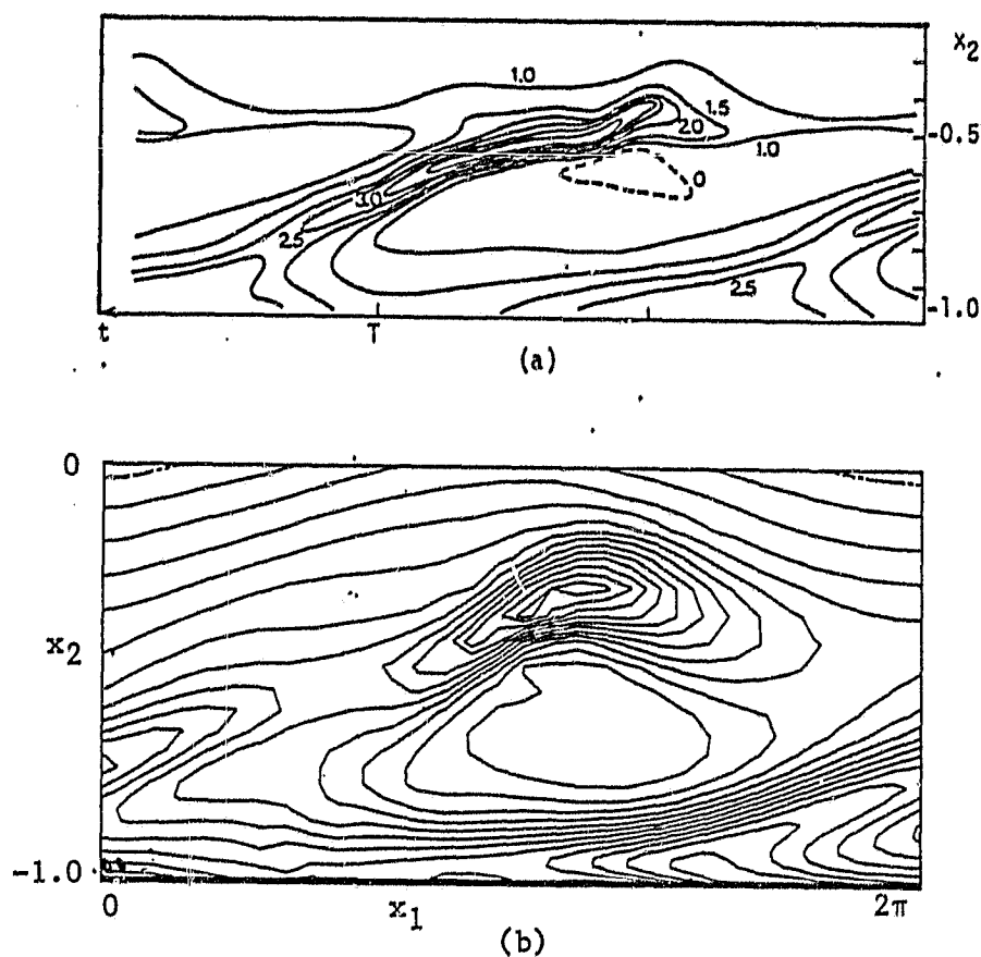
Figure 11. Contour plots of \partial u_1 / \partial x_2 . (a) One-spike stage, figure 4 from Nishioka et al. (1981); (b) computations at T = 17 in the x_1 - x_2 plane, contours from -0.2 to 2.6.
