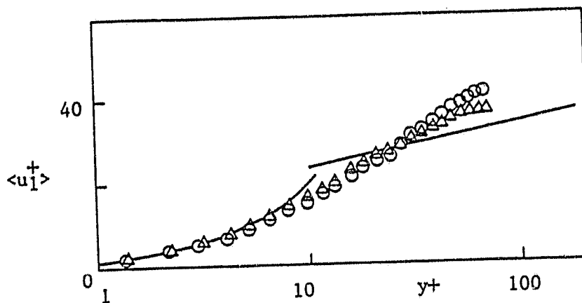
Figure 6. Plots of plane-averaged mean velocity in wall units. \circ , T = 0 ; \Delta , T = 79 .
