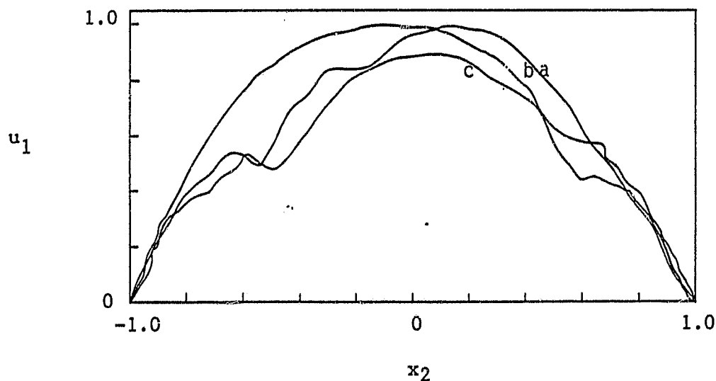
Figure 5. Plots of instantaneous velocity profiles at x_1 = 3\pi/2 , x_3 = \pi/2 . (a) T=17 ; (b) T=44 ; (c) T=79 .
