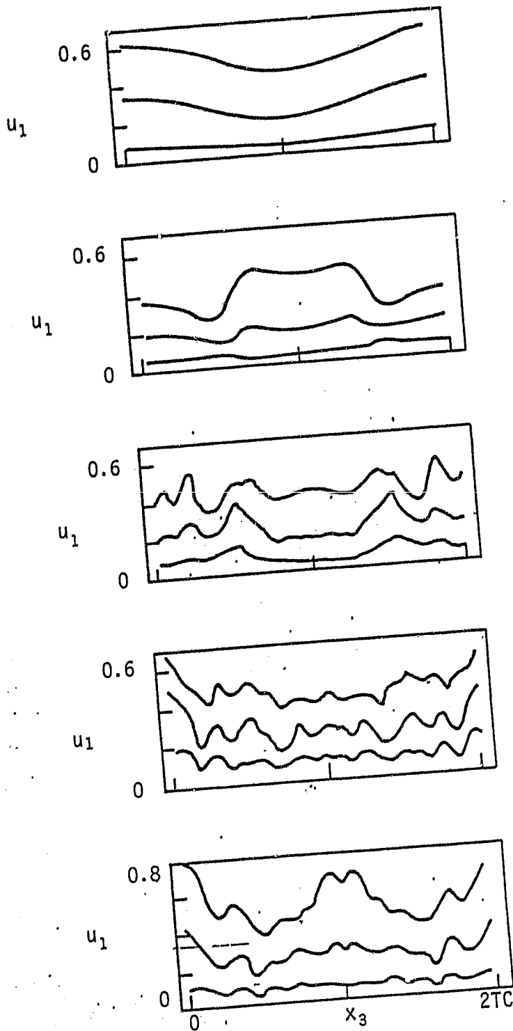
Figure 9. Spanwise variations of u_1 . (a) T = 0 ; (b) T = 17 ; (c) T = 27 ; (d) T = 44 ; (e) T = 79 . (i) bottom, x_2 = -0.968 ; (ii) middle, x_2 = -0.903 ; (iii) top, x_2 = -0.764 .
