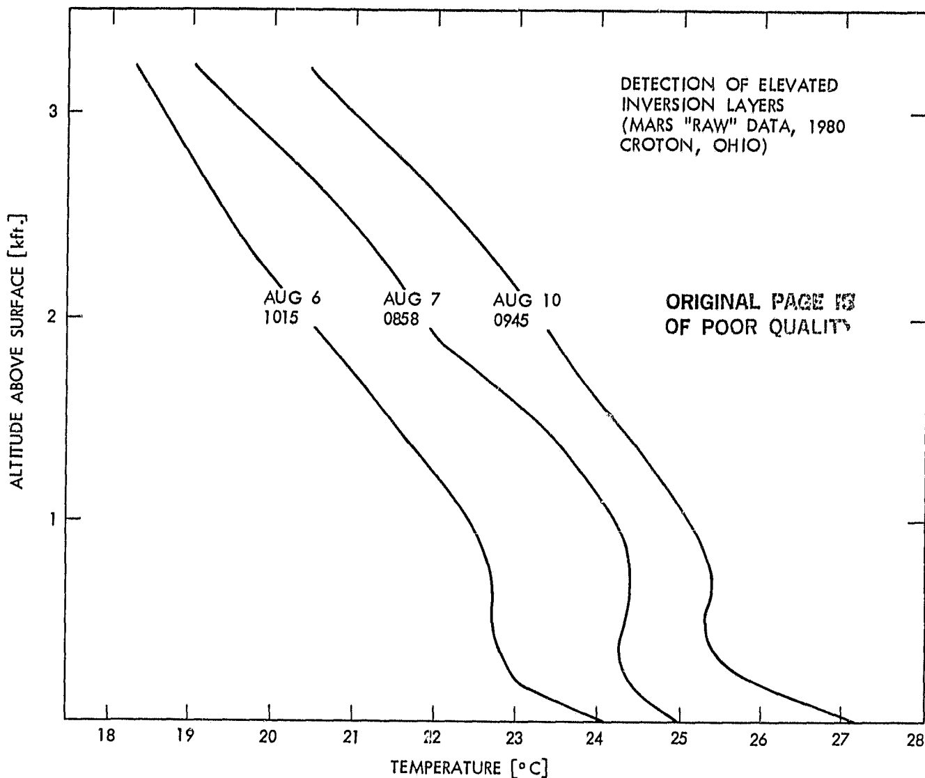
Figure B-6. Samples of Three MARS Profiles During Morning Periods When Elevated Inversion Layers Were Present. The early-morning ground-based inversions were converting to late-morning adiabatic lapse rate profiles. From such "raw data" plots it is apparent that inversion structures were present, and the altitudes of the bases and tops can easily be estimated. Note the small temperature contrast.
