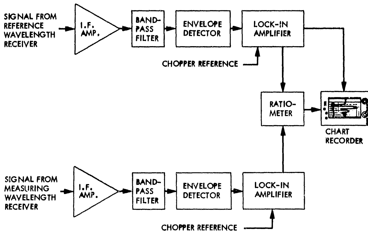
Figure 2-3. Block Diagram of the LAS Electronics and Signal Processing Systems
