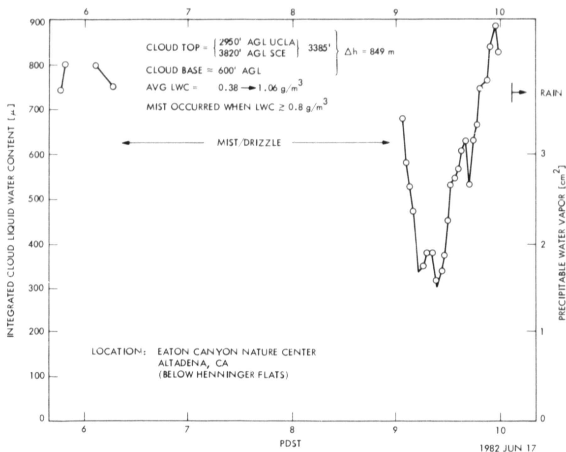
Figure A-2. Plot of Cloud Liquid Water Content Versus Time, During Acid Fog Coordinated Measurements with Caltech Investigators. Liquid content varies from 300 to 900 microns during this 4-hour period, during which there is no apparent "burn-off."
