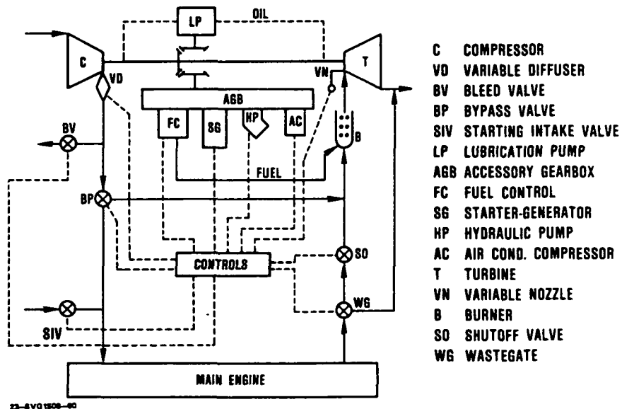
Figure 21. Schematic of the Turbocharger APU Mode.
