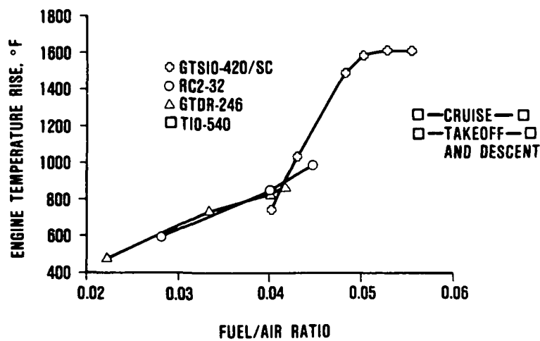
Figure 3. Engine Temperature Rise Characterization.
