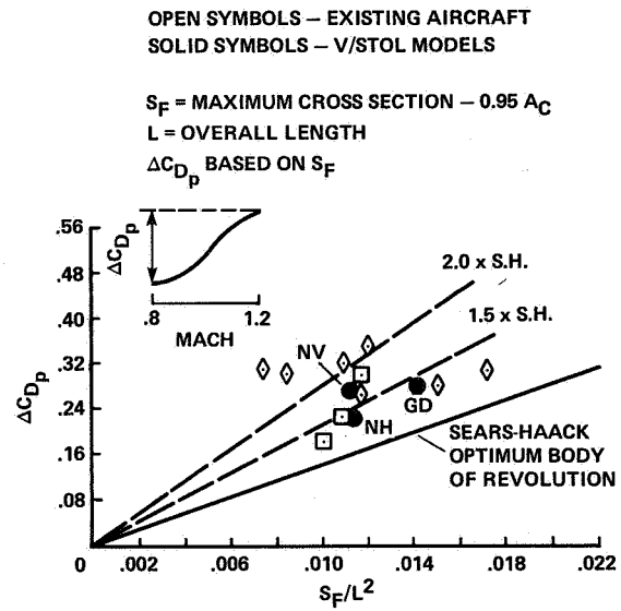
Figure 26. Wave drag comparison.
