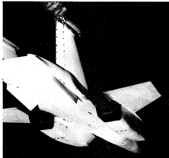
Figure 34. ADEN nozzles on the 623 model.
