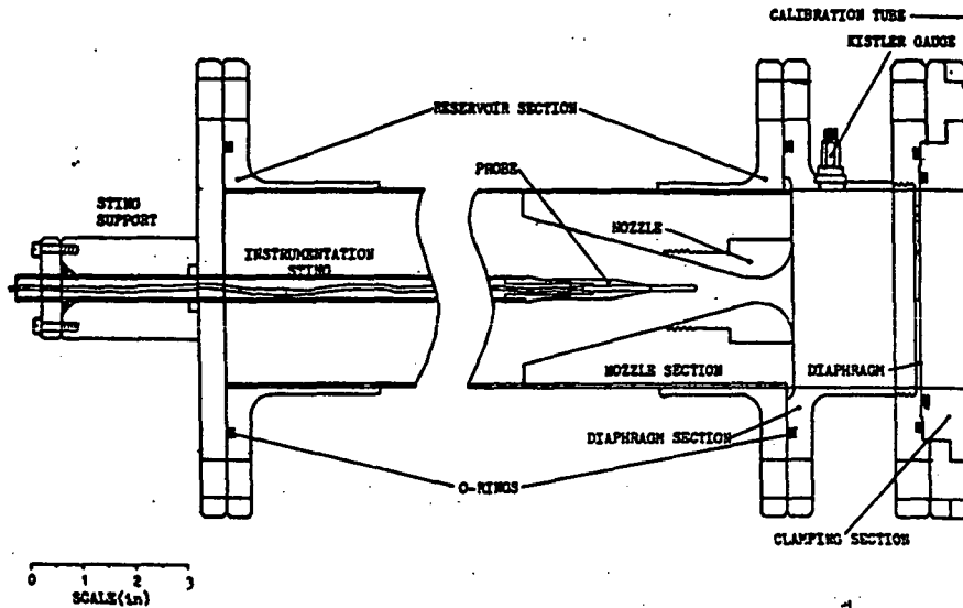
Figure 22 Test Section With Conical Nozzle
