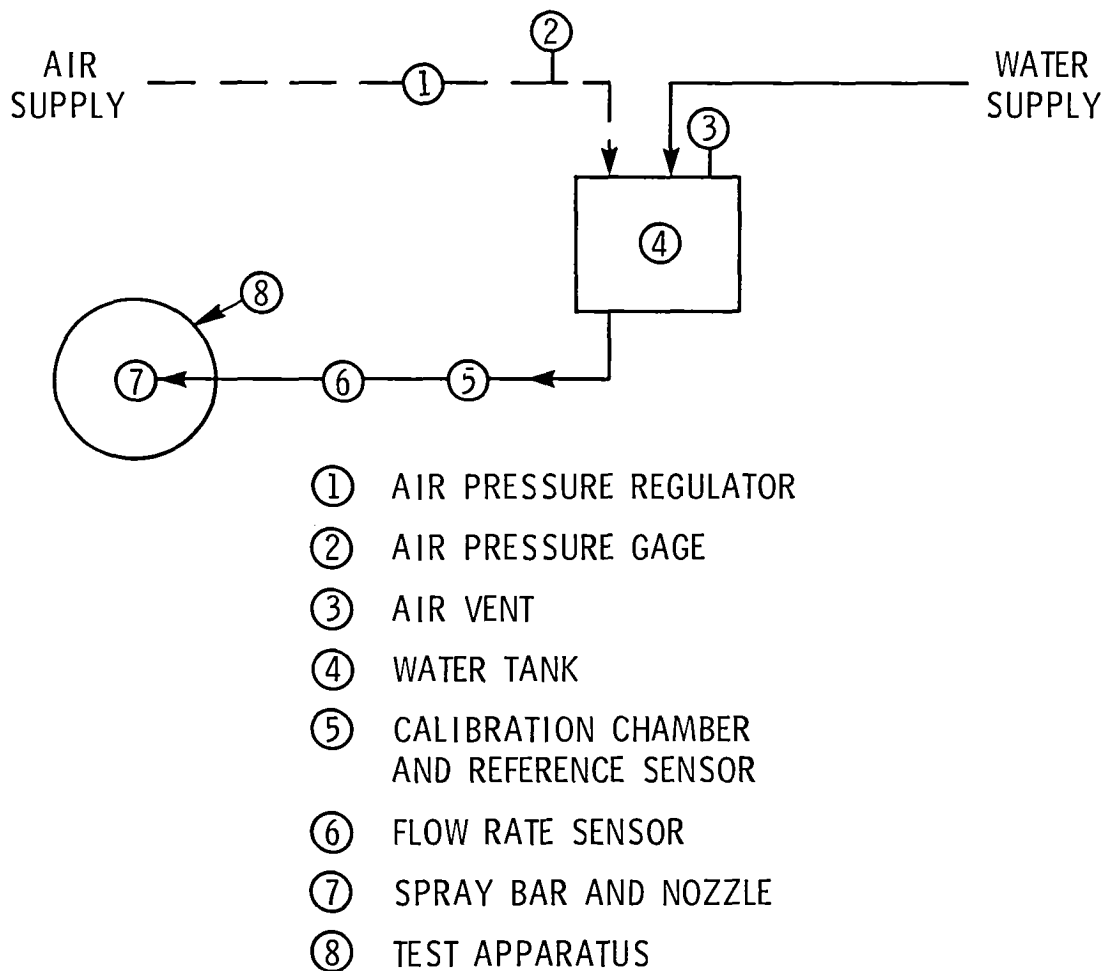
Figure 2.- Diagram of the water feed system.
