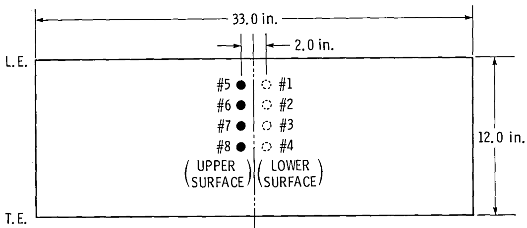
PLAN VIEW OF WING
