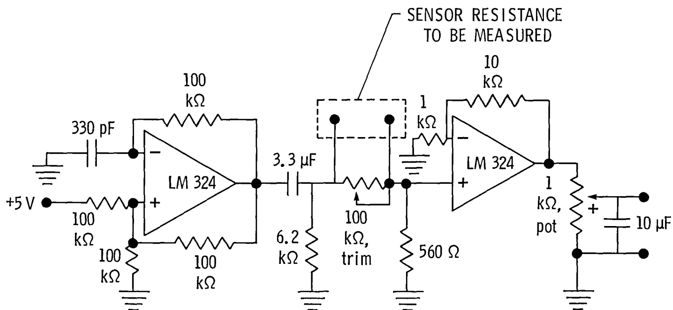
Figure 5.- Resistance-measuring circuit.
